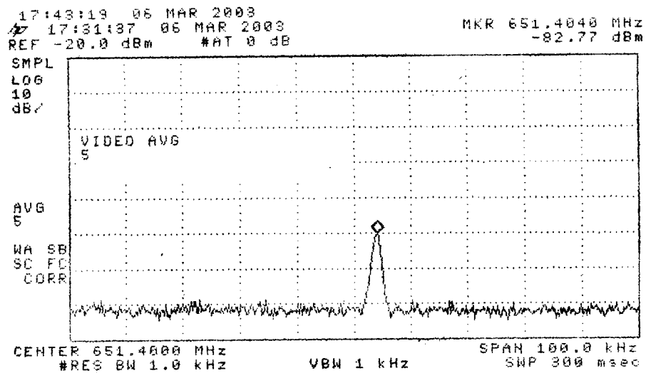
Figure 6.1. Receiver emission at 651.4 MHz.
