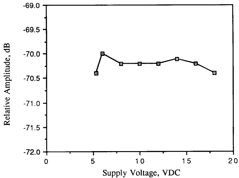
Figure 6.2. Relative emission at 651.4 MHz vs. supply voltage.
