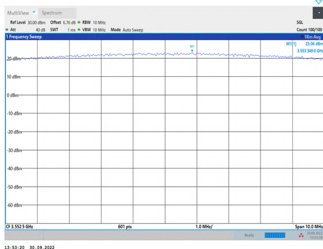
Band48-5MHz-QPSK-55265-1RB#12
