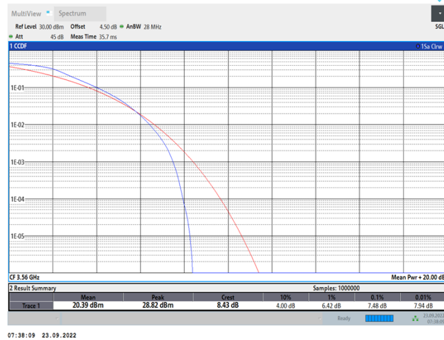
Band48-20MHz-QPSK-55990-100RB#0
