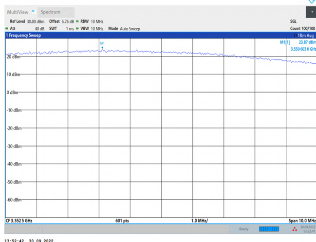
Band48-5MHz-QPSK-55265-1RB#12
