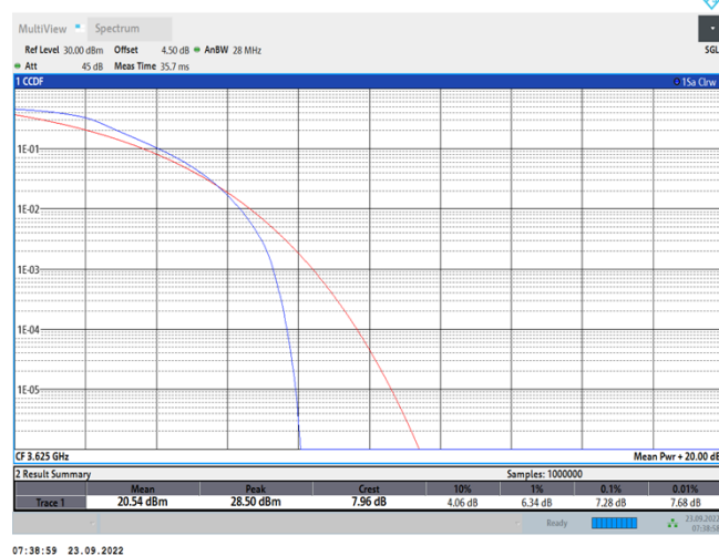
Band48-20MHz-QPSK-55990-100RB#0
