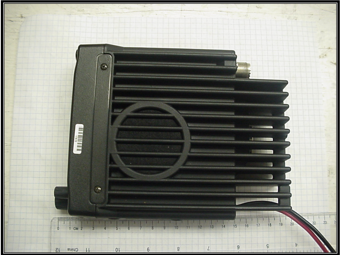
Photograph 8: Top of EUT
