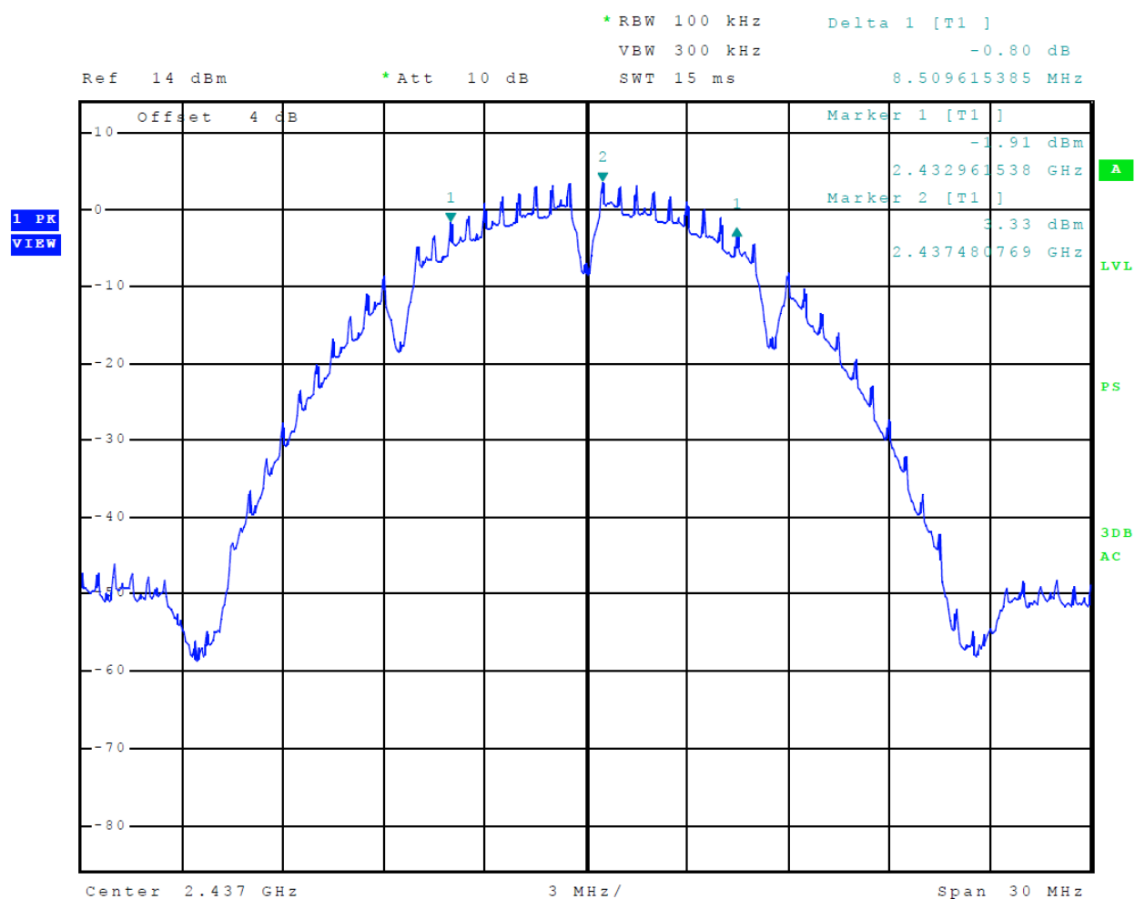
Figure 27 Plot of Transmitter 6-dB Occupied Band Width (802.11b) Chain 0
