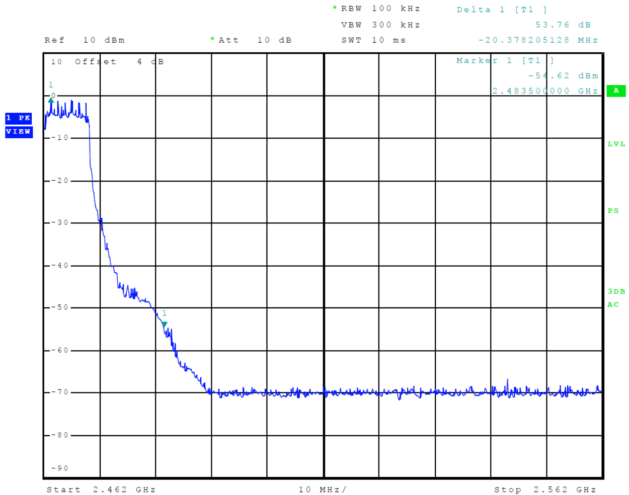
Figure 22 Plot of Transmitter High Band Edge (802.11g) Chain 1
