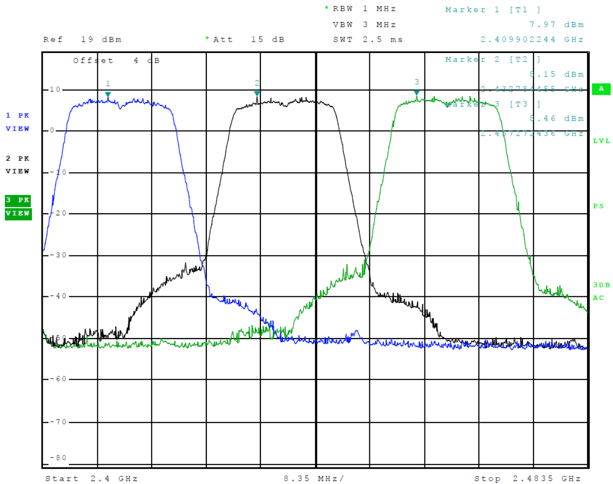
Figure 7 Plot of Transmitter Emissions (Across Operational Band, 802.11n) Chain 0
