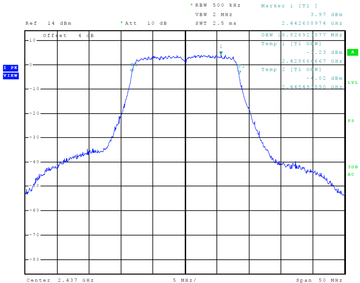
Figure 37 Plot of Transmitter 99% Occupied Band Width (802.11g) Chain 0
