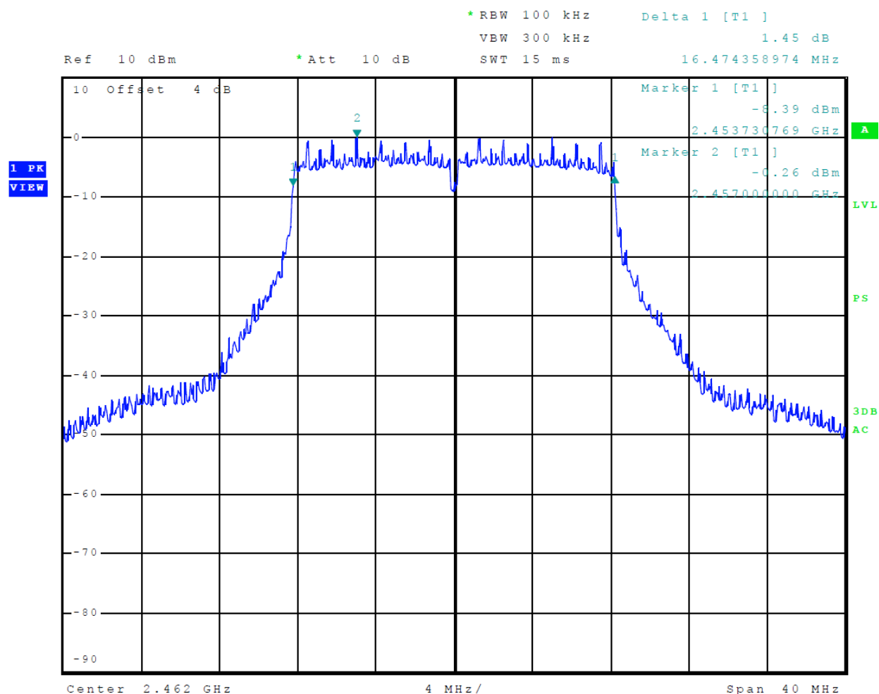
Figure 32 Plot of Transmitter 6-dB Occupied Band Width (802.11n) Chain 1
