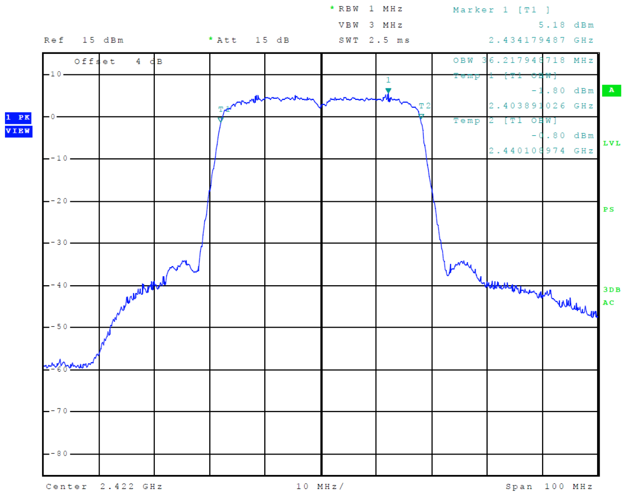
Figure 42 Plot of Transmitter 99% Occupied Band Width (802.11n40) Chain 1
