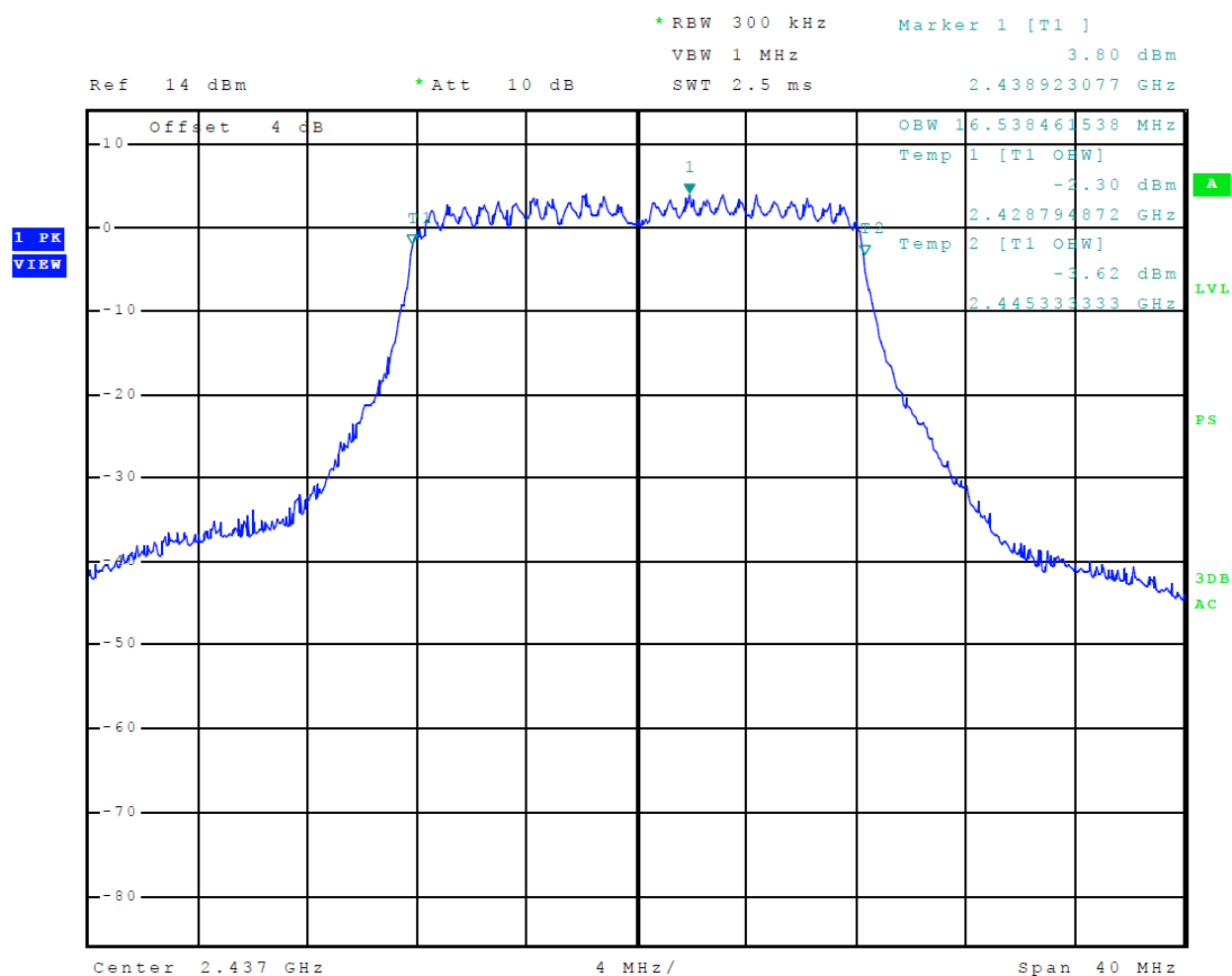
Figure 38 Plot of Transmitter 99% Occupied Band Width (802.11g) Chain 1
