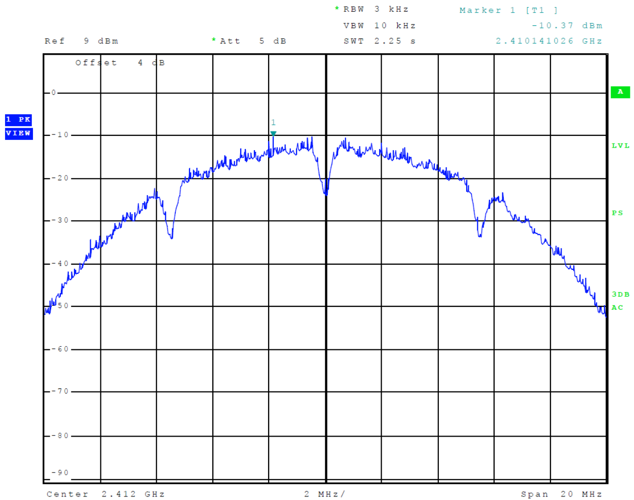
Figure 43 Plot of Transmitter Power Spectral Density (802.11b) Chain 0
