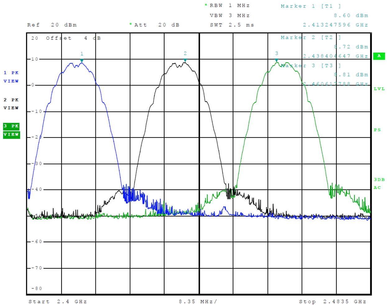
Figure 3 Plot of Transmitter Emissions (Across Operational Band 802.11b) Chain 0
