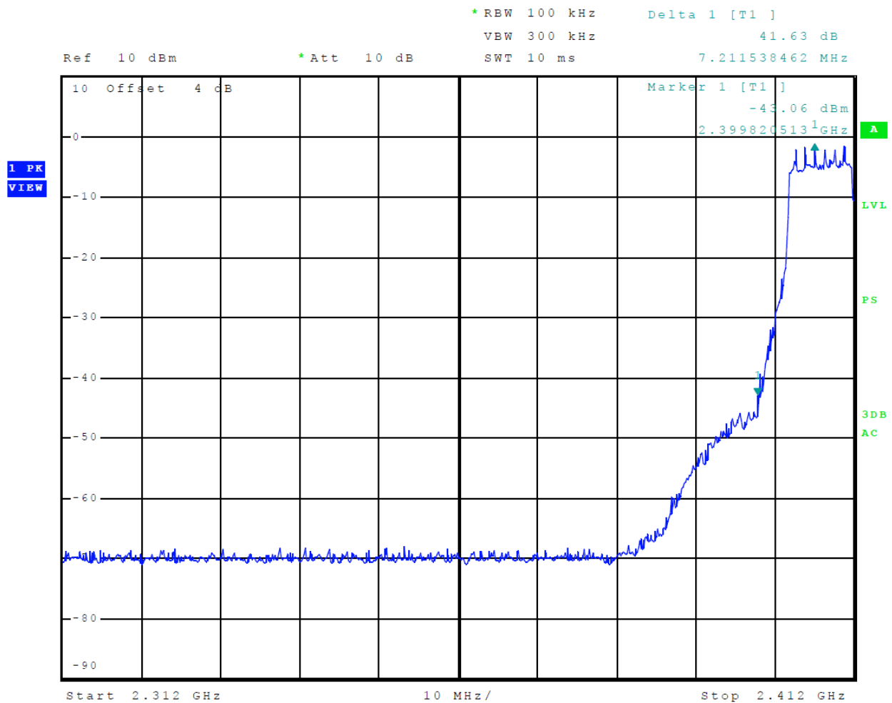
Figure 13 Plot of Transmitter Low Band Edge (802.11g) Chain 0
