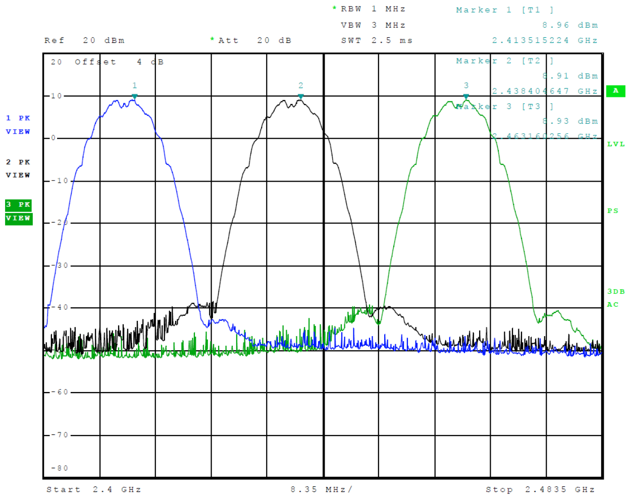
Figure 4 Plot of Transmitter Emissions (Across Operational Band 802.11b) Chain 1
