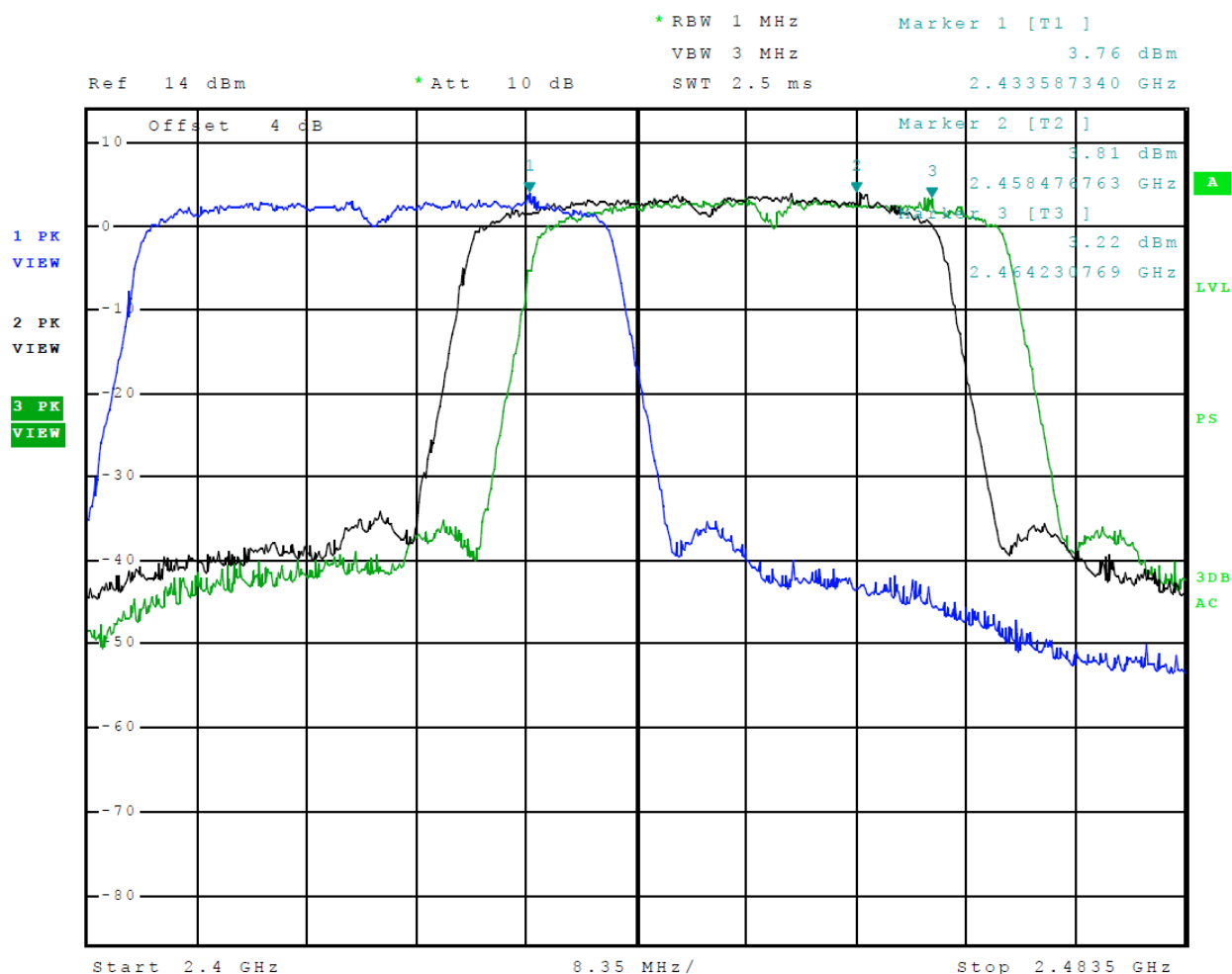
Figure 9 Plot of Transmitter Emissions (Across Operational Band, 802.11n40) Chain 0
