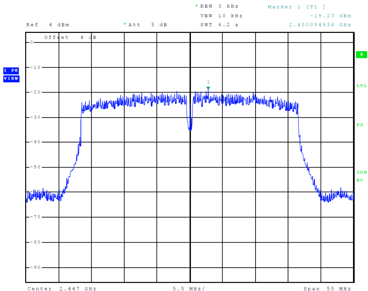
Figure 49 Plot of Transmitter Power Spectral Density (802.11n40) Chain 0
