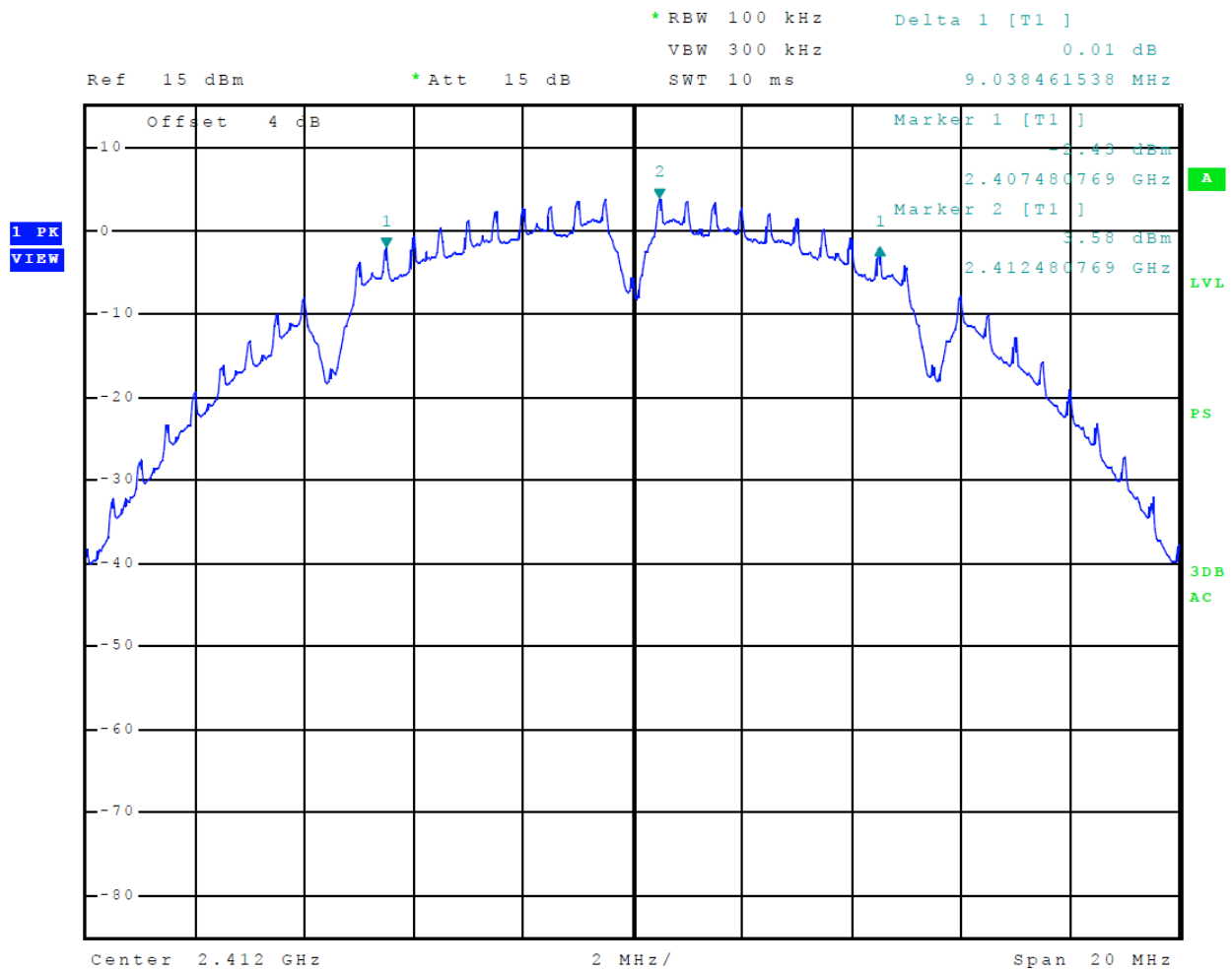
Figure 28 Plot of Transmitter 6-dB Occupied Band Width (802.11b) Chain 1
