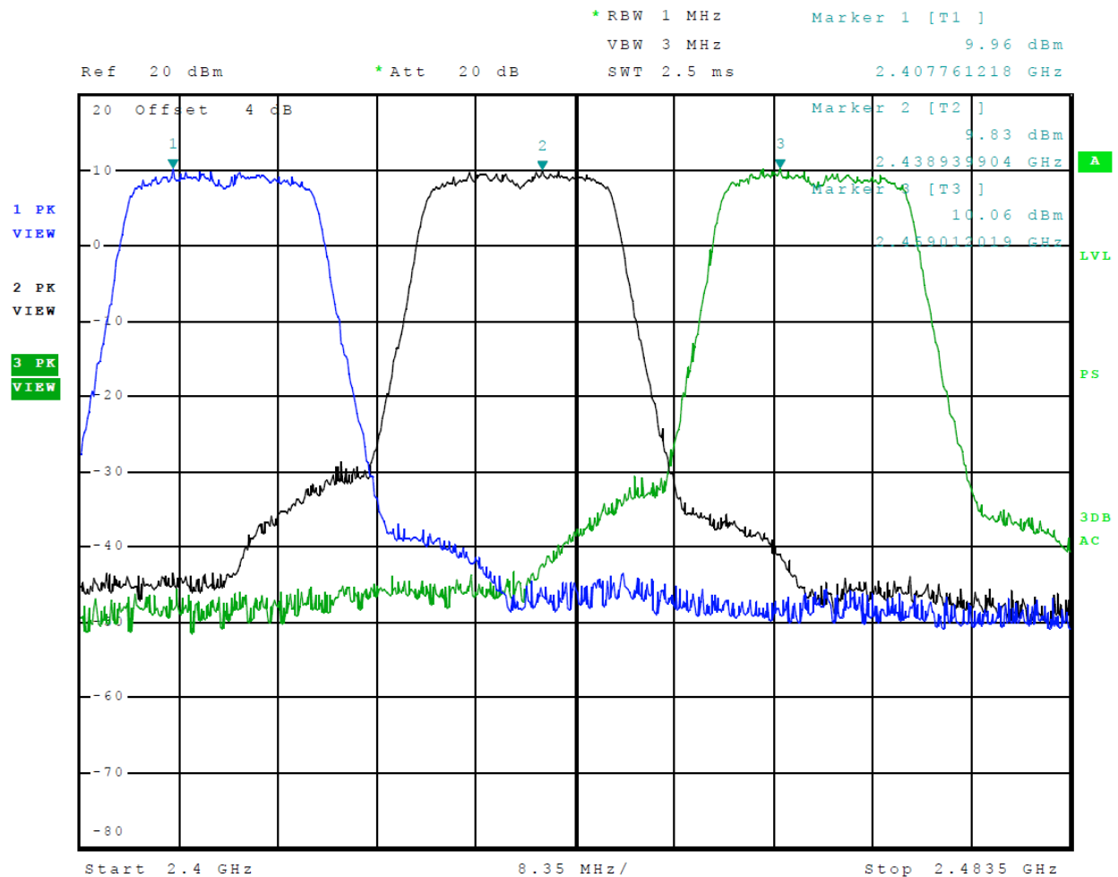
Figure 8 Plot of Transmitter Emissions (Across Operational Band, 802.11n) Chain 1
