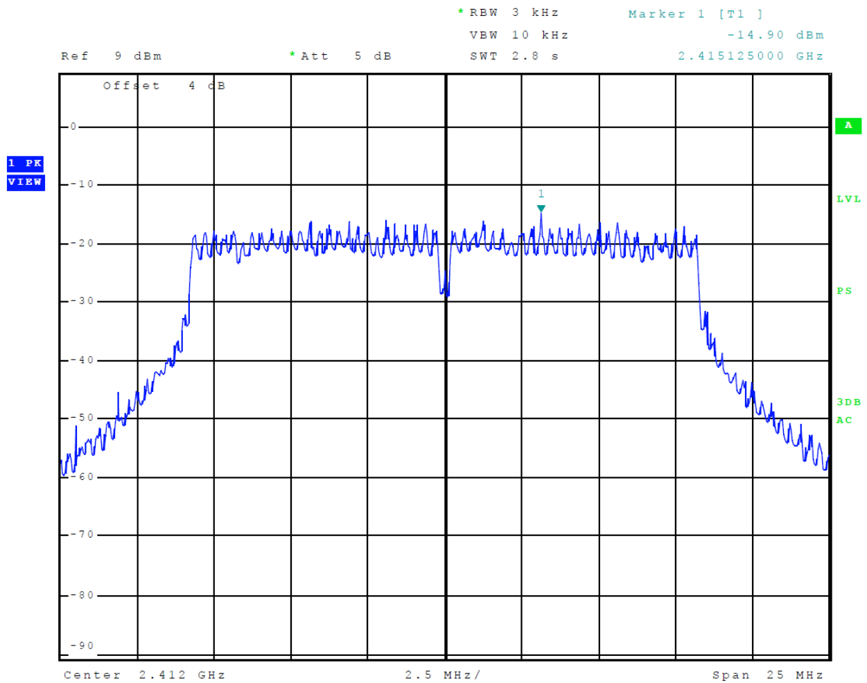
Figure 47 Plot of Transmitter Power Spectral Density (802.11n) Chain 0
