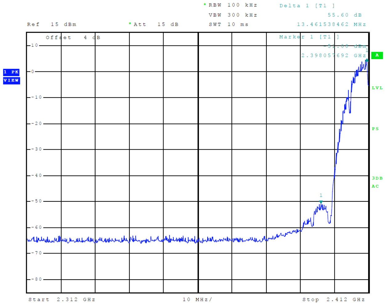
Figure 12 Plot of Transmitter Low Band Edge (802.11b) Chain 1
