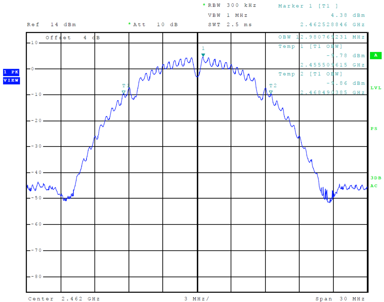
Figure 35 Plot of Transmitter 99% Occupied Band Width (802.11b) Chain 0
