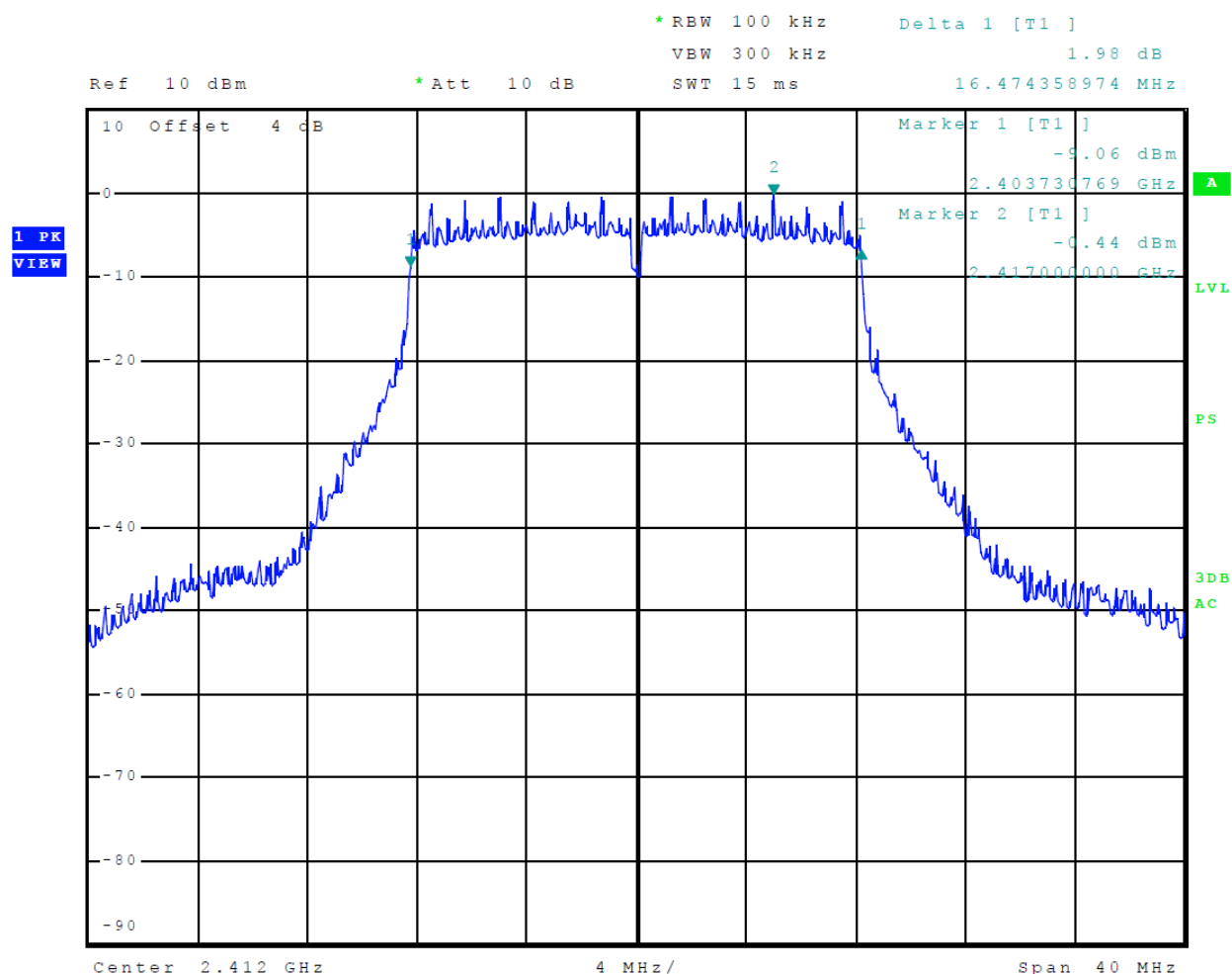
Figure 30 Plot of Transmitter 6-dB Occupied Band Width (802.11g) Chain 1
