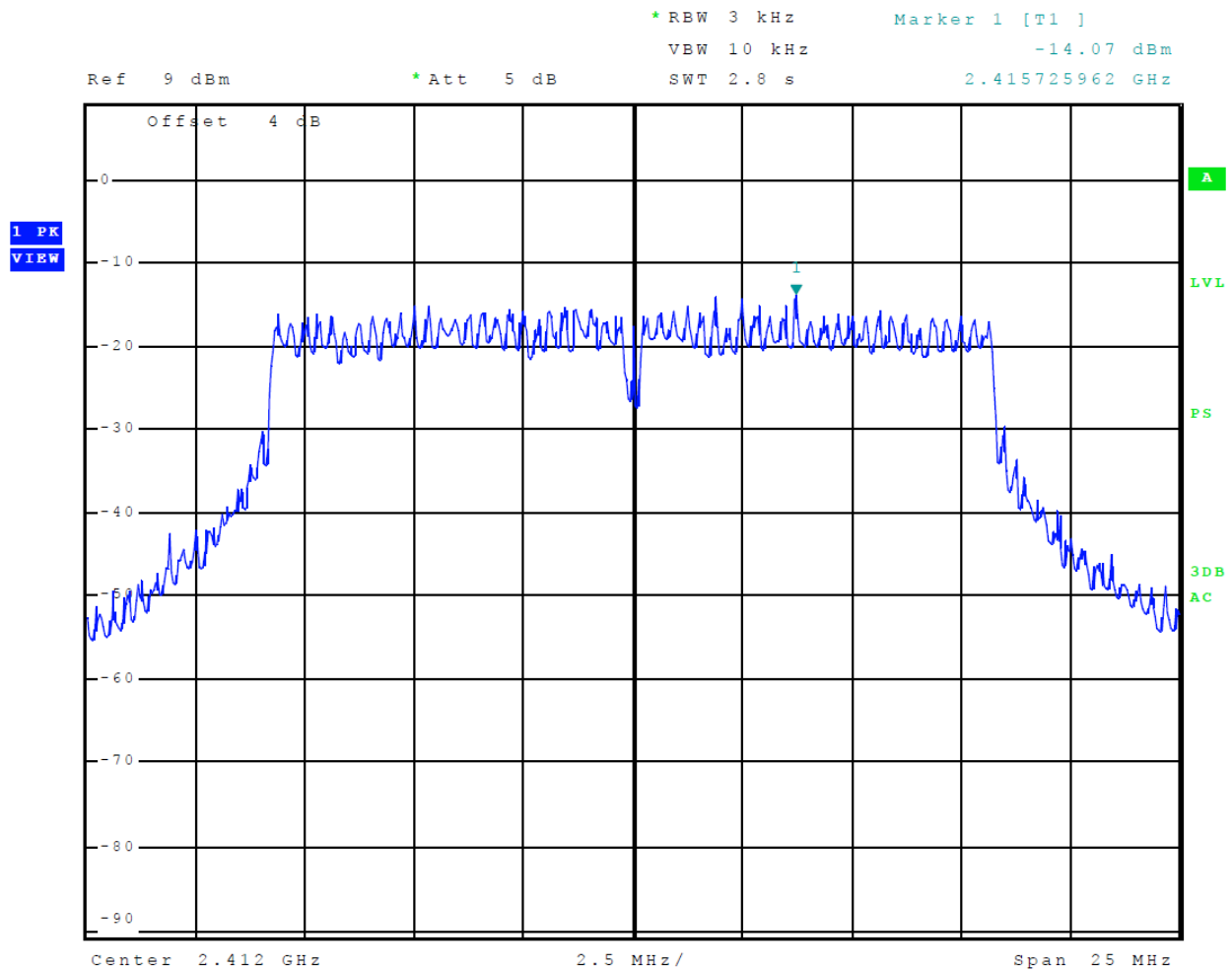
Figure 46 Plot of Transmitter Power Spectral Density (802.11g) Chain 1
