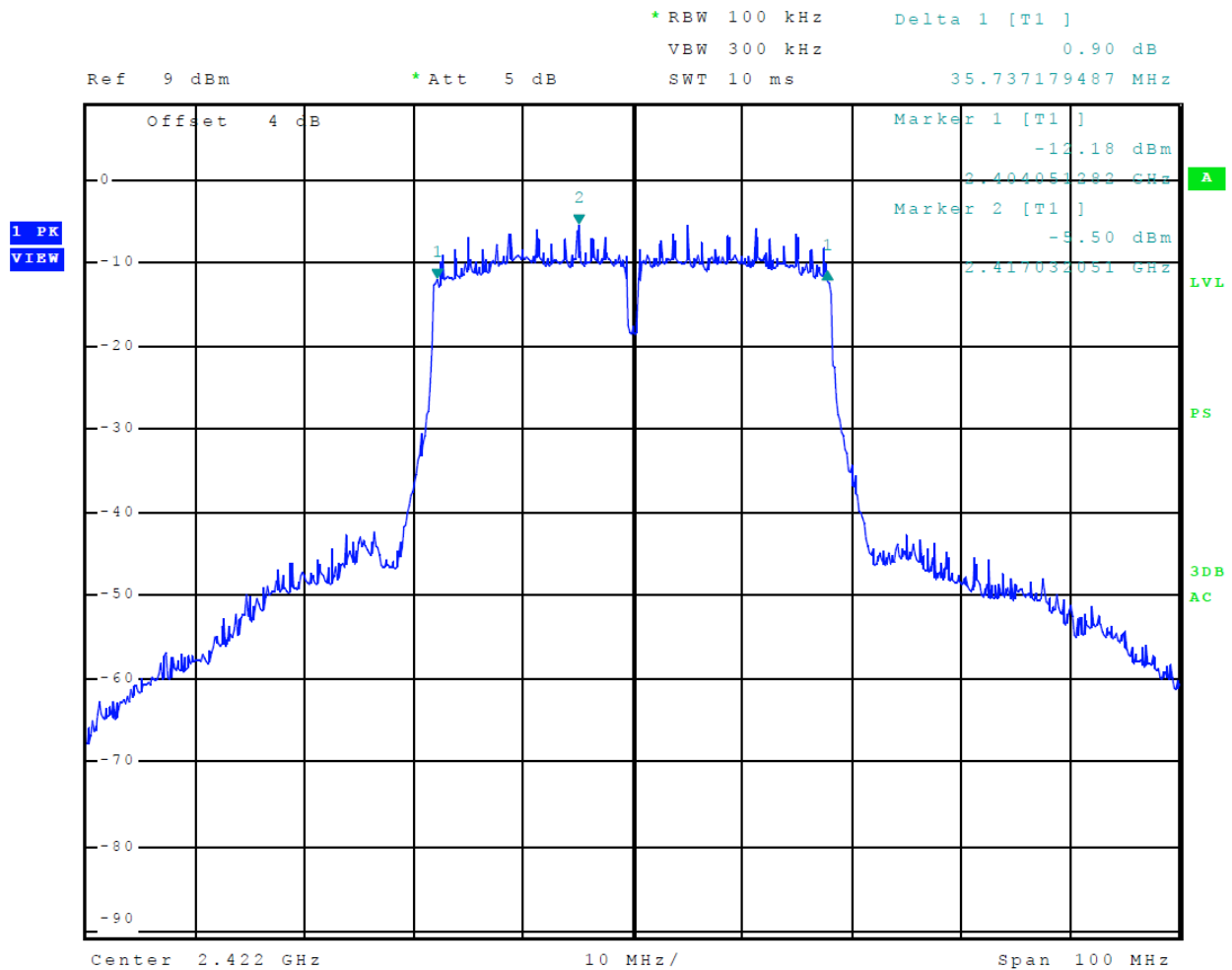
Figure 33 Plot of Transmitter 6-dB Occupied Band Width (802.11n40) Chain 0
