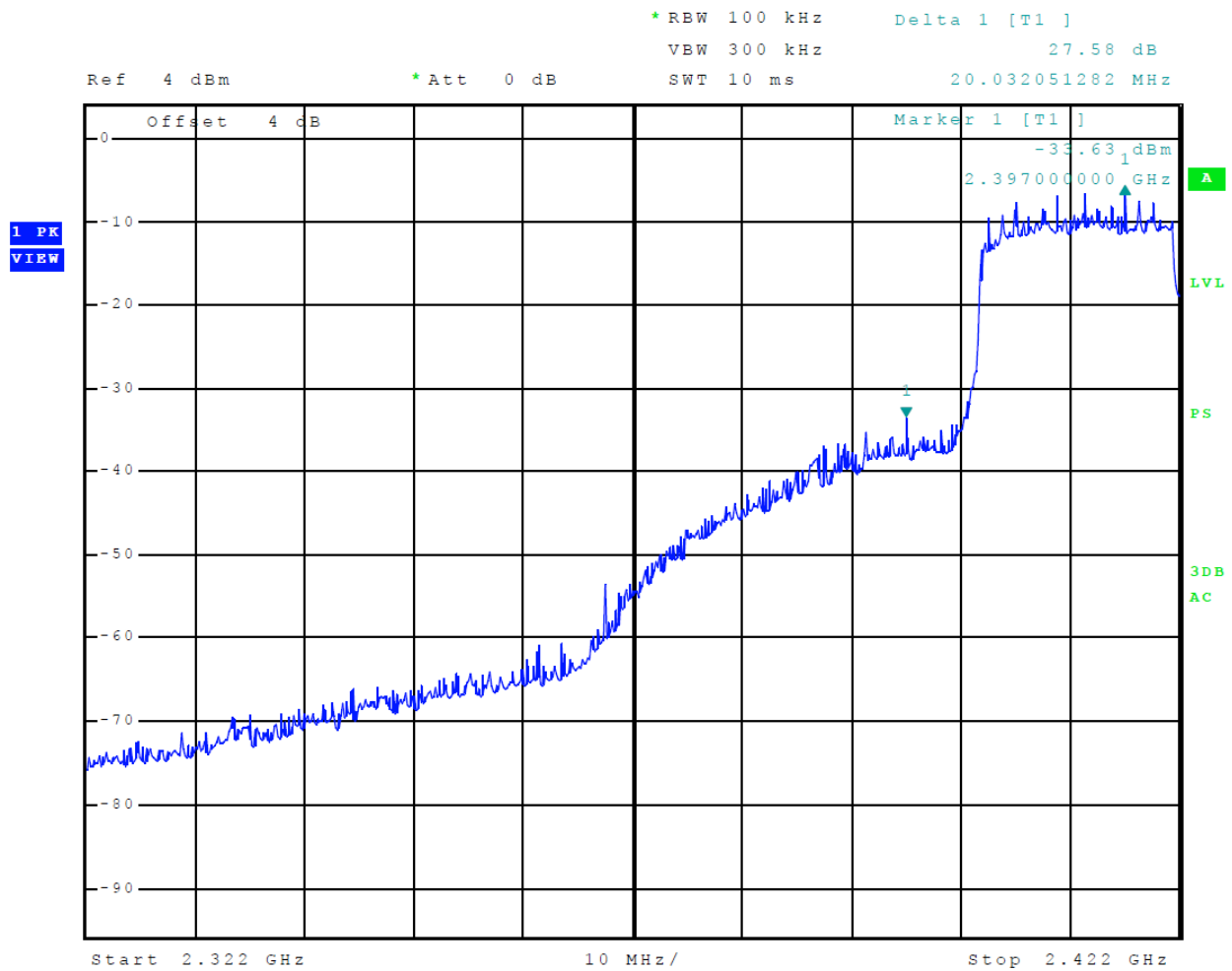
Figure 17 Plot of Transmitter Low Band Edge (802.11n40) Chain 0
