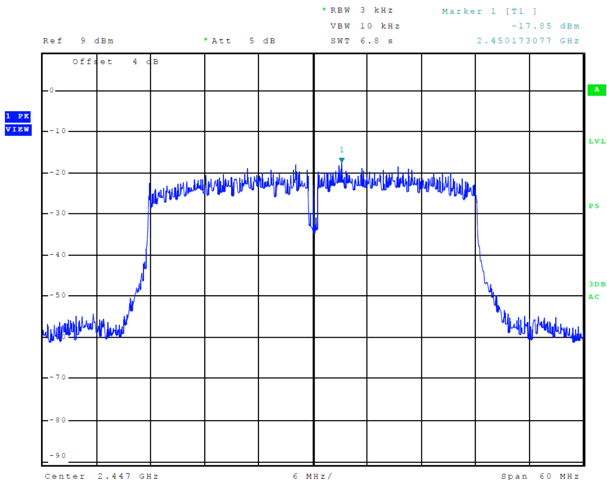
Figure 50 Plot of Transmitter Power Spectral Density (802.11n40) Chain 1
