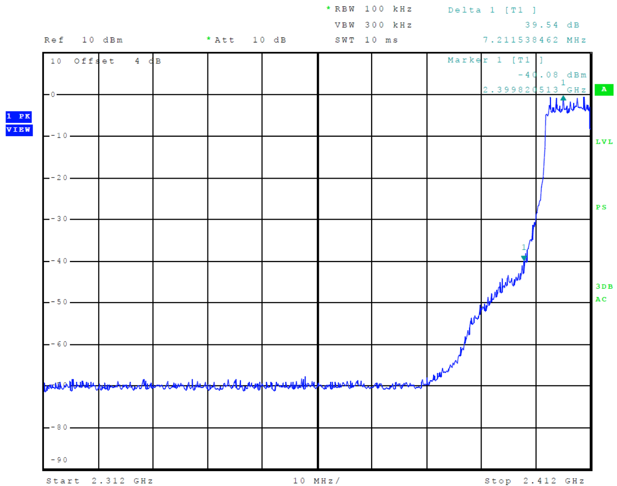
Figure 16 Plot of Transmitter Low Band Edge (802.11n) Chain 1
