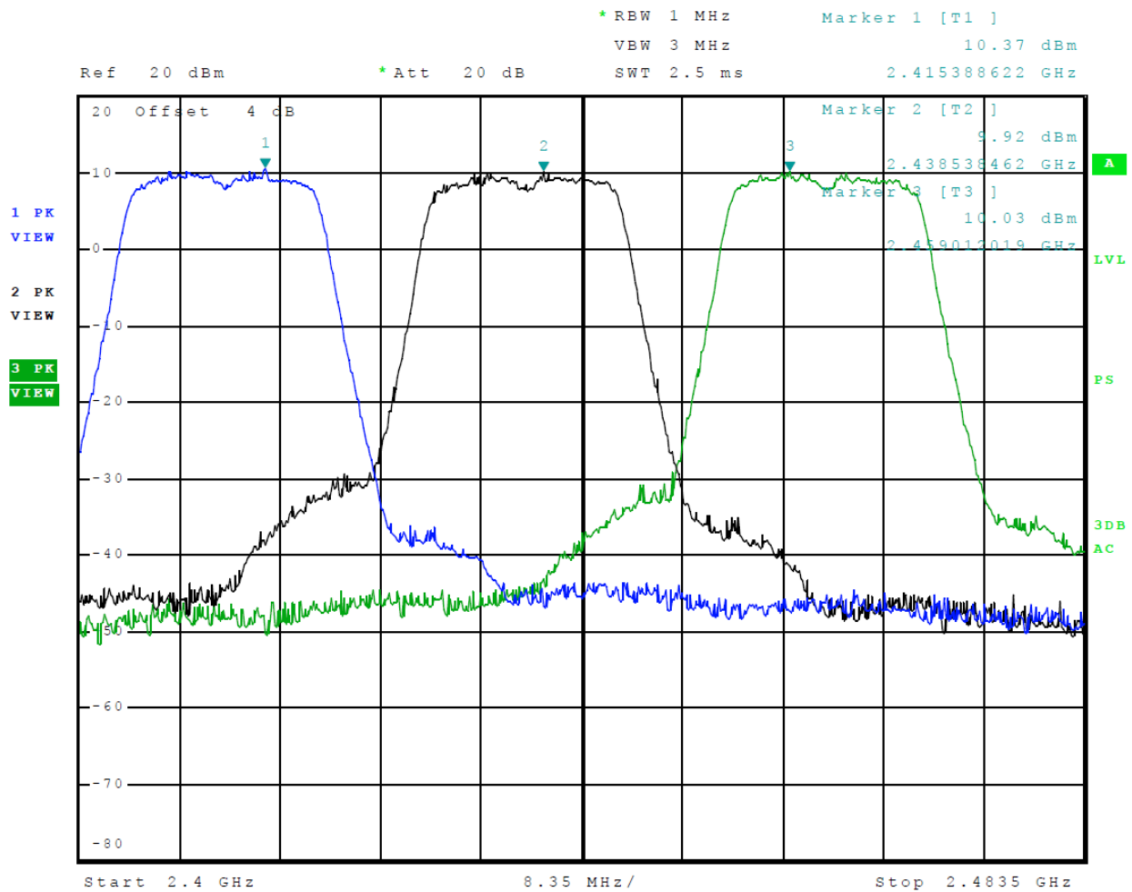
Figure 6 Plot of Transmitter Emissions (Across Operational Band, 802.11g) Chain 1
