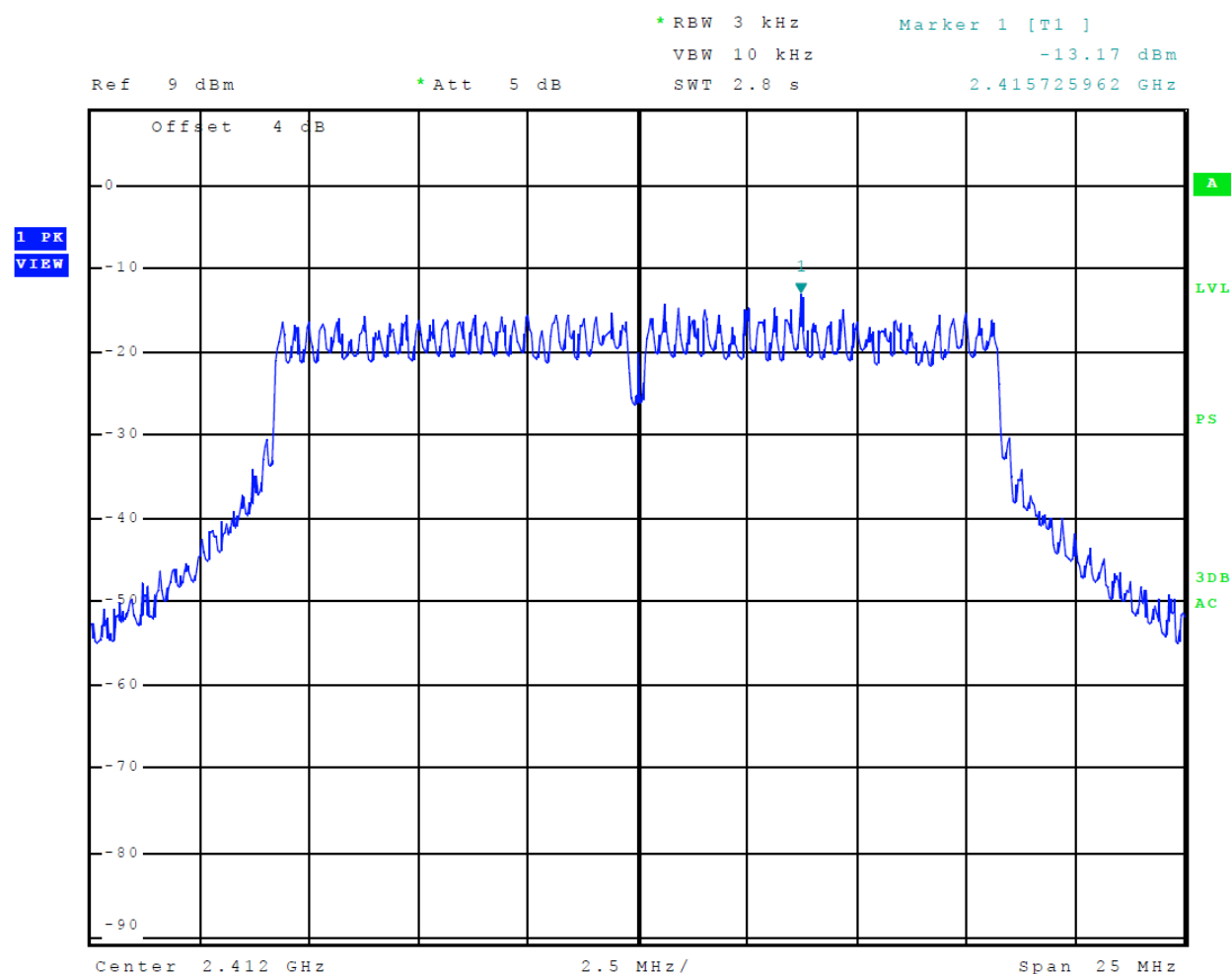
Figure 48 Plot of Transmitter Power Spectral Density (802.11n) Chain 1
