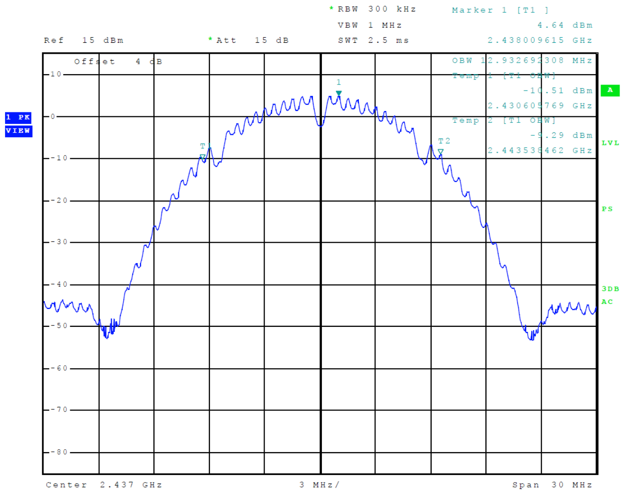
Figure 36 Plot of Transmitter 99% Occupied Band Width (802.11b) Chain 1
