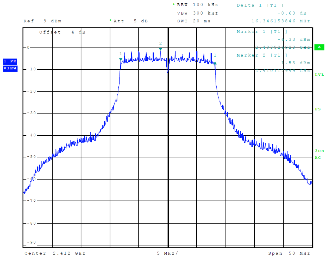
Figure 29 Plot of Transmitter 6-dB Occupied Band Width (802.11g) Chain 0
