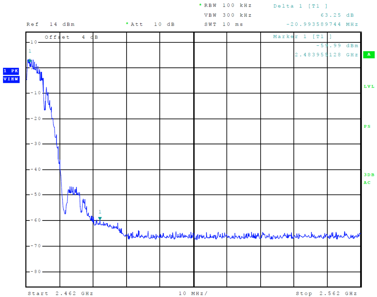
Figure 19 Plot of Transmitter High Band Edge (802.11b) Chain 0
