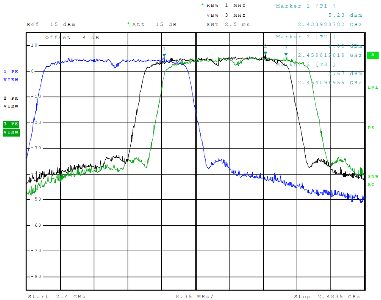
Figure 10 Plot of Transmitter Emissions (Across Operational Band, 802.11n40) Chain 1
