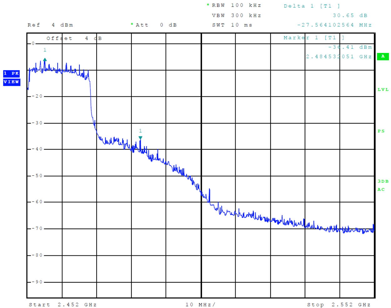
Figure 25 Plot of Transmitter High Band Edge (802.11n40) Chain 0
