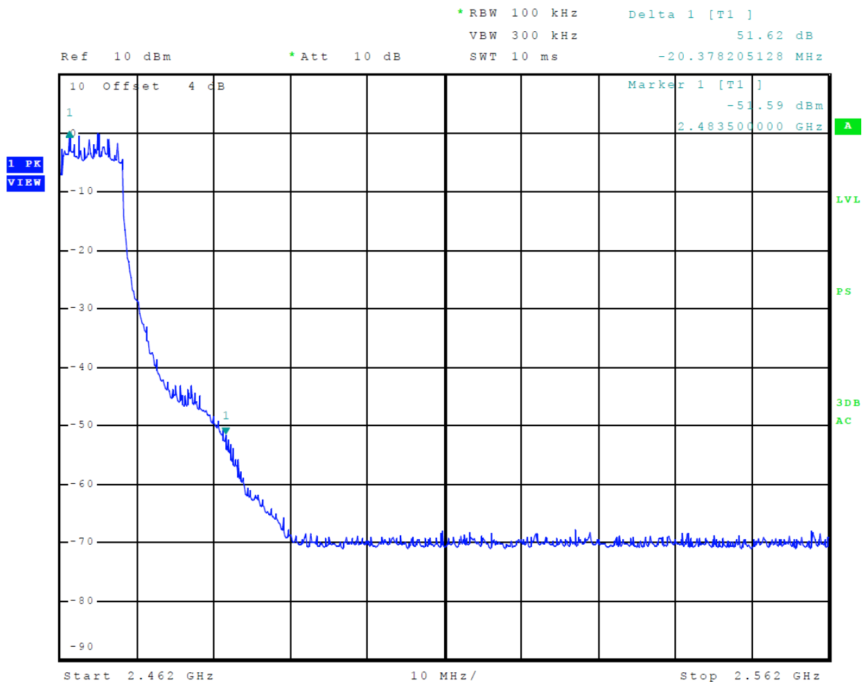
Figure 24 Plot of Transmitter High Band Edge (802.11n) Chain 1
