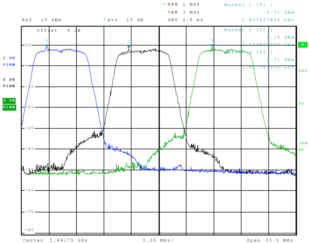
Figure 5 Plot of Transmitter Emissions (Across Operational Band, 802.11g) Chain 0
