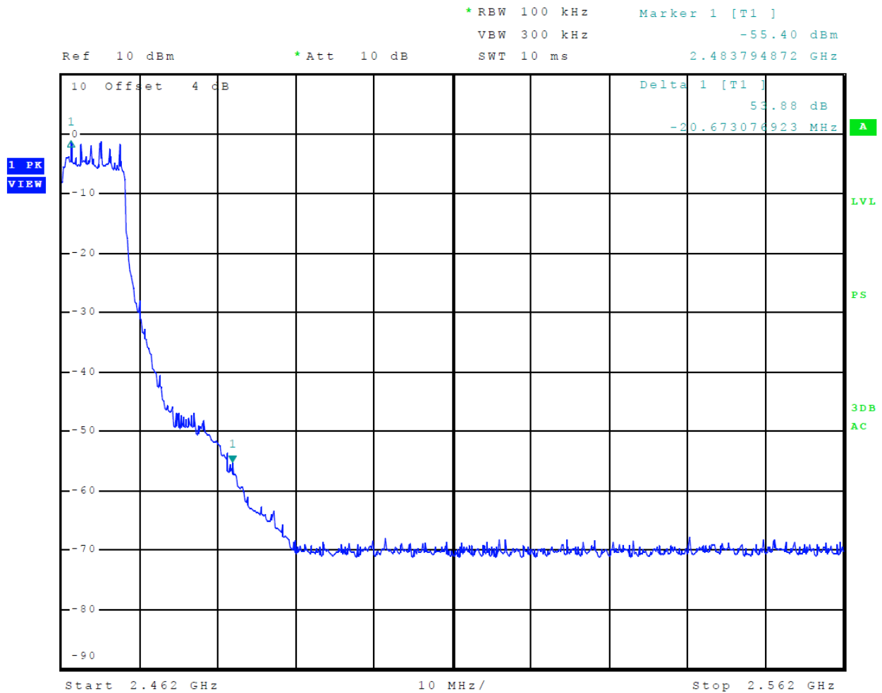
Figure 23 Plot of Transmitter High Band Edge (802.11n) Chain 0
