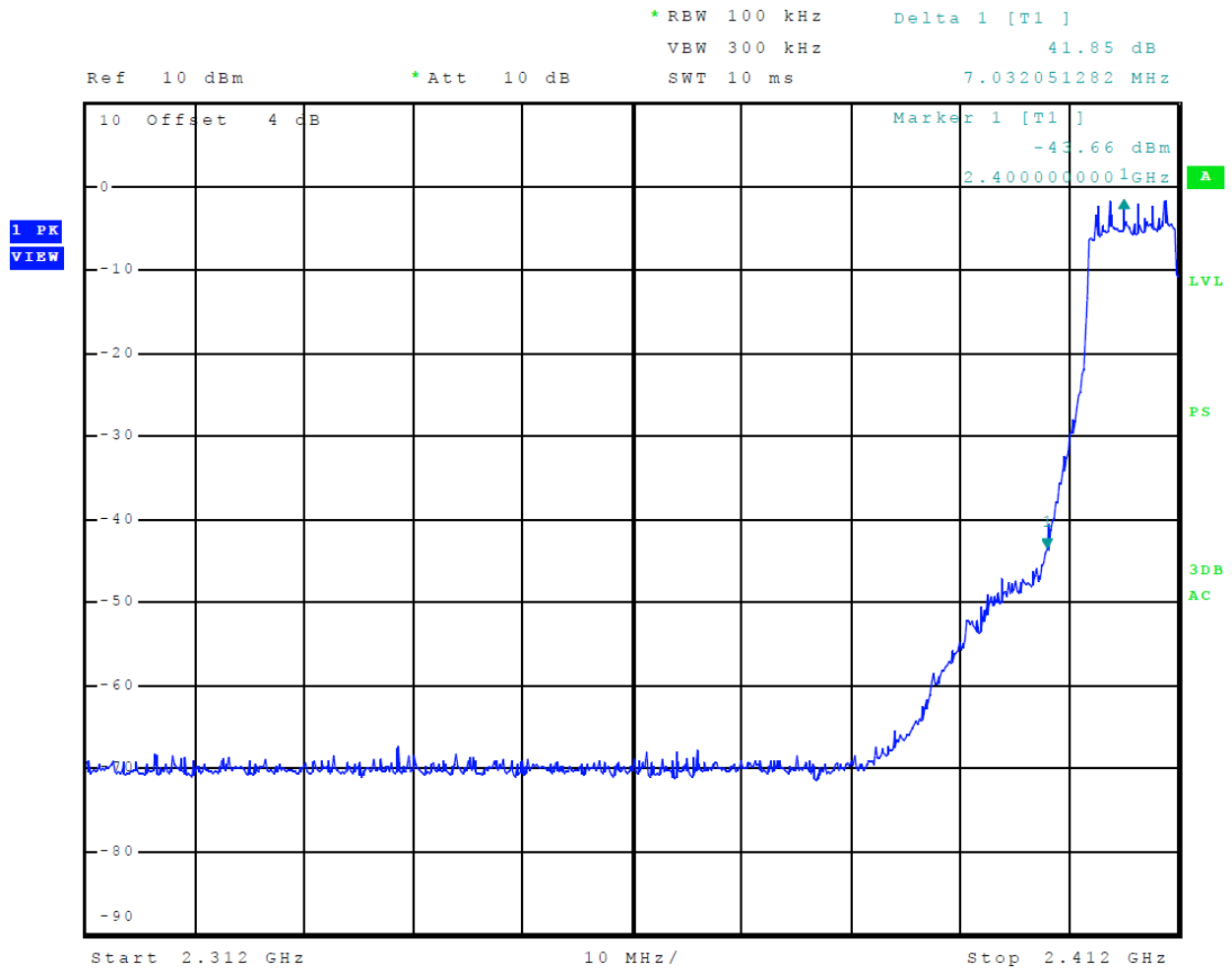
Figure 15 Plot of Transmitter Low Band Edge (802.11n) Chain 0
