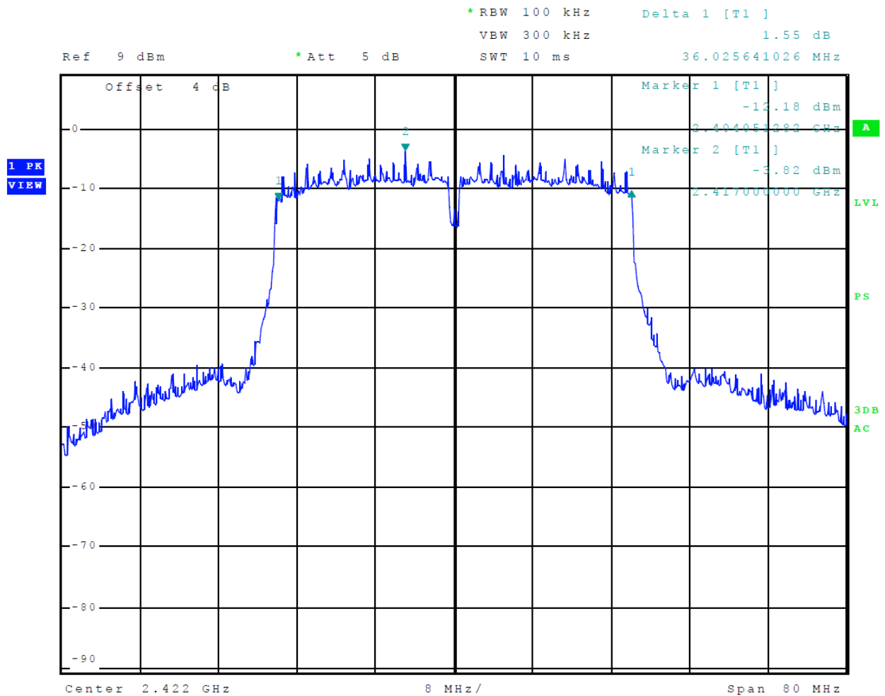
Figure 34 Plot of Transmitter 6-dB Occupied Band Width (802.11n40) Chain 1
