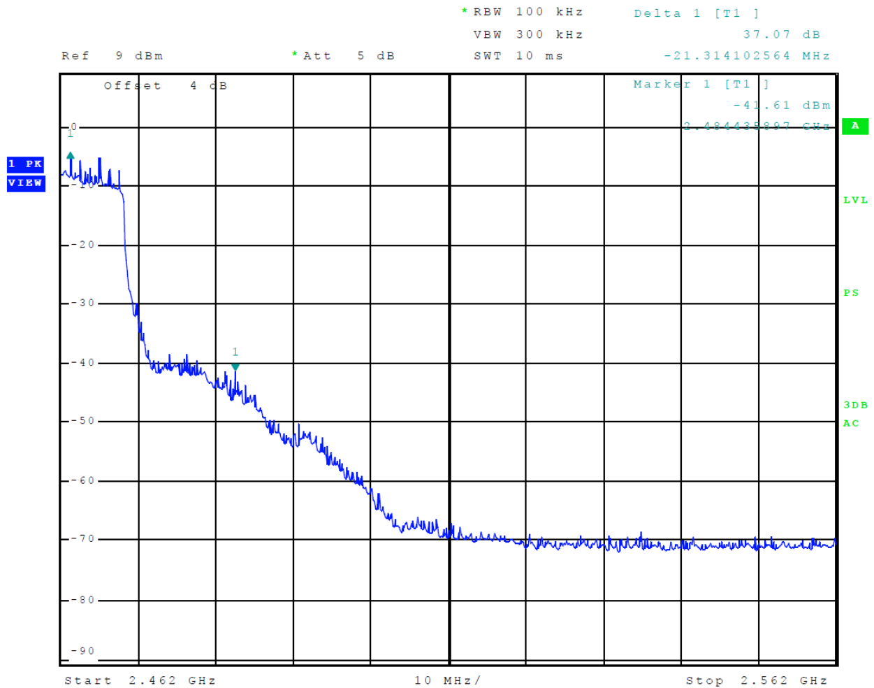
Figure 26 Plot of Transmitter High Band Edge (802.11n40) Chain 1
