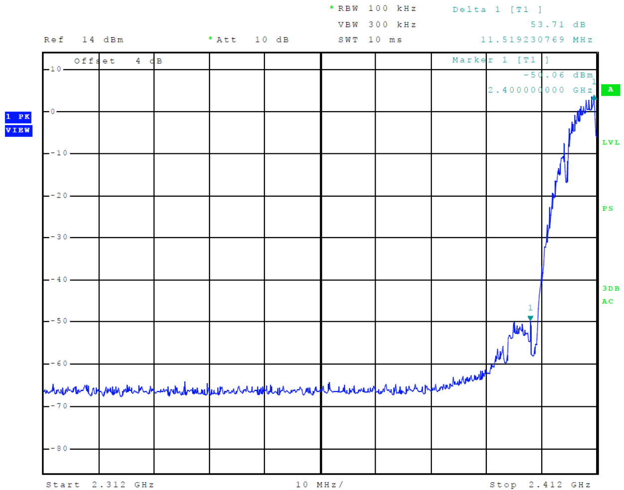
Figure 11 Plot of Transmitter Low Band Edge (802.11b) Chain 0
