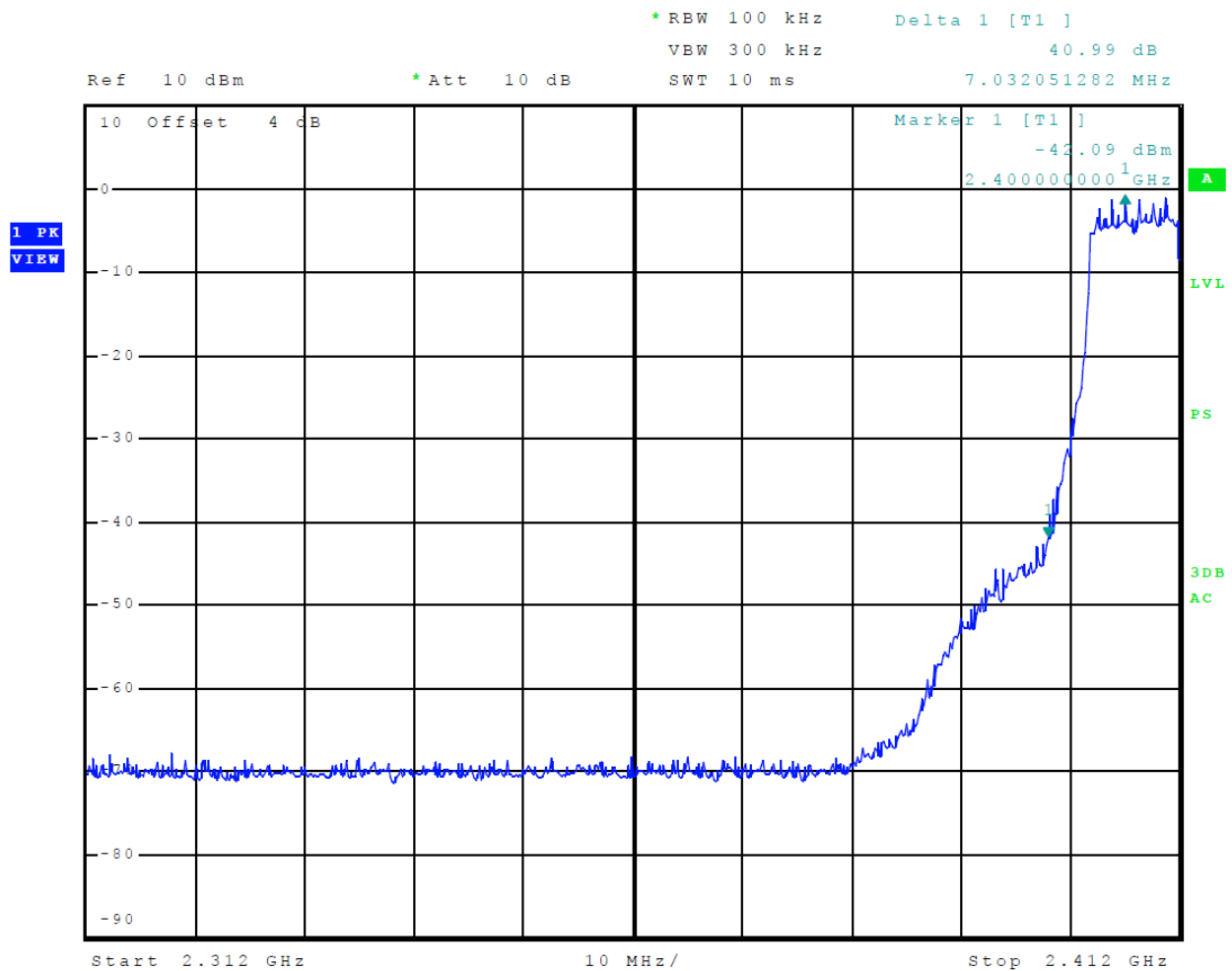
Figure 14 Plot of Transmitter Low Band Edge (802.11g) Chain 1
