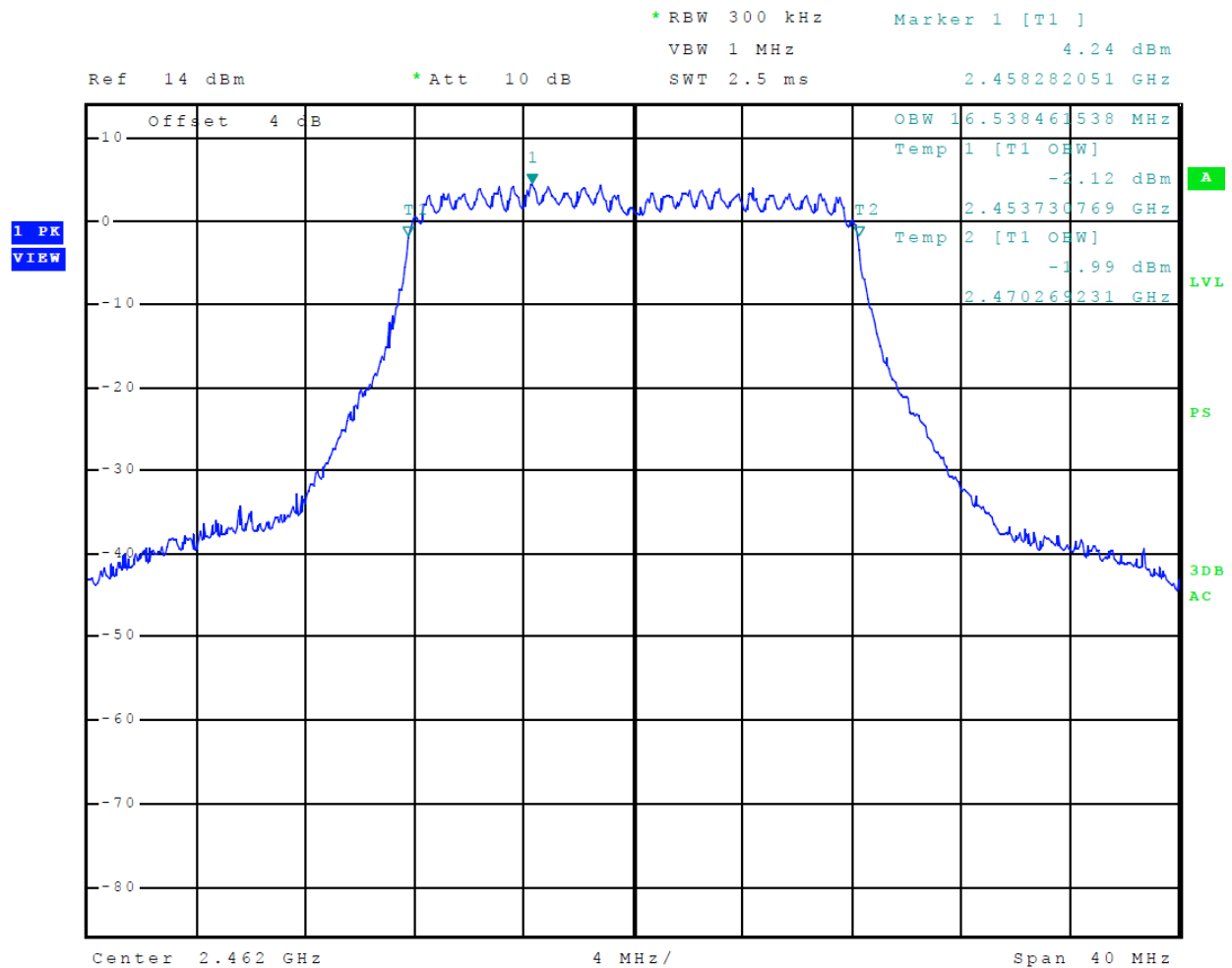
Figure 40 Plot of Transmitter 99% Occupied Band Width (802.11n) Chain 1
