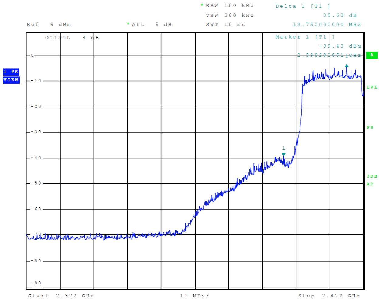
Figure 18 Plot of Transmitter Low Band Edge (802.11n40) Chain 1
