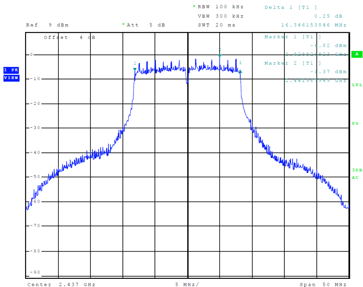
Figure 31 Plot of Transmitter 6-dB Occupied Band Width (802.11n) Chain 0
