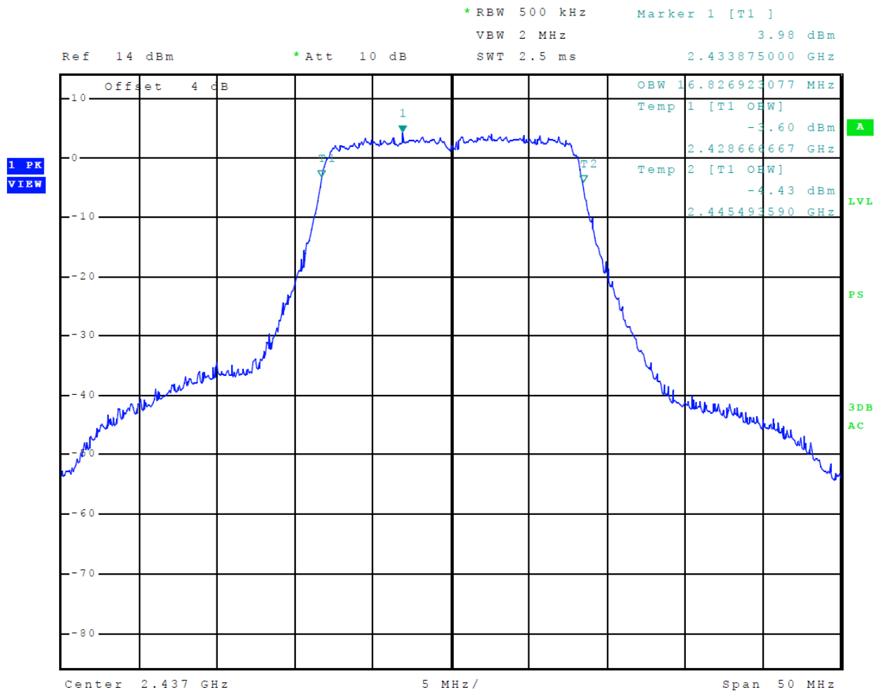
Figure 39 Plot of Transmitter 99% Occupied Band Width (802.11n) Chain 0
