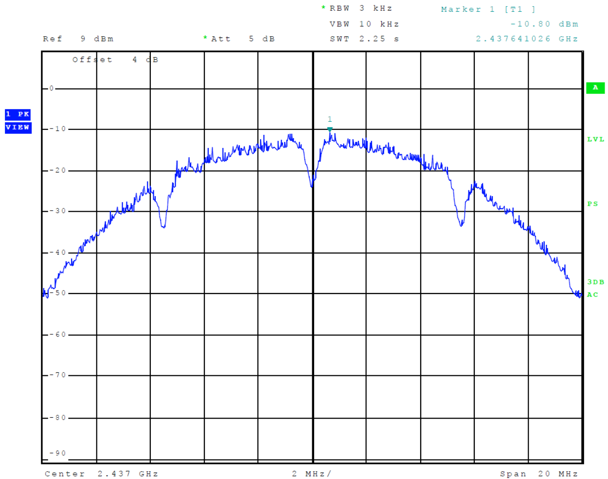
Figure 44 Plot of Transmitter Power Spectral Density (802.11b) Chain 1
