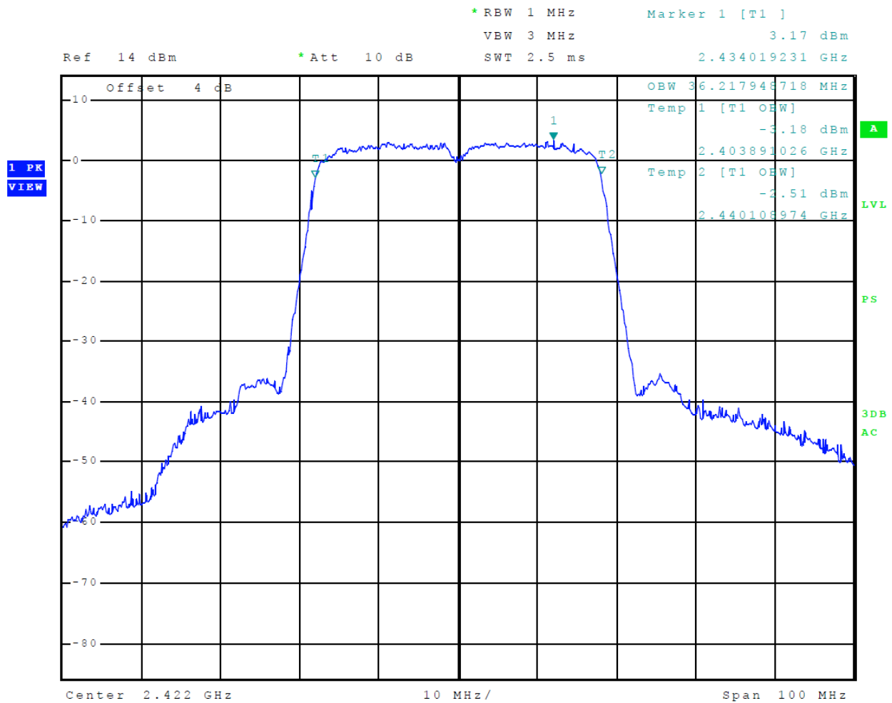
Figure 41 Plot of Transmitter 99% Occupied Band Width (802.11n40) Chain 0
