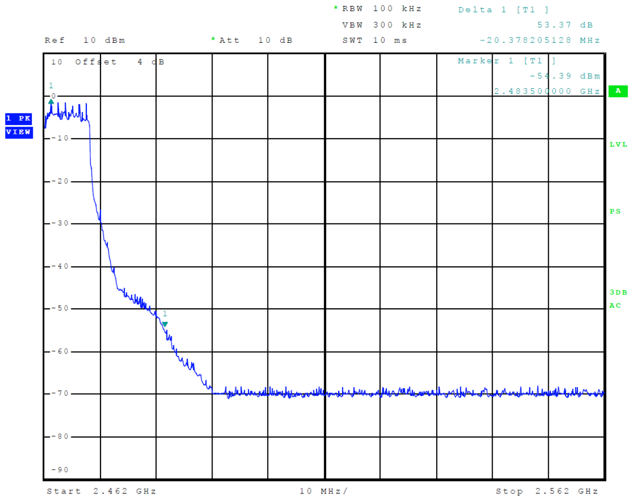
Figure 21 Plot of Transmitter High Band Edge (802.11g) Chain 0
