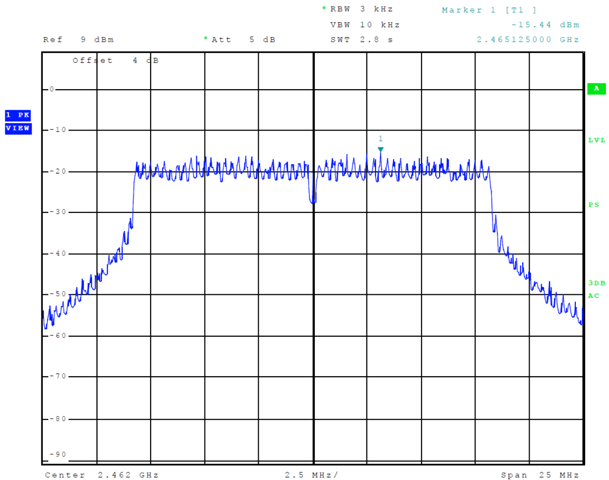
Figure 45 Plot of Transmitter Power Spectral Density (802.11g) Chain 0
