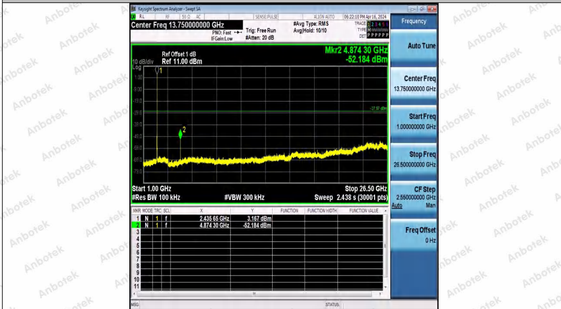
11B-Ant1-2437-1000~26500-PASS
