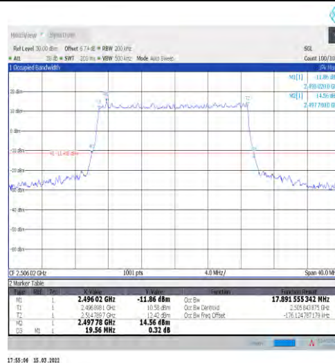
1-N41-30-20-L-4-DFT-64QAM-Outer_Full-50@0-Ant 1-17.892-19.560-≤20-PASS
