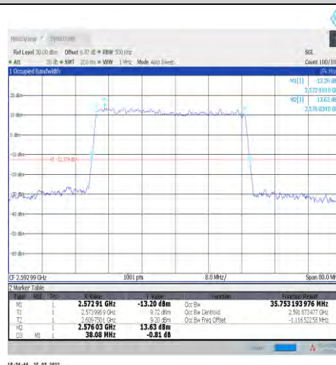
1-N41-30-40-M-5-DFT-256QAM-Outer_Full-100@0-A Ant1-35.753-38.080-≤40-PASS
