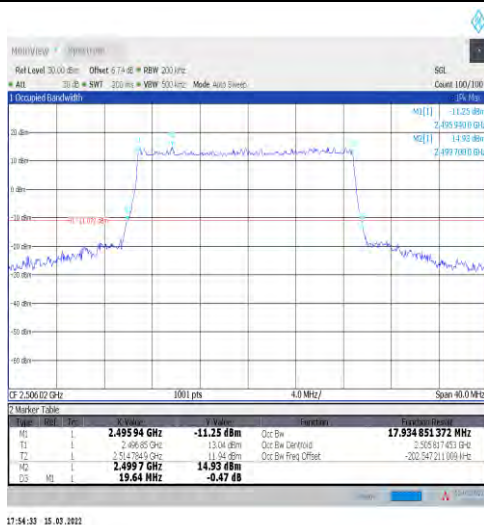
1-N41-30-20-L-3-DFT-16QAM-Outer_Full-50@0-Ant 1-17.935-19.640-≤20-PASS
