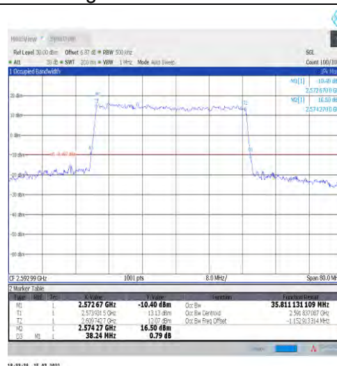
1-N41-30-40-M-3-DFT-16QAM-Outer_Full-100@0-A nt1-35.811-38.240-≤40-PASS
