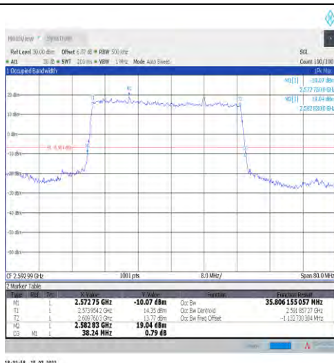
1-N41-30-40-M-2-DFT-PI2BPSK-Outer_Full-100@0-A Ant1-35.806-38.240-≤40-PASS
