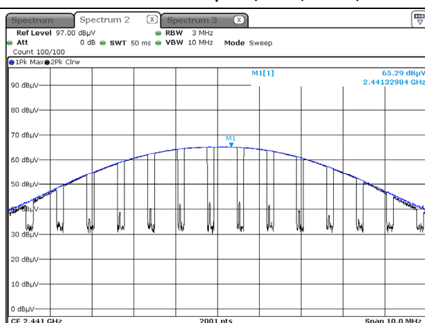
Radiated Power plot (GFSK, Ch.39)
