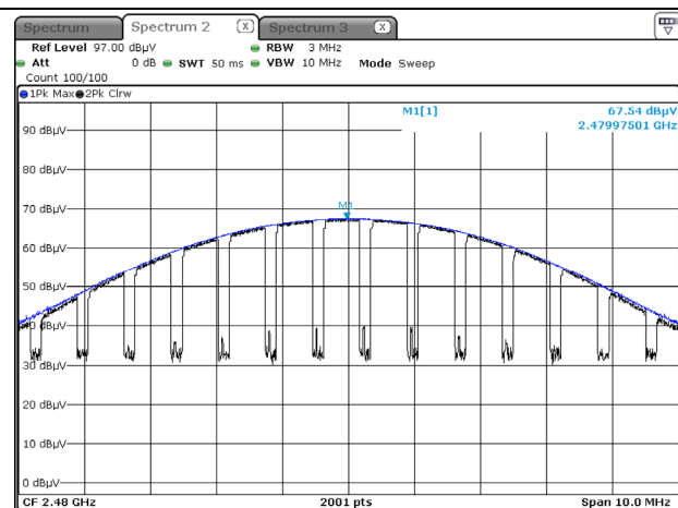
Radiated Power plot (8DPSK, Ch.78)
