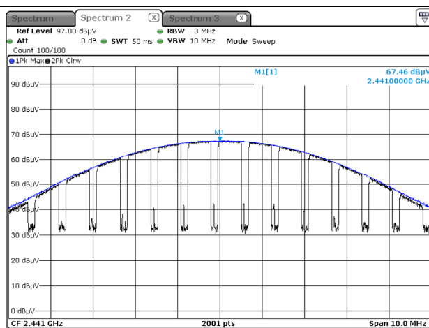
Radiated Power plot ( \pi/4 DQPSK, Ch.39)
