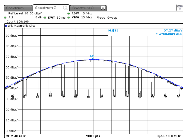
Radiated Power plot (G \pi/4 DQPSK, Ch.78)
