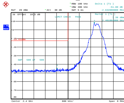
GFSK_Low
