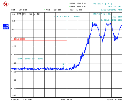
GFSK_Hopping_Lower
