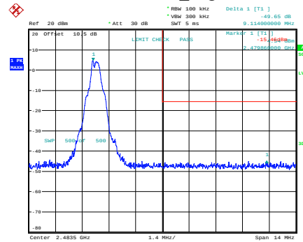
GFSK_High
