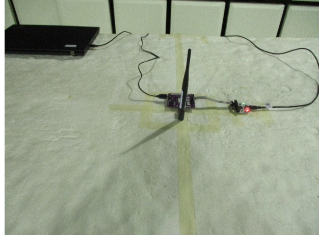
FCC_15_247_902~928MHz_OFDM_Conducted_Setup
