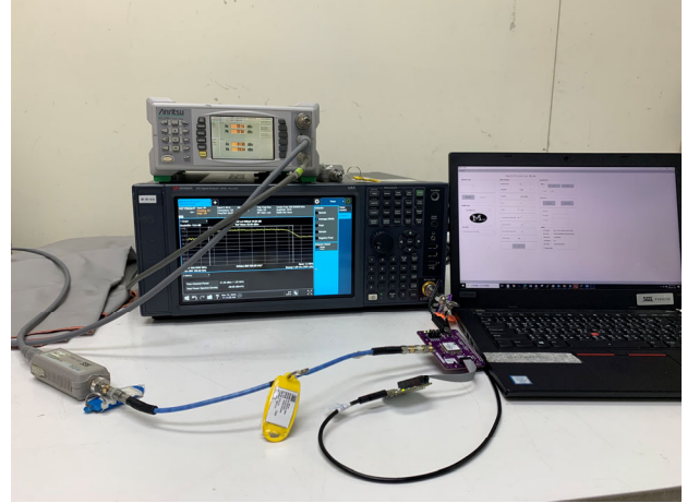
FCC_15_247_902~928MHz_OFDM_Conducted_Setup
