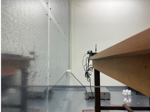
FCC_15_247_902~928MHz_OFDM_Conduction_Setup
