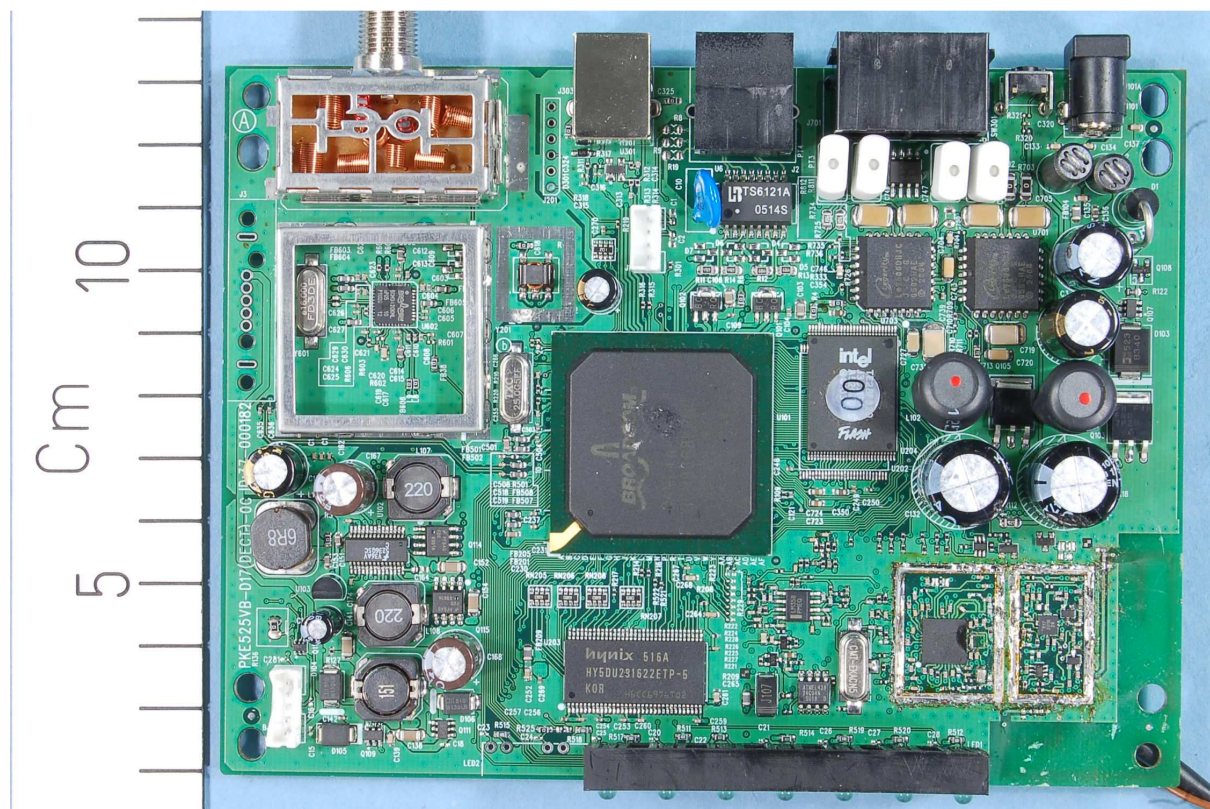
DPC2223 – Radiated Sample Without Shielding
