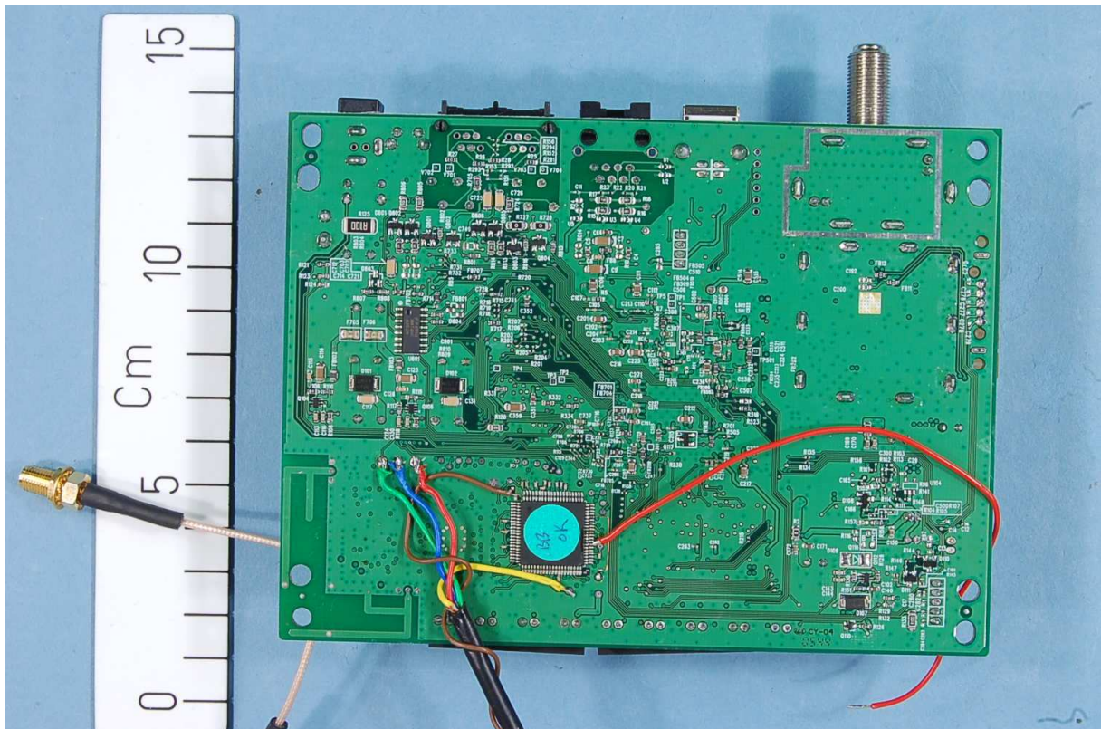
DPC2223 – Conducted Sample
