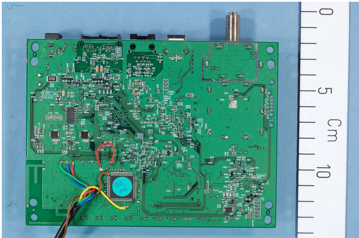
DPC2223 – Radiated Sample
