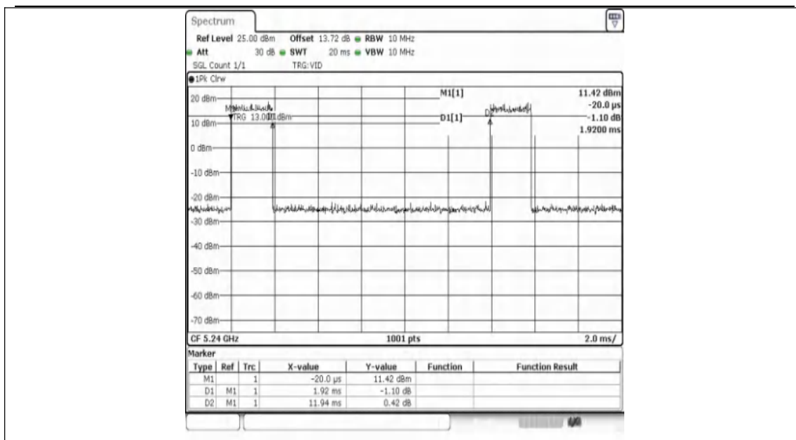
NTNV-11AX20SISO-Ant1-5240
