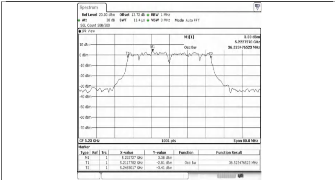
11AC40SISO-Ant1-5230
