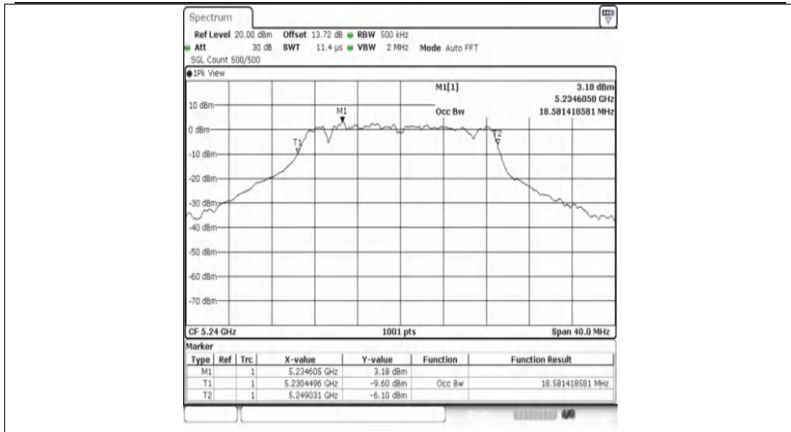
11AX20SISO-Ant1-5240
