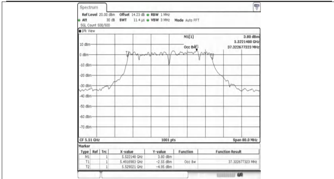
11N40SISO-Ant1-5510
