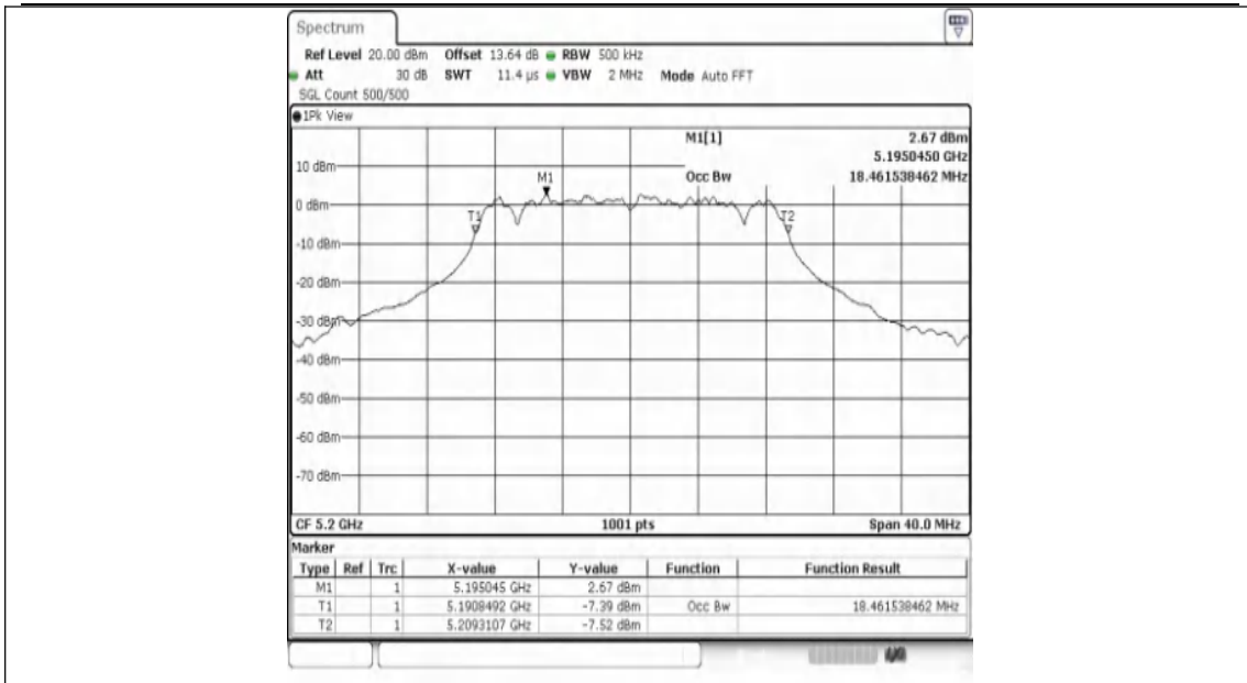
11AC20SISO-Ant1-5200
