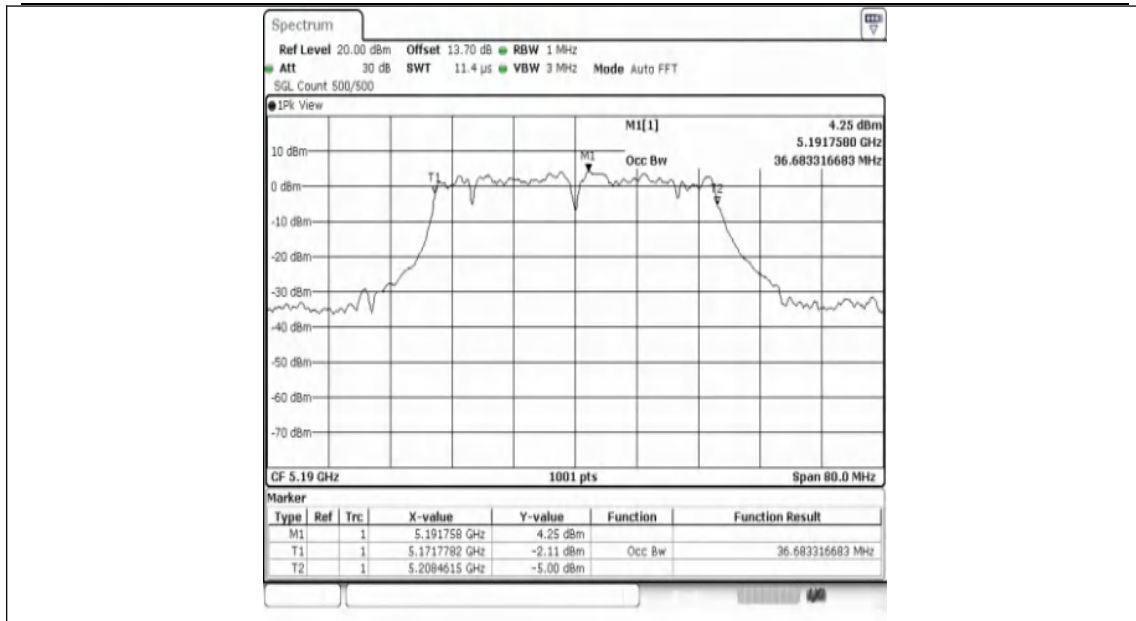
11N40SISO-Ant1-5190
