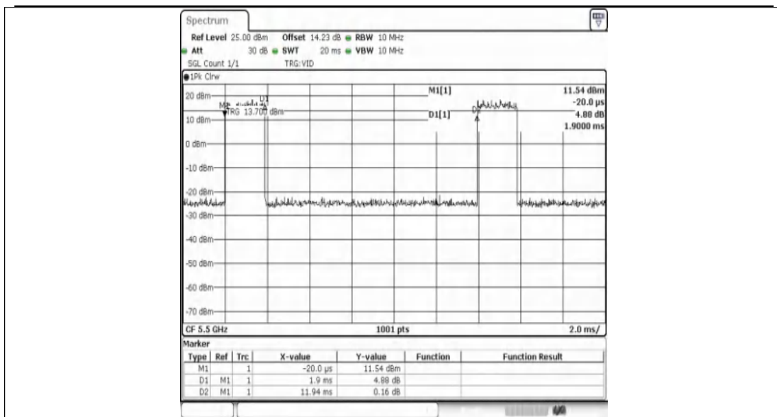
NTNV-11AX20SISO-Ant1-5500
