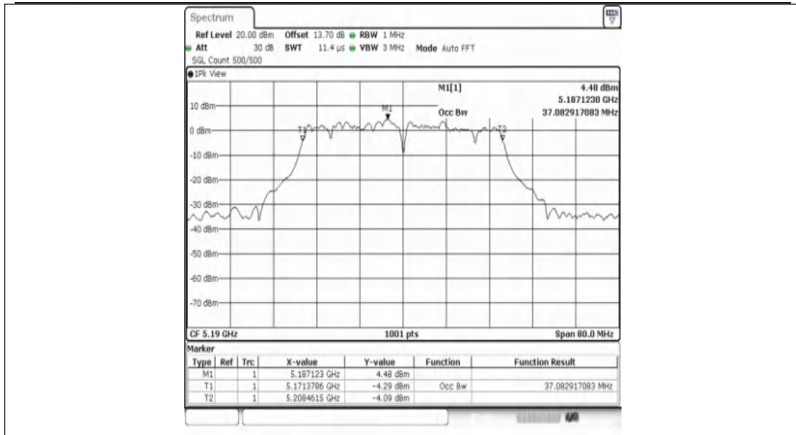
11AX40SISO-Ant1-5190
