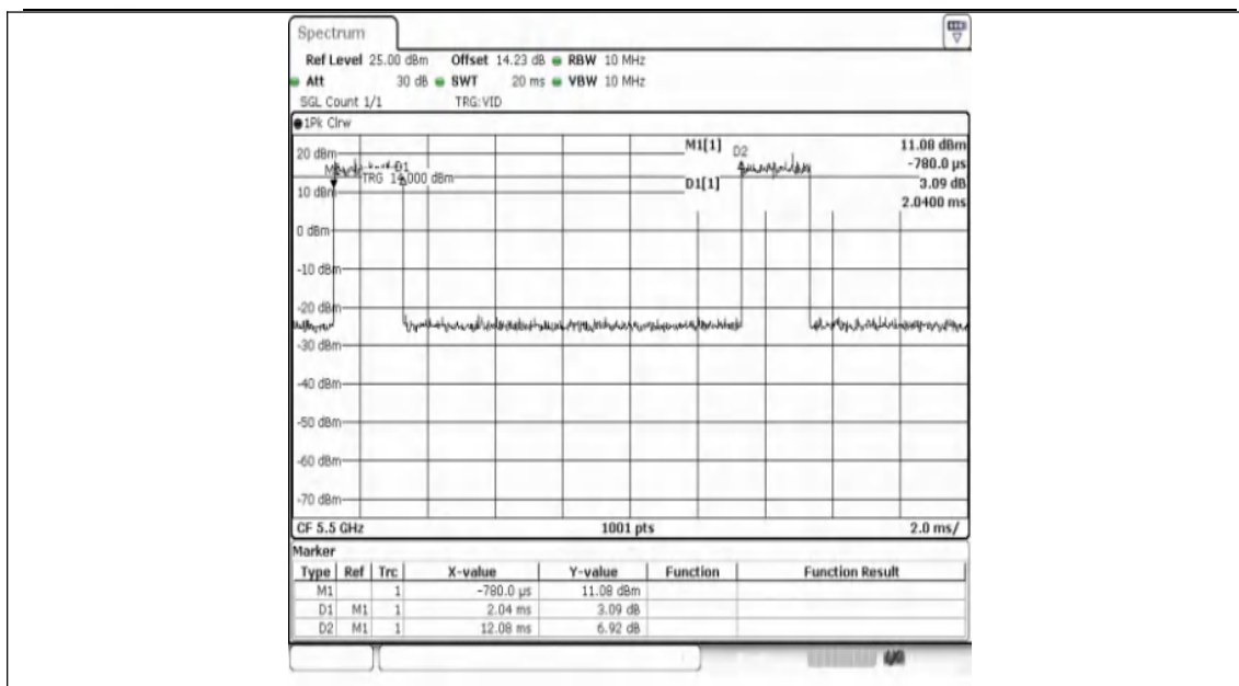
NTNV-11A-Ant1-5500
