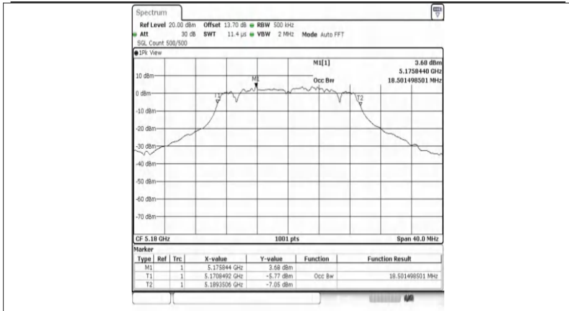
11AX20SISO-Ant1-5180
