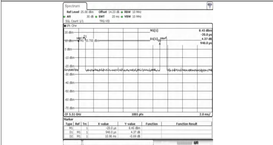
NTNV-11AC40SISO-Ant1-5510
