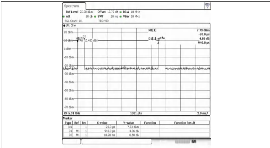
NTNV-11AC40SISO-Ant1-5310
