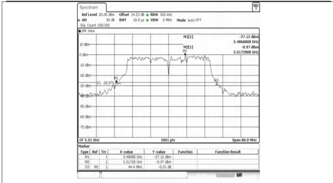
11AX40SISO-Ant1-5510
