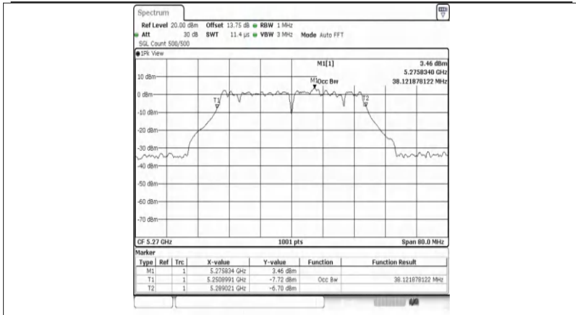
11AX40SISO-Ant1-5270
