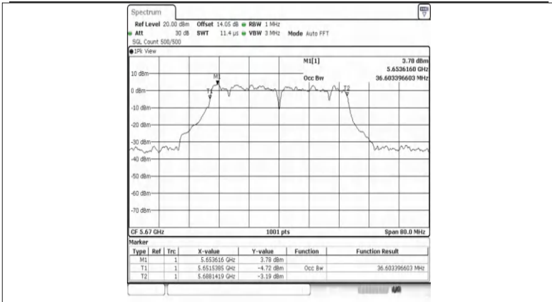
11AX40SISO-Ant1-5670
