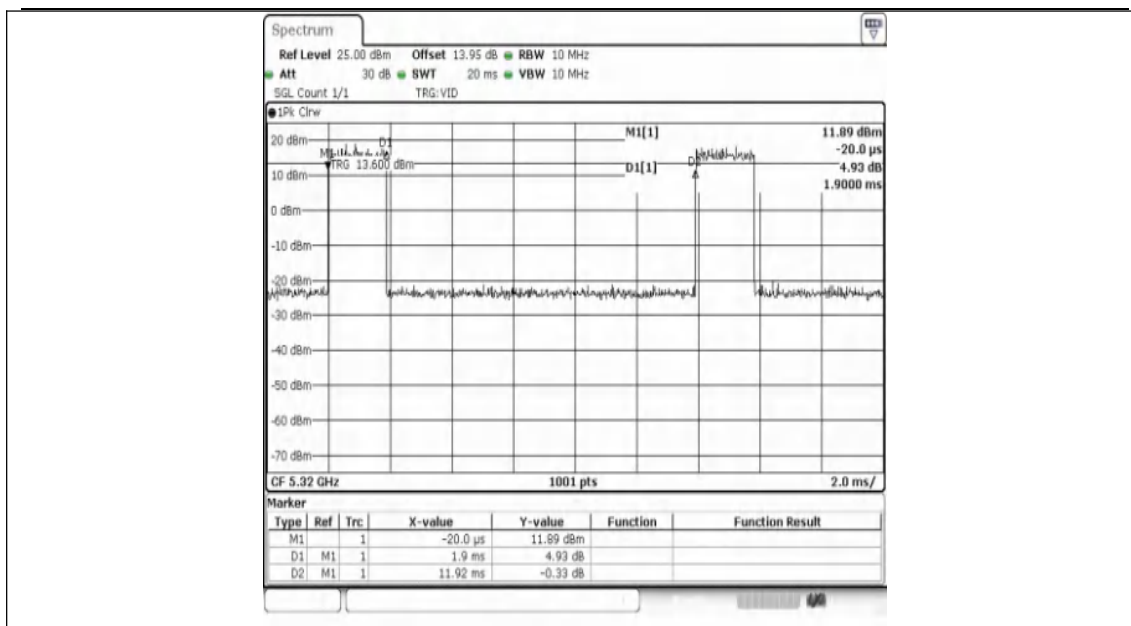
NTNV-11AC20SISO-Ant1-5320
