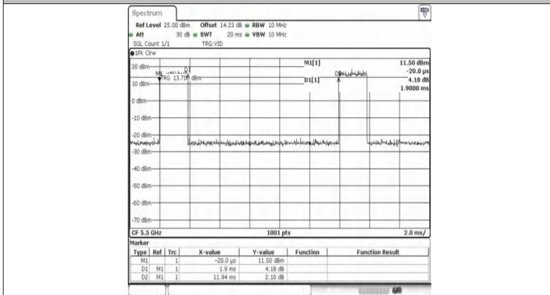
NTNV-11AC20SISO-Ant1-5500
