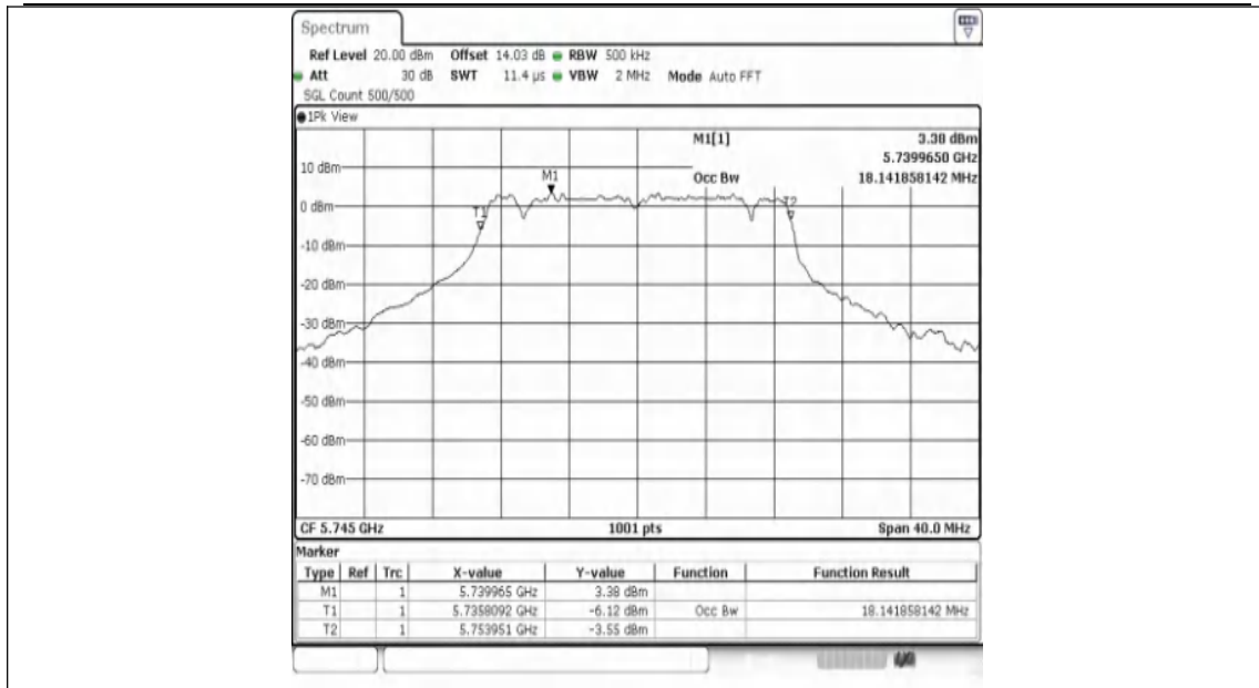
11AC20SISO-Ant1-5745
