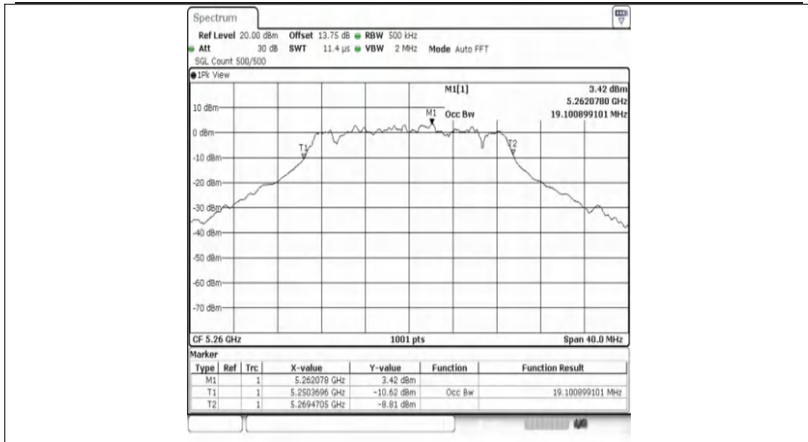
11AC20SISO-Ant1-5260
