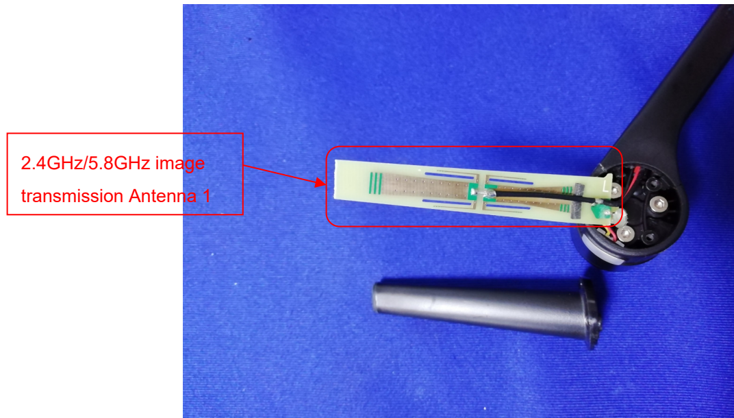
Front view of Original antenna 1
