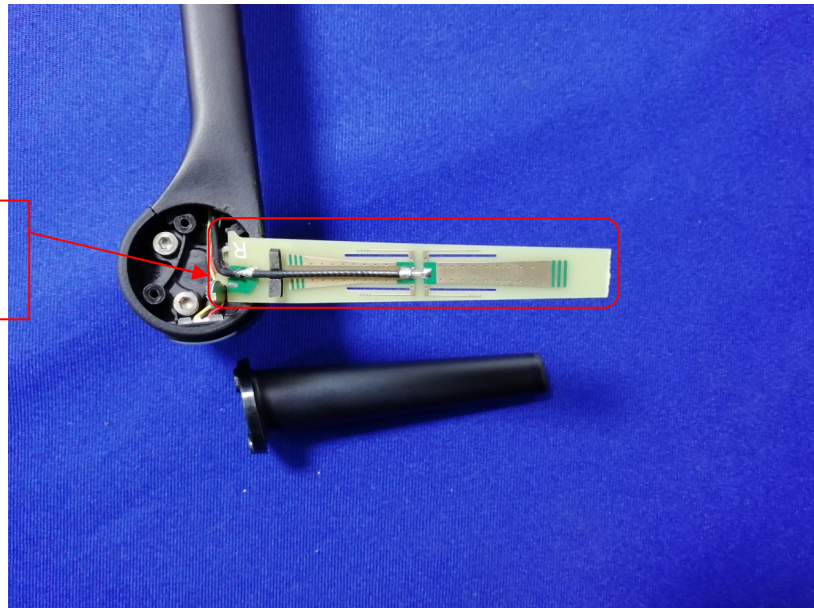
Front view of Original antenna 2
