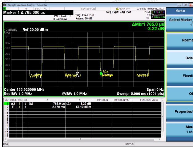
T on2
