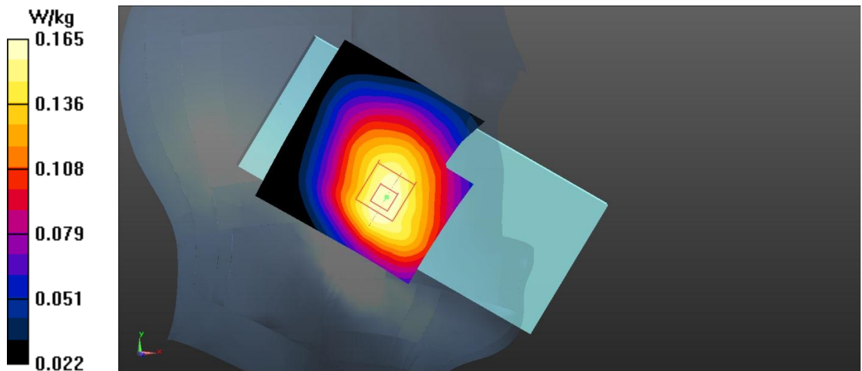
Fig.21 LTE Band 28 Head
