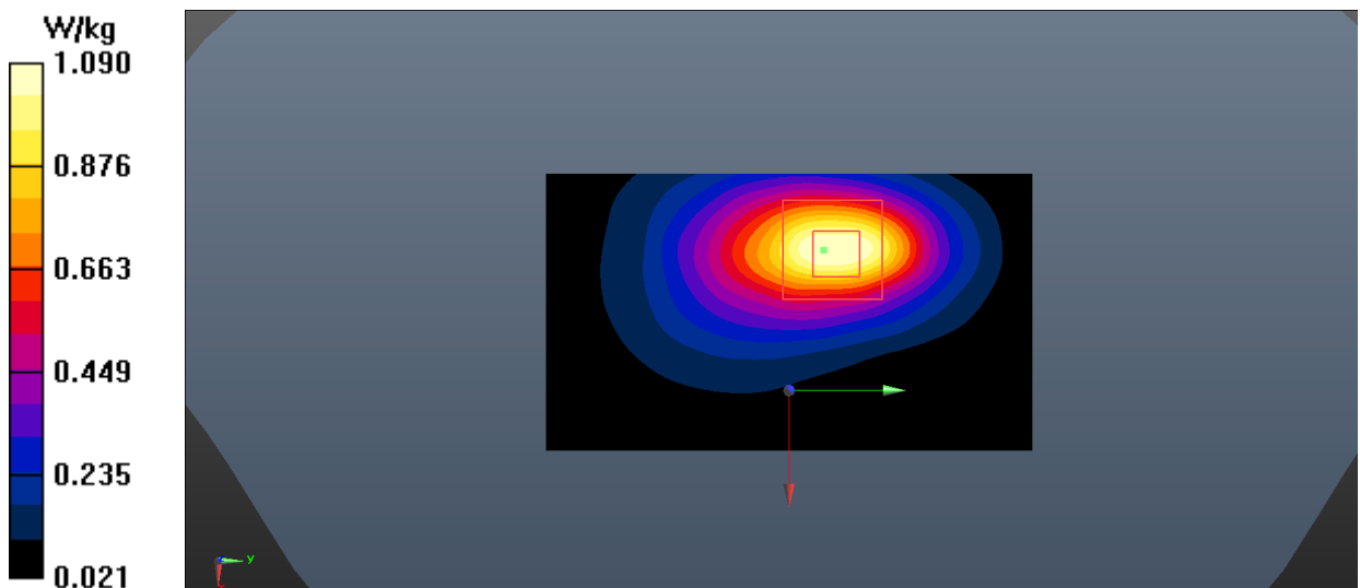
Fig.12 LTE Band 2 Body
