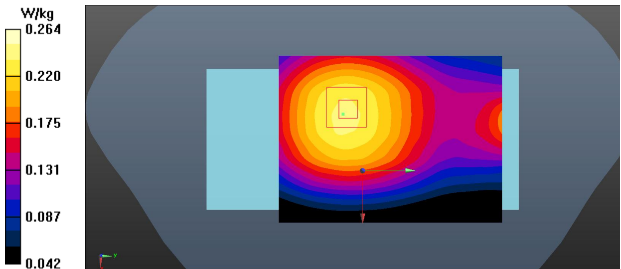
Fig.20 LTE Band 13 Body
