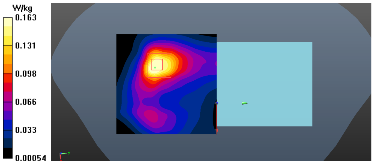
Fig.26 WLAN 2.4G Body
