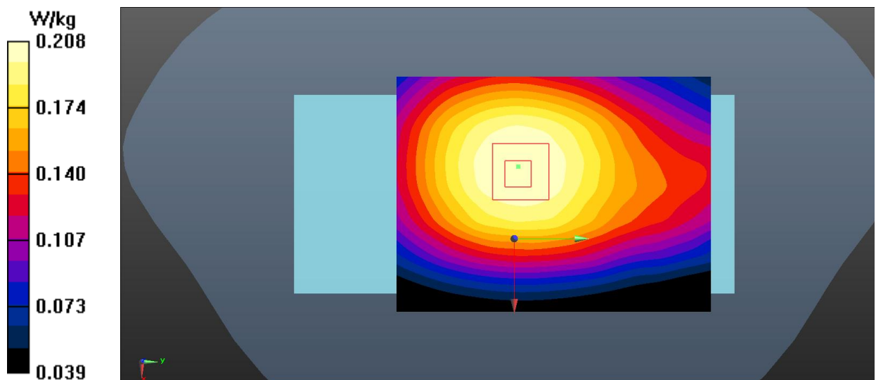
Fig.18 LTE Band 12 Body
