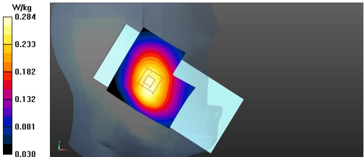
Fig.13 LTE Band 5 Head
