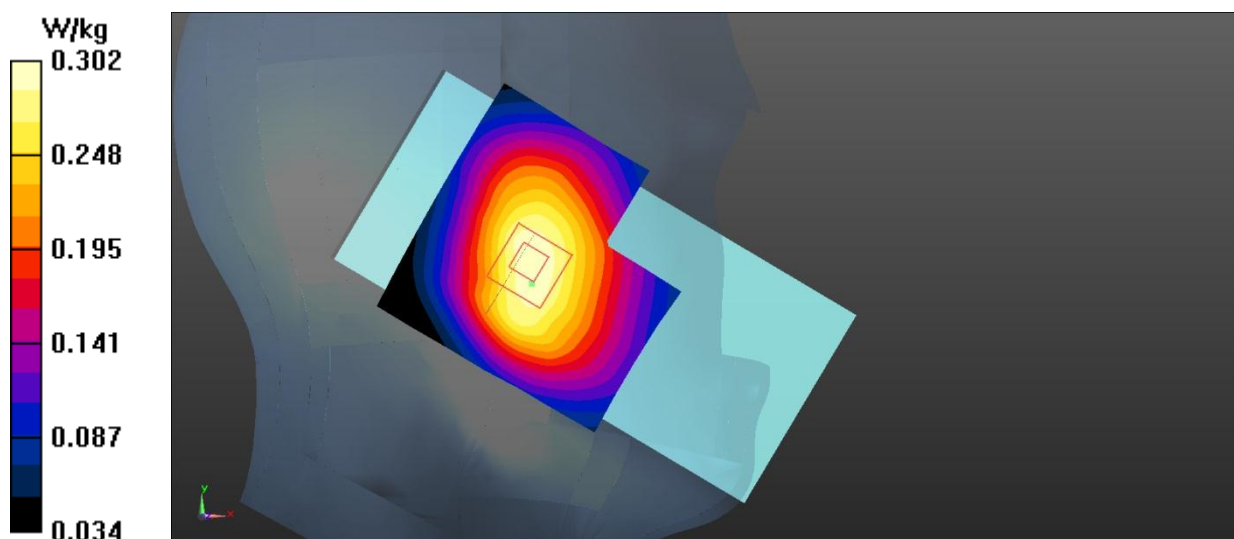
Fig.9 WCDMA Band 5 Head
