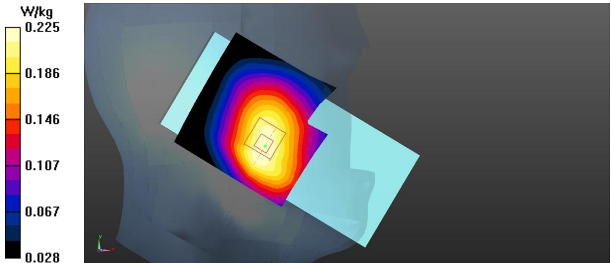
Fig.19 LTE Band 13 Head
