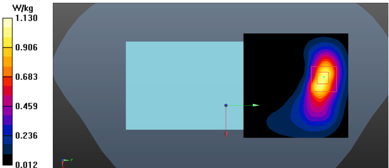
Fig.24 LTE Band 66 Body
