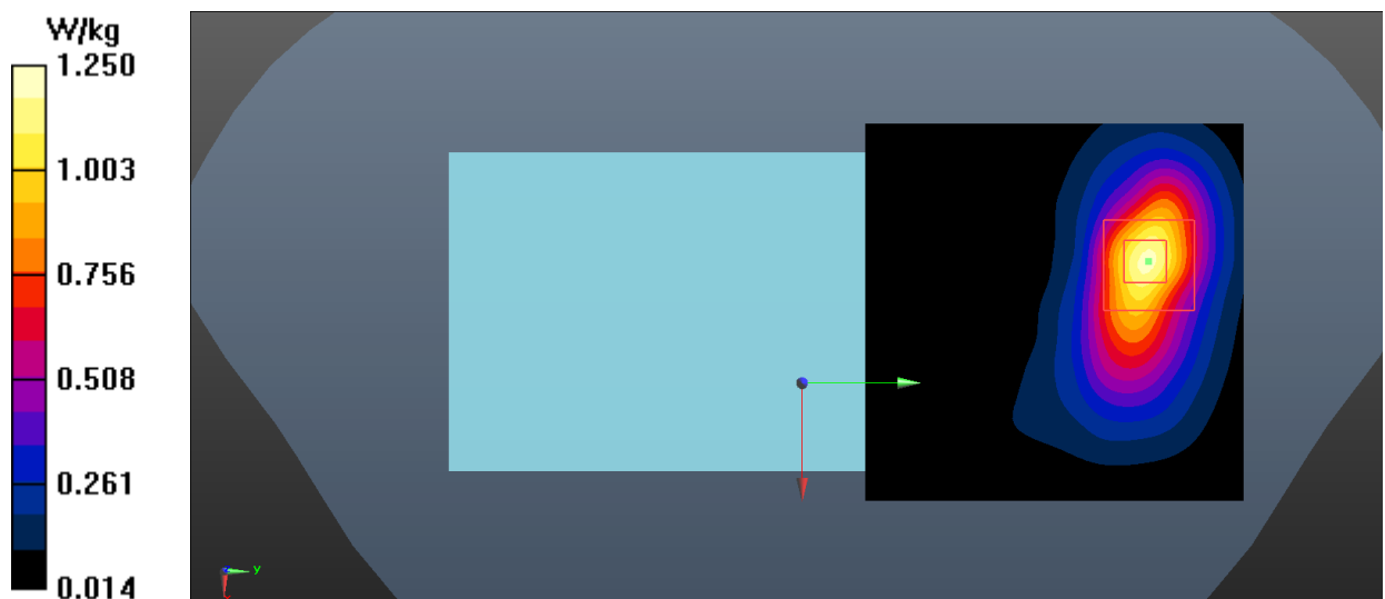
Fig.8 WCDMA Band 4 Body
