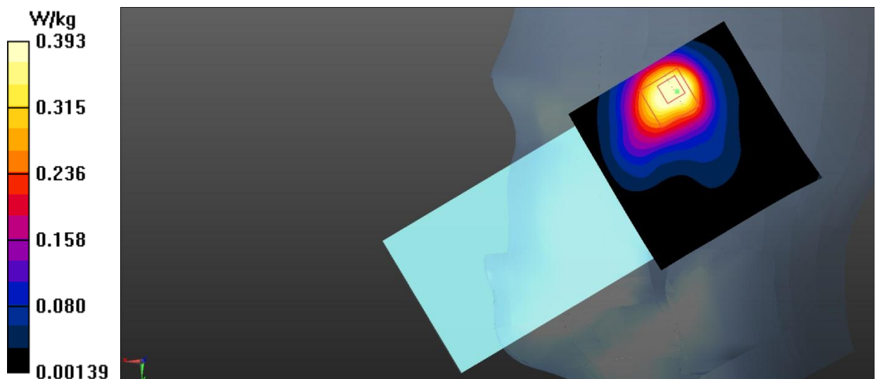
Fig.25 WLAN 2.4G Head
