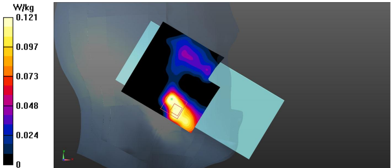
Fig.15 LTE Band 7 Head
