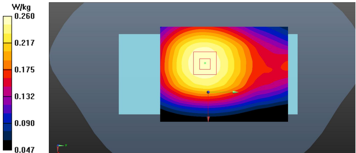
Fig.22 LTE Band 28 Body
