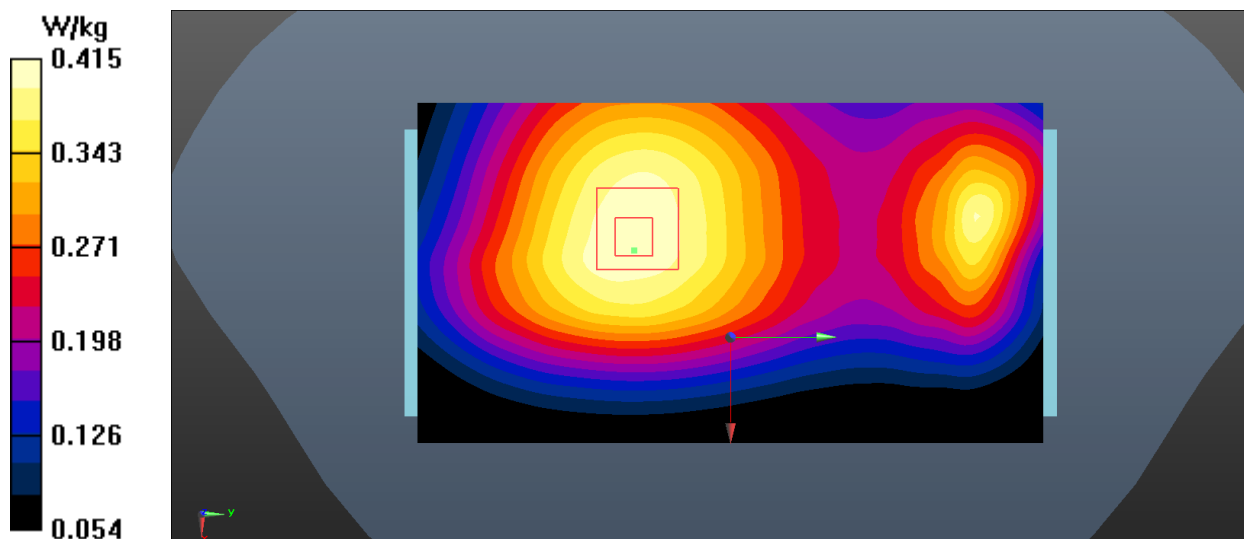
Fig.10 WCDMA Band 5 Body
