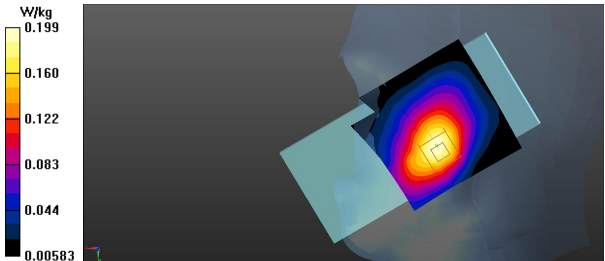
Fig.23 LTE Band 66 Head
