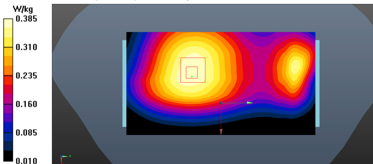
Fig.14 LTE Band 5 Body
