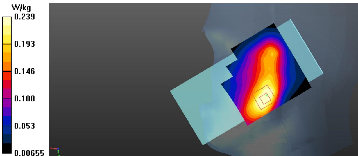
Fig.11 LTE Band 2 Head
