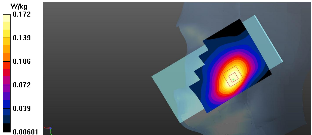
Fig.7 WCDMA Band 4 Head
