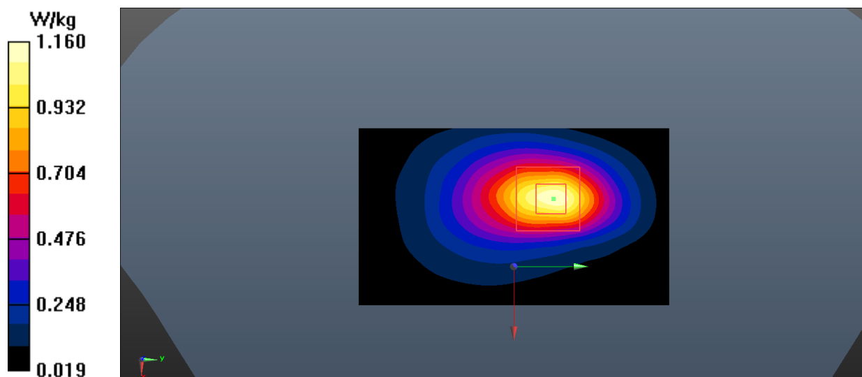
Fig.6 WCDMA Band 2 Body
