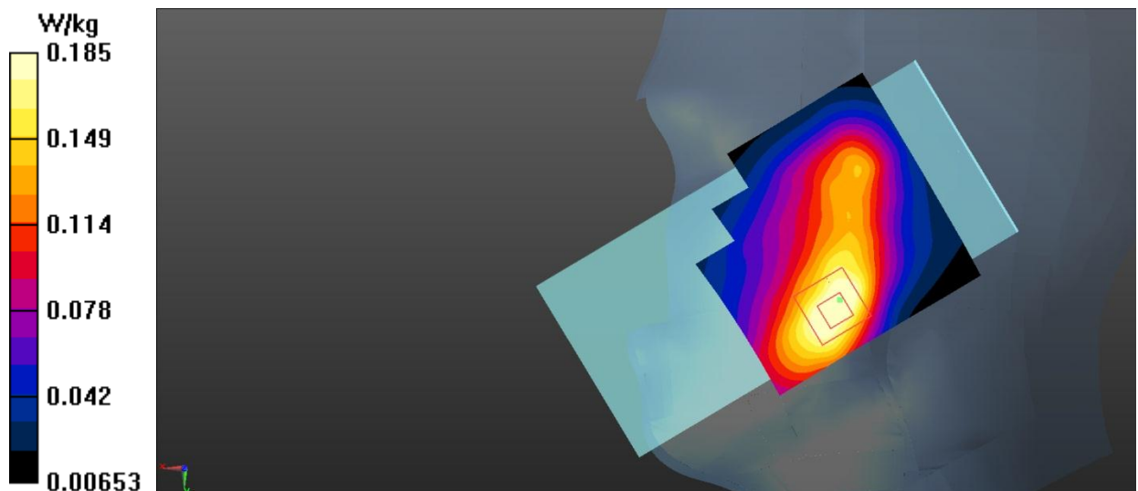
Fig.5 WCDMA Band 2 Head
