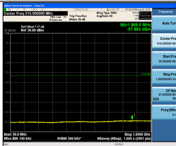
Band4_15MHz_QPSK_20175_1RB#0_30~1000_30~1000
