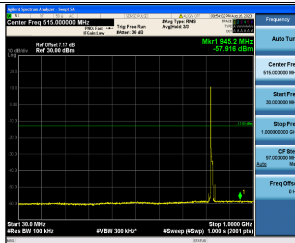
Band5_10MHz_QPSK_20450_1RB#0_30~1000_30~1000
