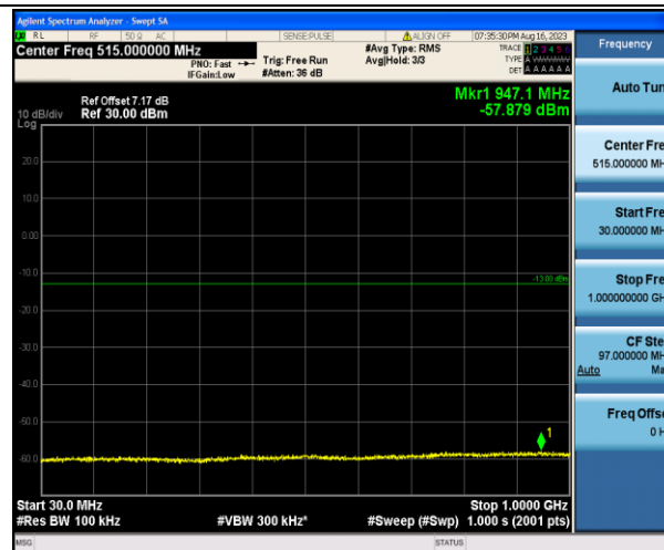
Band4_15MHz_QPSK_20025_1RB#0_30~1000_30~1000
