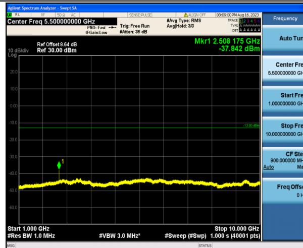
Band5_1.4MHz_QPSK_20525_1RB#0_1000~10000_1000~10000
