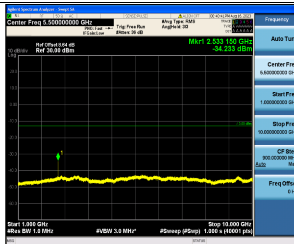
Band5_5MHz_QPSK_20625_1RB#0_1000~10000_1000~10000
