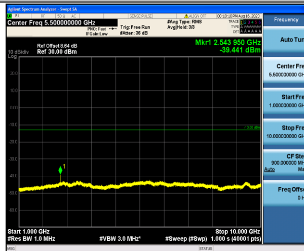
Band5_1.4MHz_16QAM_20643_1RB#0_1000~10000_1000~10000
