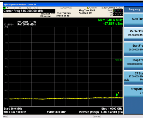
Band4_10MHz_16QAM_20350_1RB#0_30~1000_30~1000
