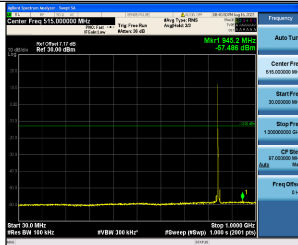
Band5_5MHz_16QAM_20625_1RB#0_30~1000_30~1000
