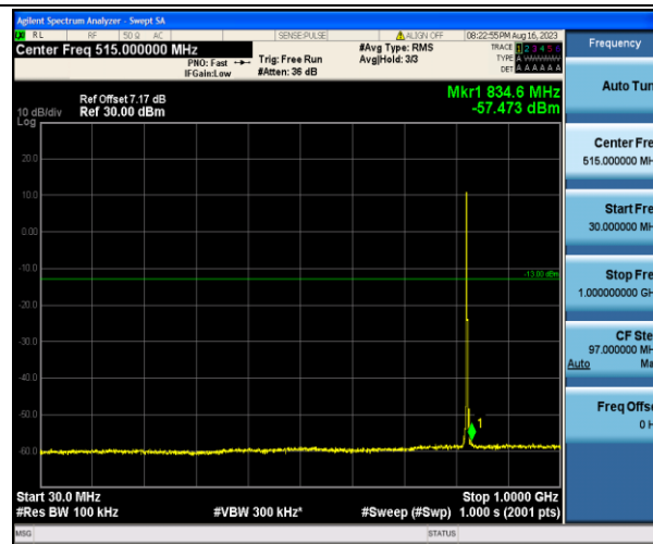
Band5_3MHz_QPSK_20415_1RB#0_30~1000_30~1000
