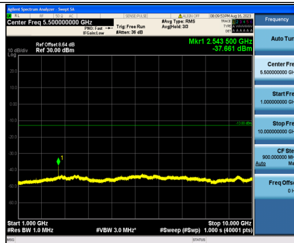
Band5_1.4MHz_QPSK_20643_1RB#0_1000~10000_1000~10000
