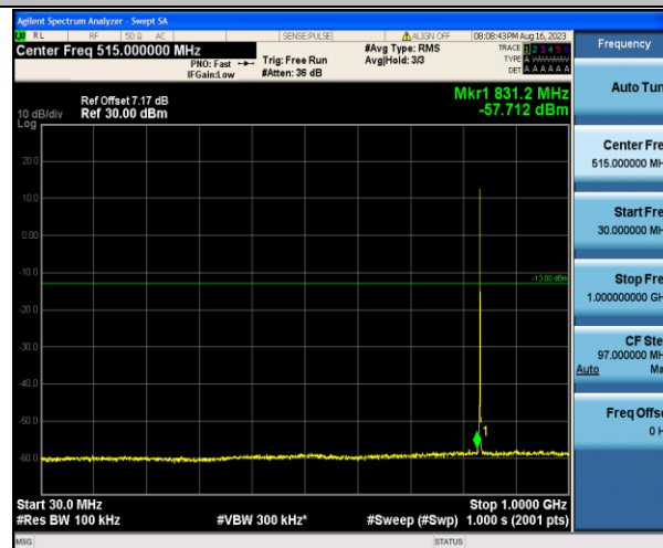
Band5_1.4MHz_QPSK_20525_1RB#0_30~1000_30~1000
