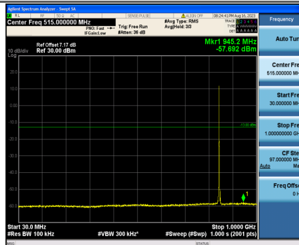
Band5_3MHz_QPSK_20635_1RB#0_30~1000_30~1000
