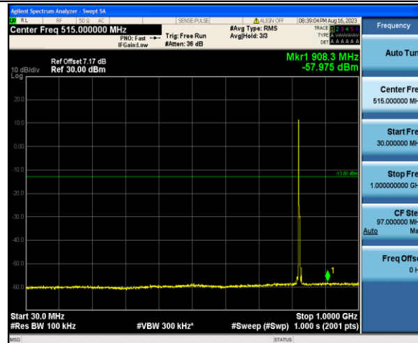
Band5_5MHz_16QAM_20425_1RB#0_30~1000_30~1000
