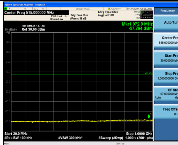
Band4_15MHz_QPSK_20325_1RB#0_30~1000_30~1000
