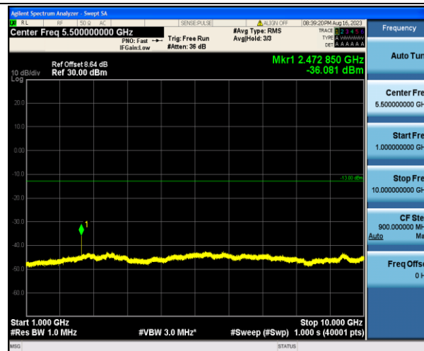
Band5_5MHz_16QAM_20425_1RB#0_1000~10000_1000~10000
