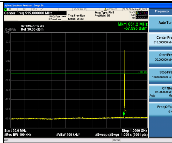
Band5_1.4MHz_16QAM_20525_1RB#0_30~1000_30~1000
