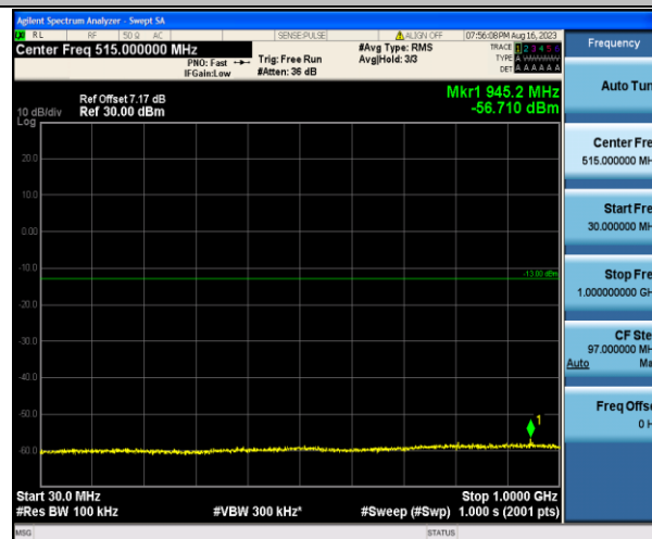
Band4_20MHz_16QAM_20300_1RB#0_30~1000_30~1000
