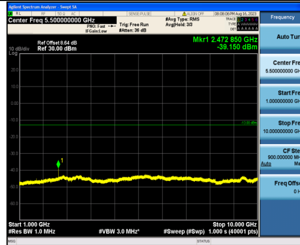
Band5_1.4MHz_QPSK_20407_1RB#0_1000~10000_1000~10000
