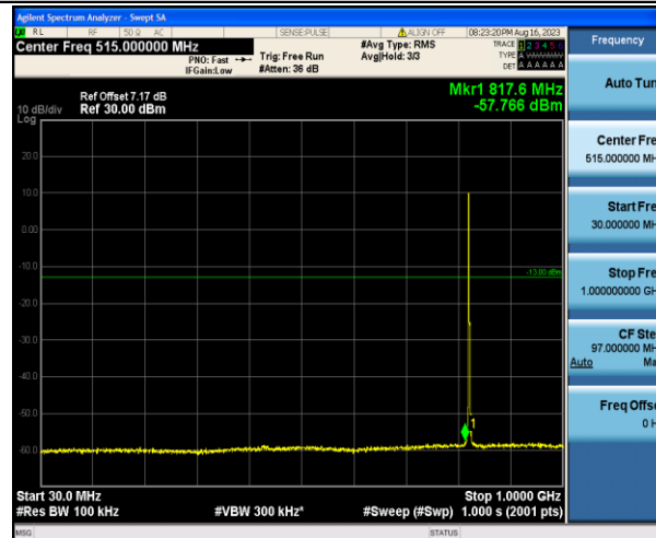
Band5_3MHz_16QAM_20415_1RB#0_30~1000_30~1000
