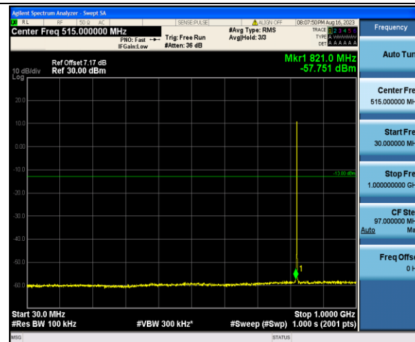
Band5_1.4MHz_QPSK_20407_1RB#0_30~1000_30~1000
