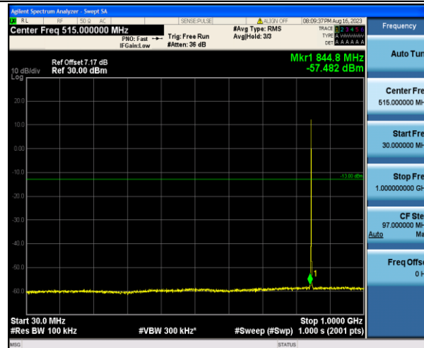
Band5_1.4MHz_QPSK_20643_1RB#0_30~1000_30~1000
