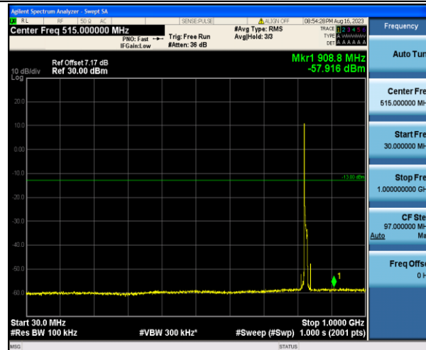
Band5_10MHz_16QAM_20450_1RB#0_30~1000_30~1000
