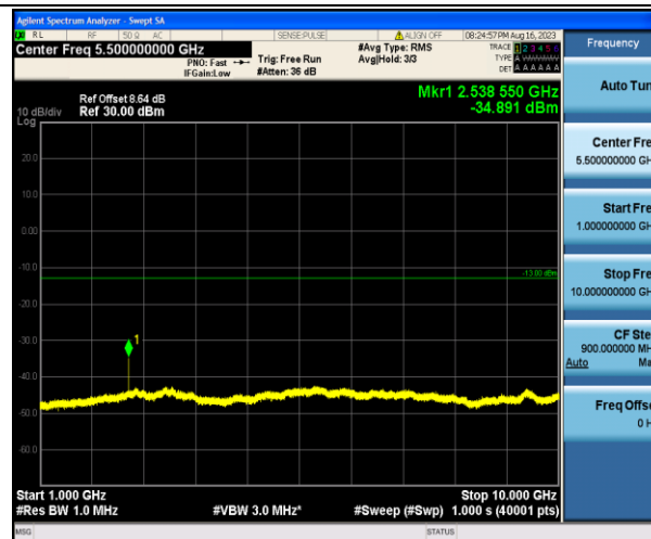
Band5_3MHz_QPSK_20635_1RB#0_1000~10000_1000~10000
