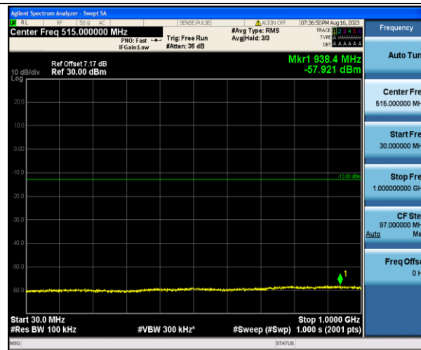
Band4_15MHz_16QAM_20175_1RB#0_30~1000_30~1000
