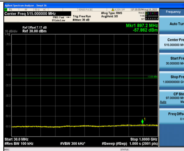
Band4_15MHz_16QAM_20025_1RB#0_30~1000_30~1000
