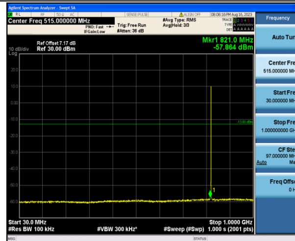
Band5_1.4MHz_16QAM_20407_1RB#0_30~1000_30~1000
