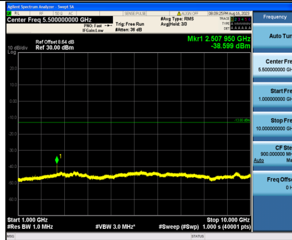
Band5_1.4MHz_16QAM_20525_1RB#0_1000~10000_1000~10000
