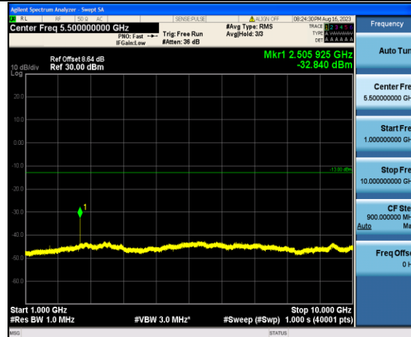
Band5_3MHz_16QAM_20525_1RB#0_1000~10000_1000~10000
