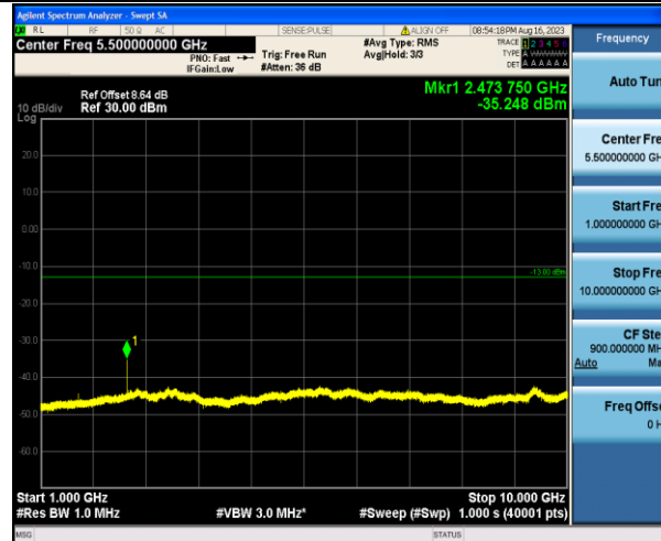
Band5_10MHz_QPSK_20450_1RB#0_1000~10000_1000~10000
