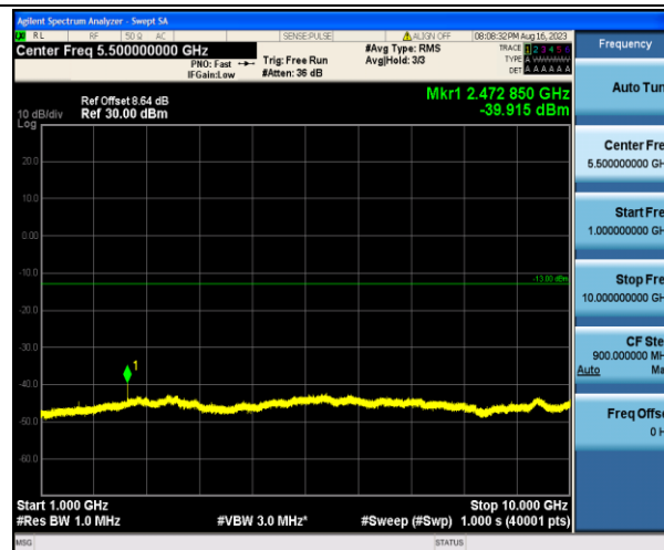
Band5_1.4MHz_16QAM_20407_1RB#0_1000~10000_1000~10000
