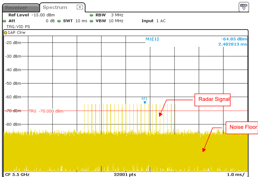
Radar Signal 2
