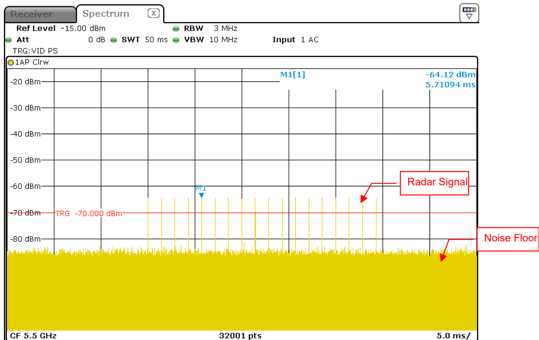
Radar Signal 0
