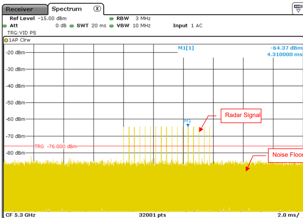
Radar Signal 3
