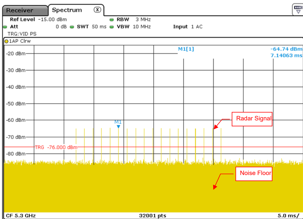
Radar Signal 0
