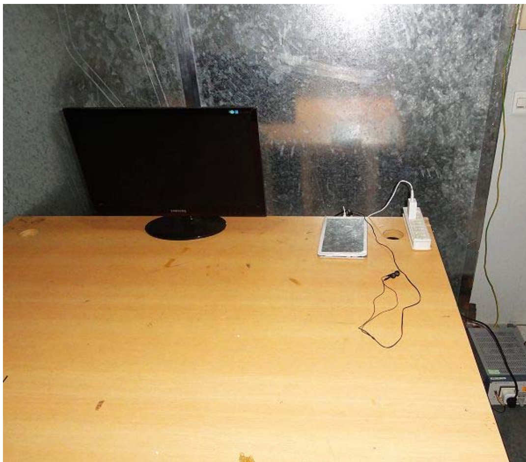
Conducted Emission Test Setup:
