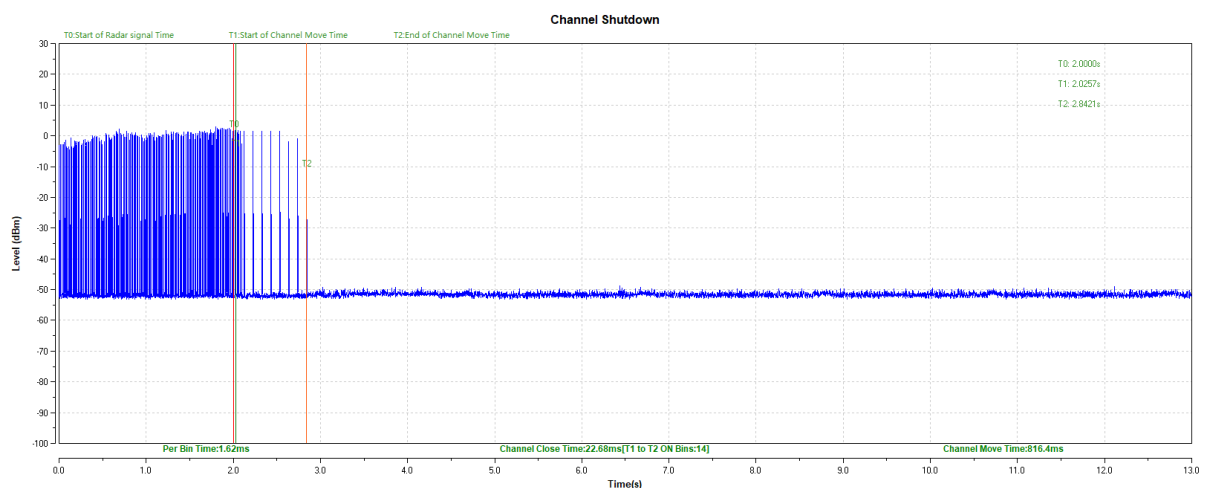
Fig.2 Channel Shutdown (HT80 Frequency Band: 5250MHz ~ 5350MHz)
