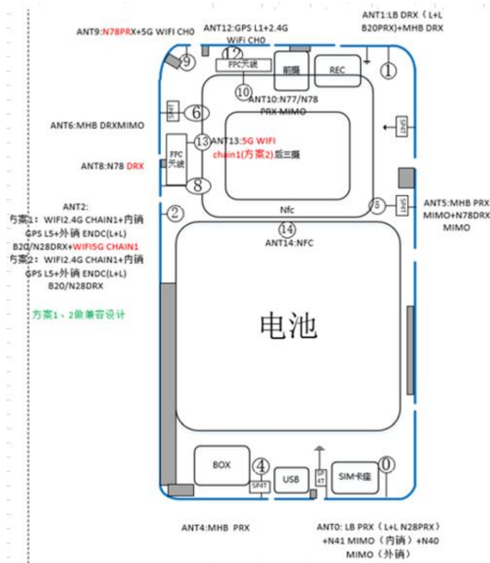
Fig 1 Antenna location & dimension
