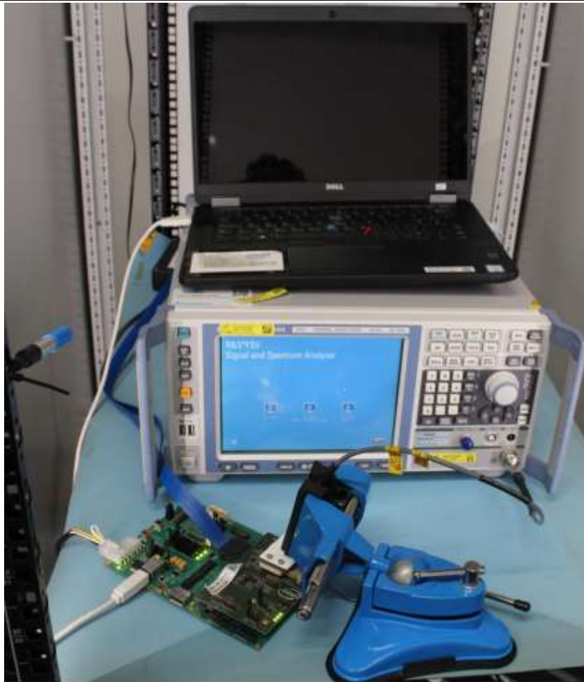
Conducted Setup
