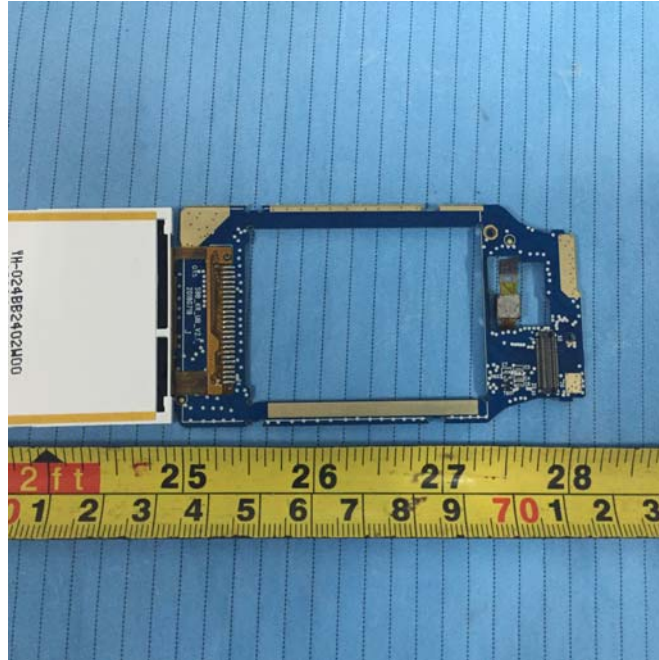
EUT – LCD Board Top View 2
