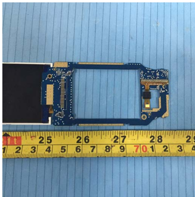
EUT – LCD Board Bottom View
