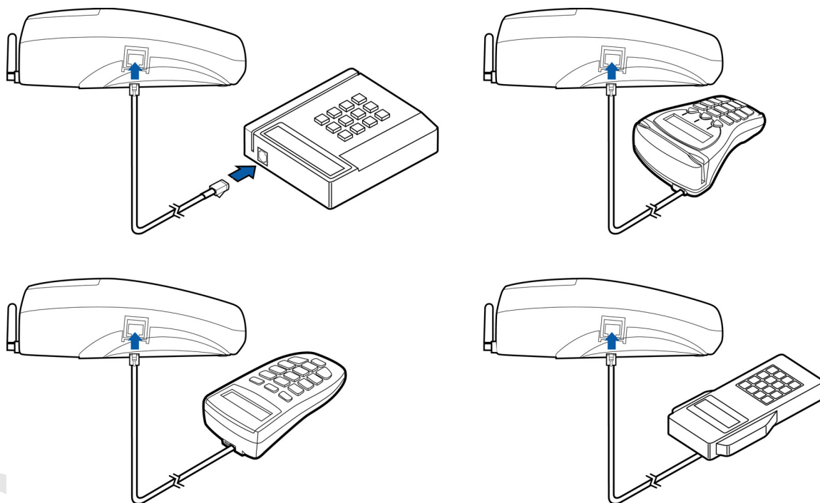
Figure 14 Vx670 Example Smart Card Reader Connection
