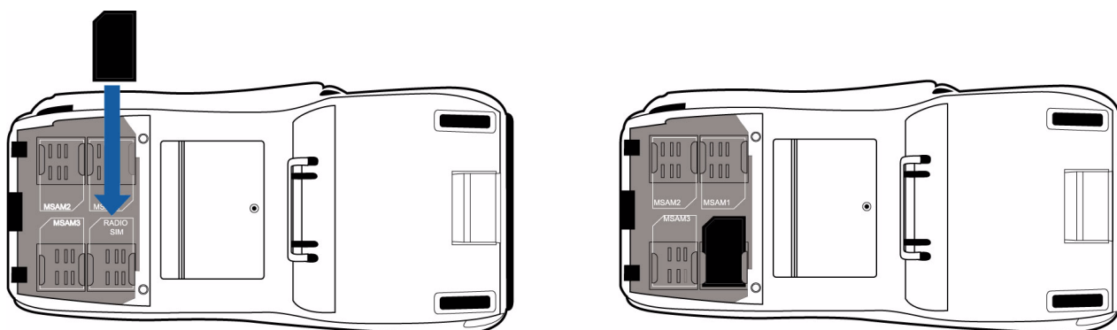
Figure 13 Inserting SIM Card
