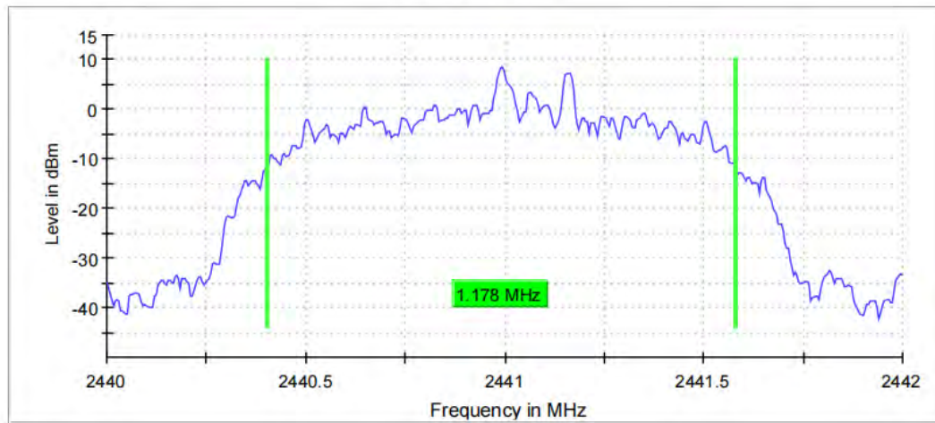
20 dB Bandwidth
