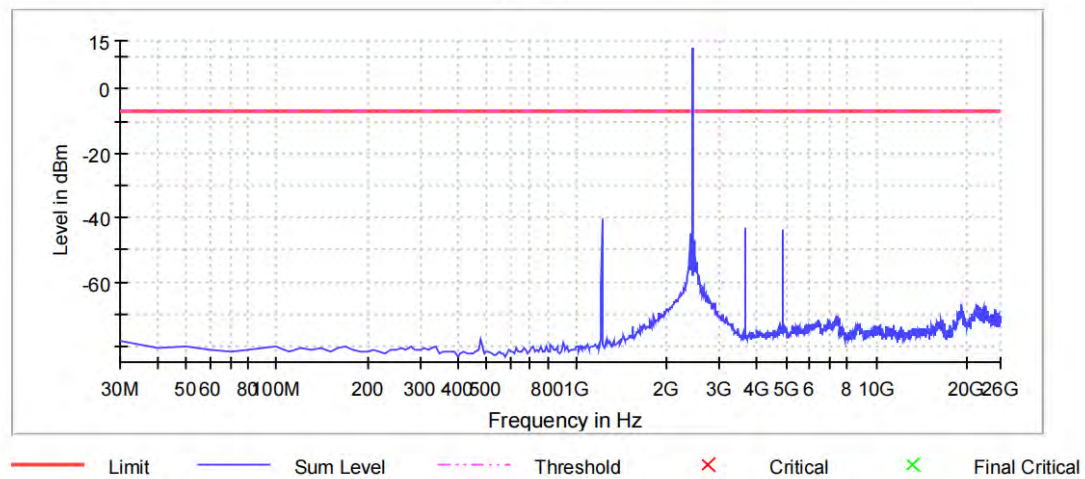
Spurious
