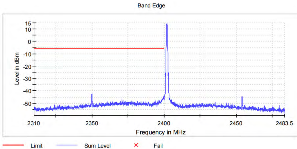
3DH5_Ant1_Low_2402
