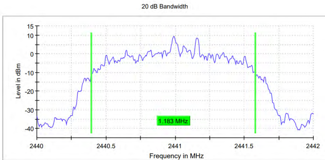
2DH5_Ant1_2441
