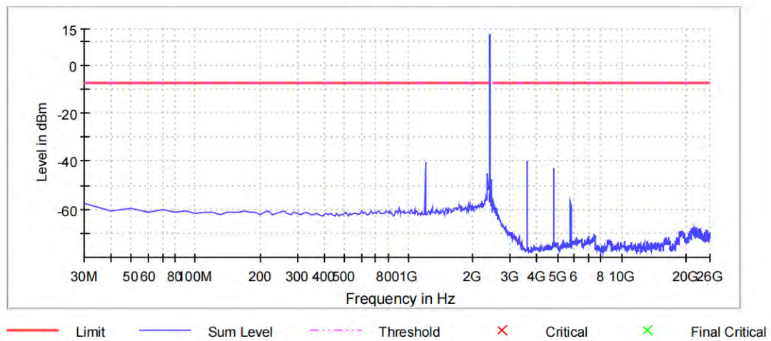
Spurious
