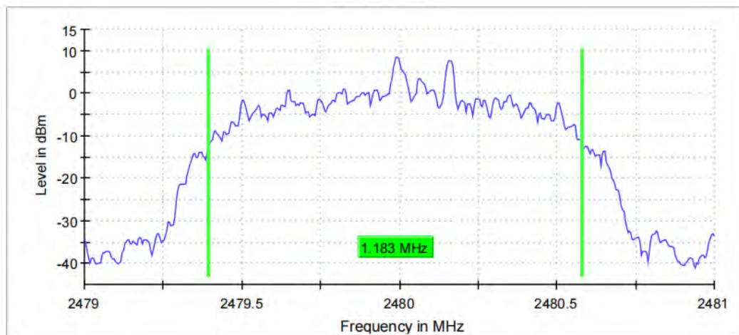
20 dB Bandwidth
