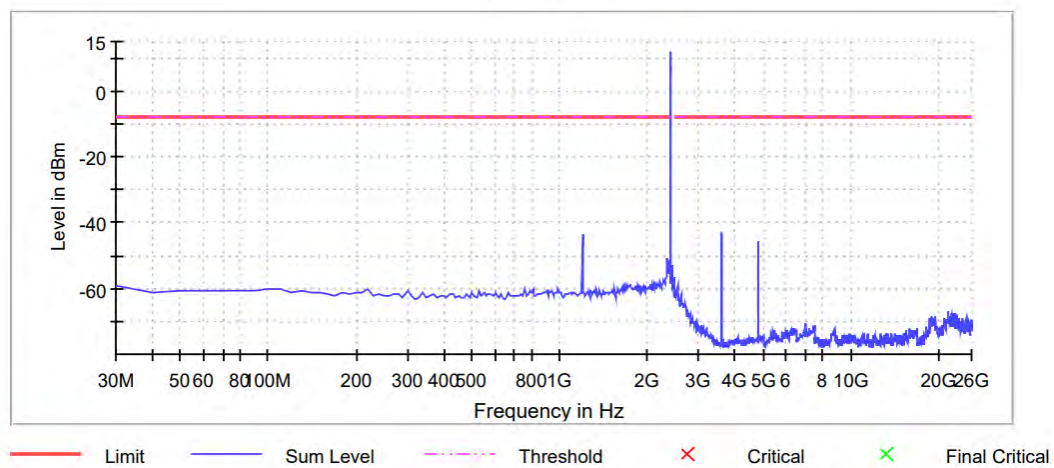
2DH5_Ant1_2402_30~26000
