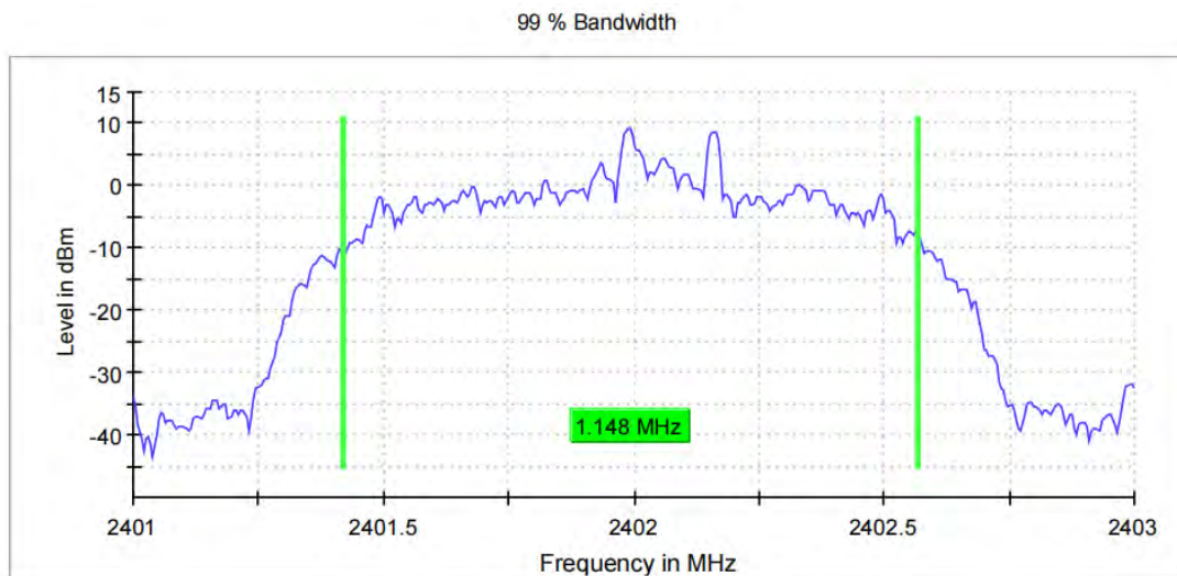
3DH5_Ant1_2402
