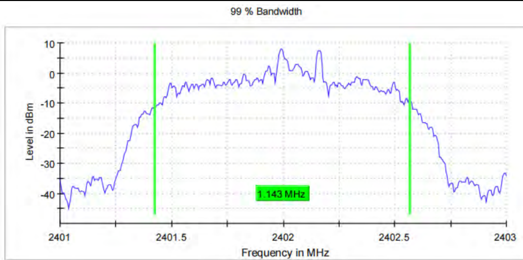
3DH5_Ant1_2402
