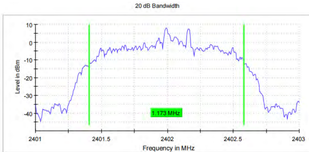
3DH5_Ant1_2402
