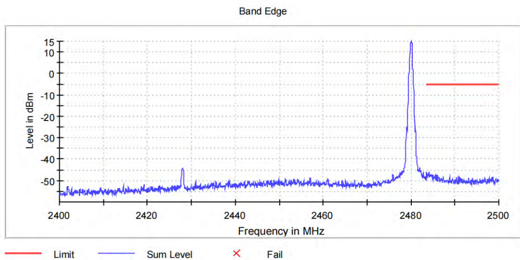
3DH5_Ant1_High_2480
