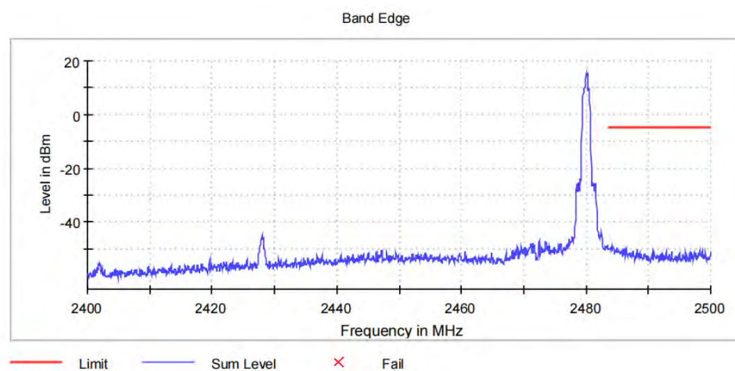
DH5_Ant1_High_2480
