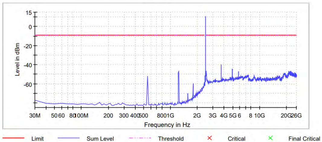
Spurious
