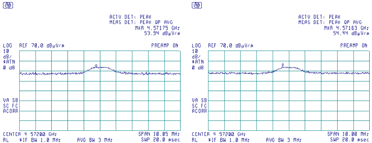
Plot 7.7.29 Radiated emission measurements at the fifth harmonic of high carrier frequency
