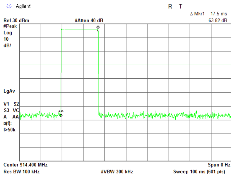
Plot 7.7.38 Transmission pulse duration
