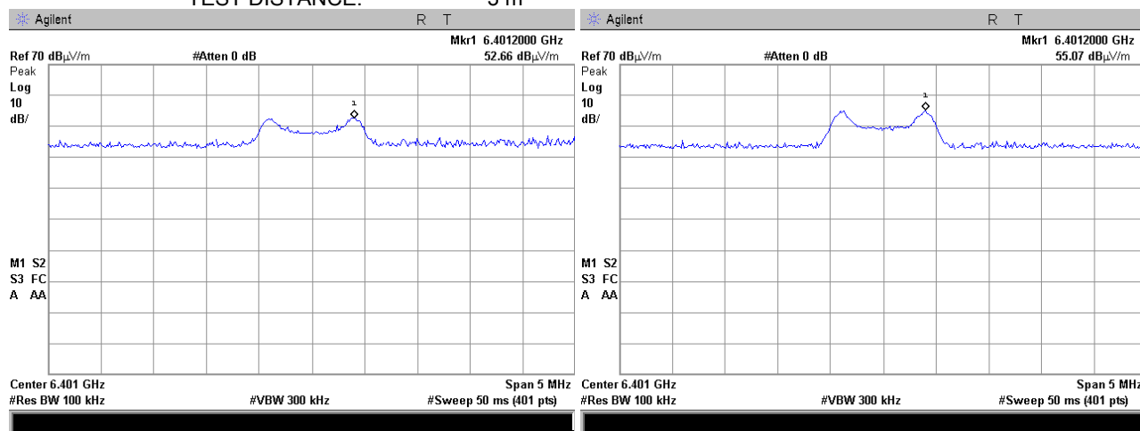
Plot 7.7.35 Radiated emission measurements at the seventh harmonic of high carrier frequency
