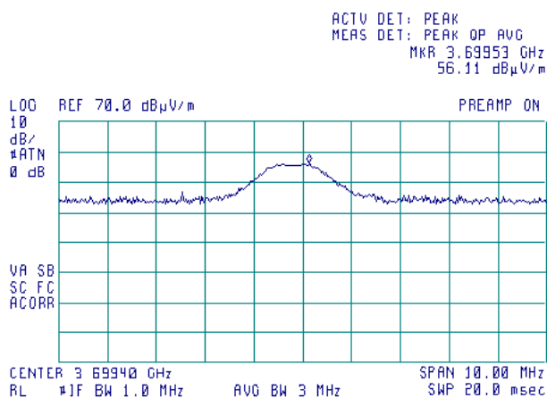
Plot 7.7.27 Radiated emission measurements at the fifth harmonic of low carrier frequency
