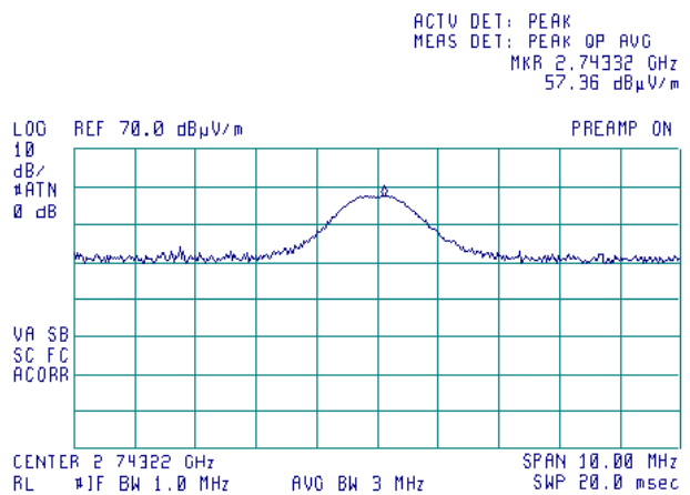
Plot 7.7.23 Radiated emission measurements at the third harmonic of high carrier frequency
