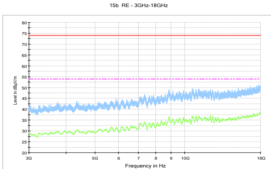
Figure A.9 Radiated Emission from 3GHz to 18GHz
