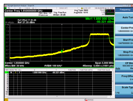
B2-20M-Low CH-BE-QPSK-Full RB 0
