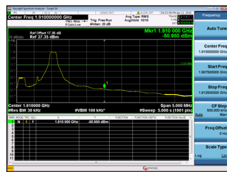
B2-20M-High CH-BE-QPSK-1 RB MAX
