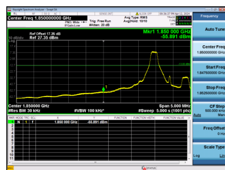
B2-20M-Low CH-BE-QPSK-1 RB 0
