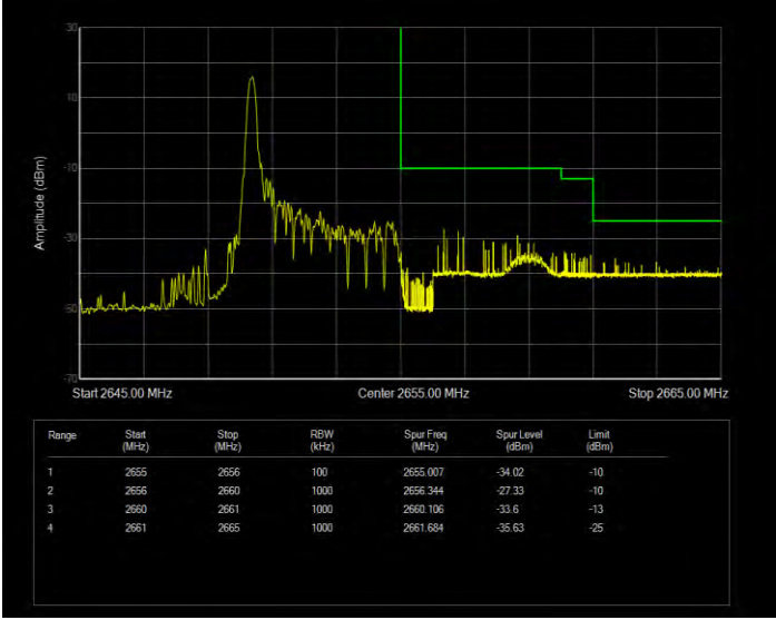
Band41(2535-2655) QPSK BW=5MHz Channel=41215 RB Size=1 Position=#Max Extended
