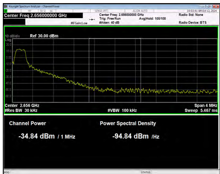
Band41(2535-2655) 16QAM BW=15MHz Channel=41165 RB Size=1 Position=#Max Normal
