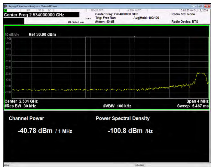
Band41(2535-2655) 16QAM BW=15MHz Channel=40115 RB Size=1 Position=#Max Normal
