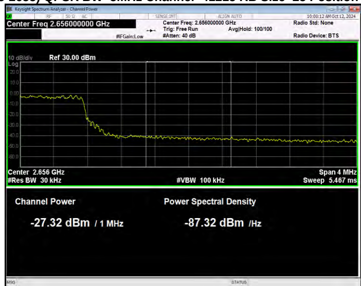
Band41(2535-2655) QPSK BW=5MHz Channel=41215 RB Size=25 Position=#0 Normal
