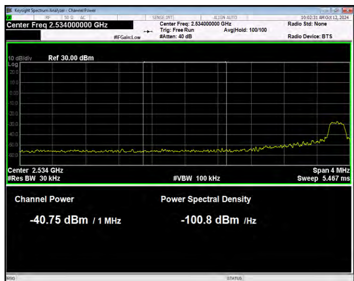
Band41(2535-2655) QPSK BW=15MHz Channel=40115 RB Size=1 Position=#Max Normal
