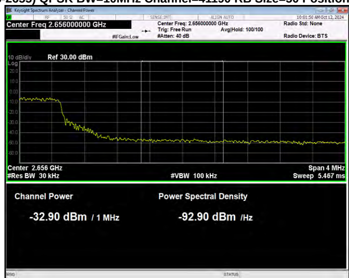
Band41(2535-2655) QPSK BW=10MHz Channel=41190 RB Size=50 Position=#0 Normal
