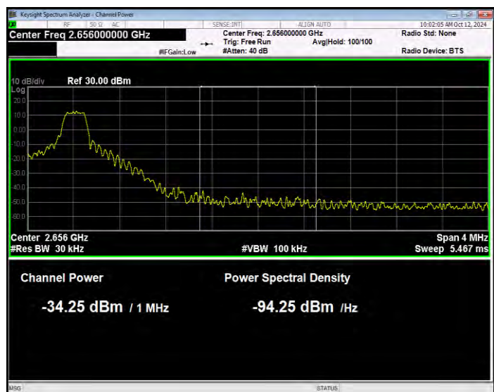
Band41(2535-2655) 16QAM BW=10MHz Channel=41190 RB Size=1 Position=#Max Normal
