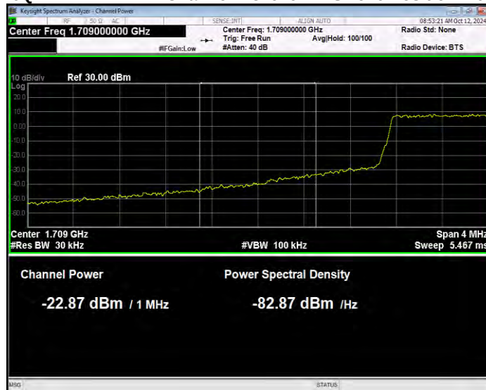
Band66 16QAM BW=1.4MHz Channel=131979 RB Size=6 Position=#0 Normal
