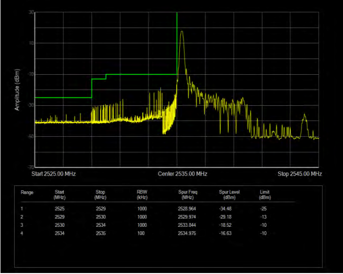
Band41(2535-2655) QPSK BW=5MHz Channel=40065 RB Size=1 Position=#Max Extended
