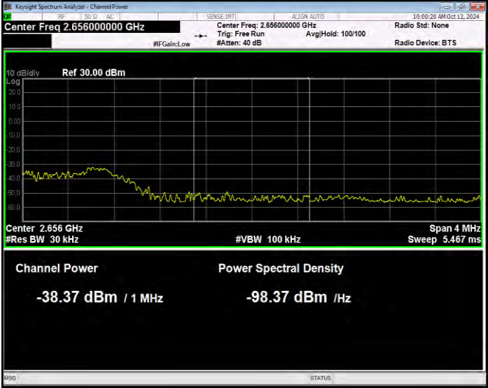
Band41(2535-2655) 16QAM BW=5MHz Channel=41215 RB Size=1 Position=#0 Normal
