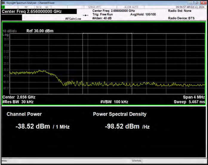
Band41(2535-2655) QPSK BW=5MHz Channel=41215 RB Size=1 Position=#0 Normal
