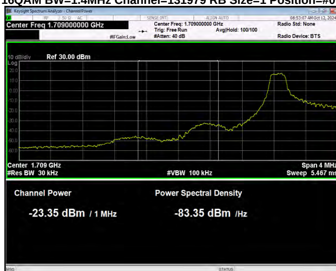
Band66 16QAM BW=1.4MHz Channel=131979 RB Size=1 Position=#0 Normal
