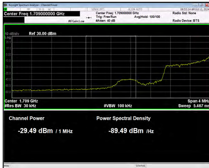
Band66 16QAM BW=1.4MHz Channel=131979 RB Size=1 Position=#Max Normal
