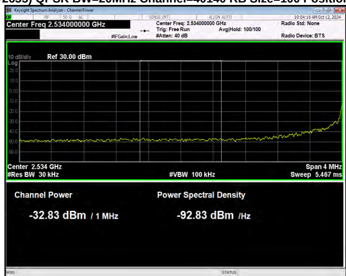
Band41(2535-2655) QPSK BW=20MHz Channel=40140 RB Size=100 Position=#0 Normal
