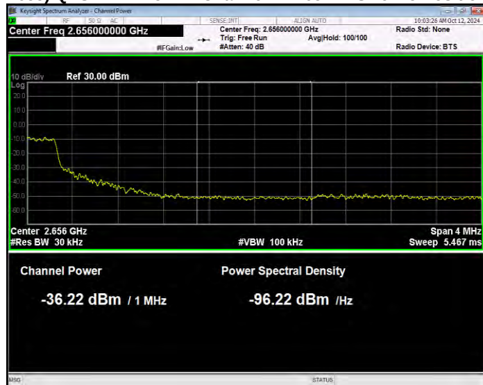
Band41(2535-2655) QPSK BW=15MHz Channel=41165 RB Size=75 Position=#0 Normal
