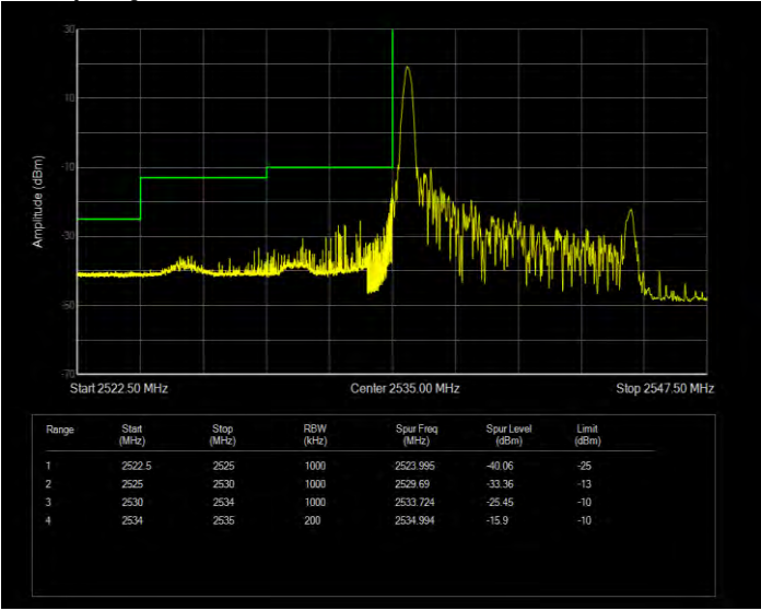
Band41(2535-2655) 16QAM BW=10MHz Channel=40090 RB Size=1 Position=#Max Extended
