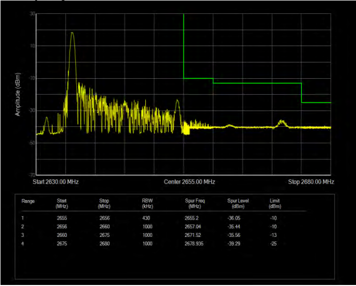
Band41(2535-2655) 16QAM BW=20MHz Channel=41140 RB Size=1 Position=#Max Extended
