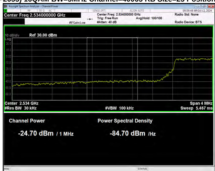
Band41(2535-2655) 16QAM BW=5MHz Channel=40065 RB Size=25 Position=#0 Normal
