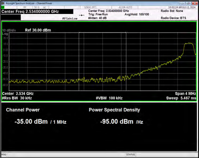
Band41(2535-2655) QPSK BW=15MHz Channel=40115 RB Size=1 Position=#0 Normal
