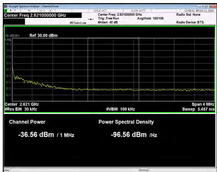
Band38 QPSK BW=20MHz Channel=38150 RB Size=100 Position=#0 Normal
