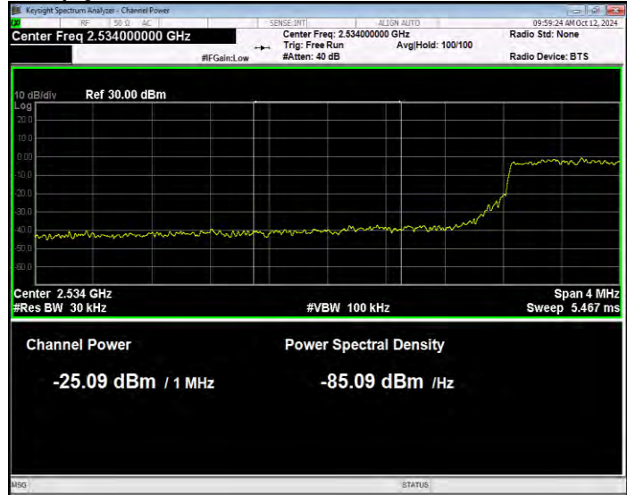
Band41(2535-2655) QPSK BW=5MHz Channel=40065 RB Size=25 Position=#0 Normal
