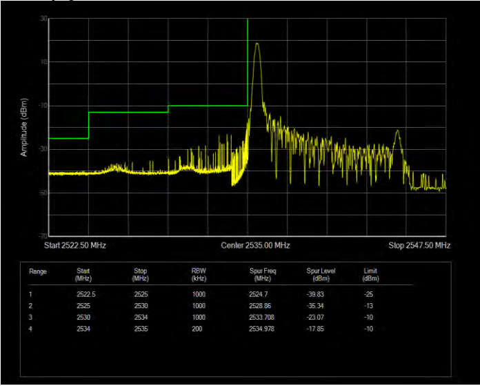
Band41(2535-2655) QPSK BW=10MHz Channel=40090 RB Size=1 Position=#Max Extended
