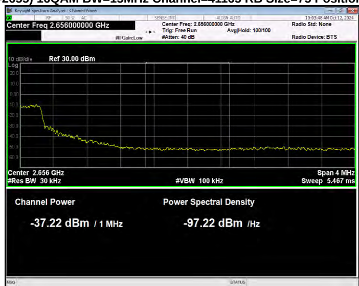
Band41(2535-2655) 16QAM BW=15MHz Channel=41165 RB Size=75 Position=#0 Normal
