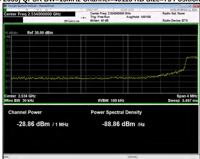
Band41(2535-2655) QPSK BW=15MHz Channel=40115 RB Size=75 Position=#0 Normal
