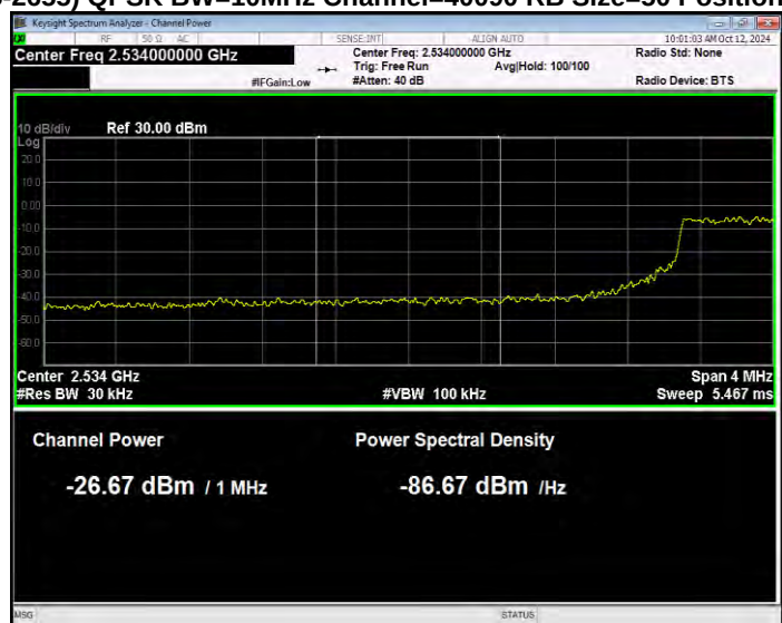
Band41(2535-2655) QPSK BW=10MHz Channel=40090 RB Size=50 Position=#0 Normal
