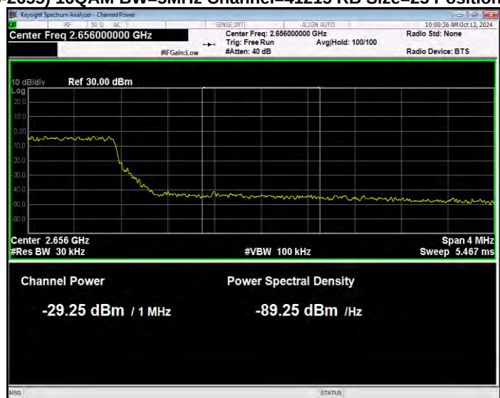
Band41(2535-2655) 16QAM BW=5MHz Channel=41215 RB Size=25 Position=#0 Normal
