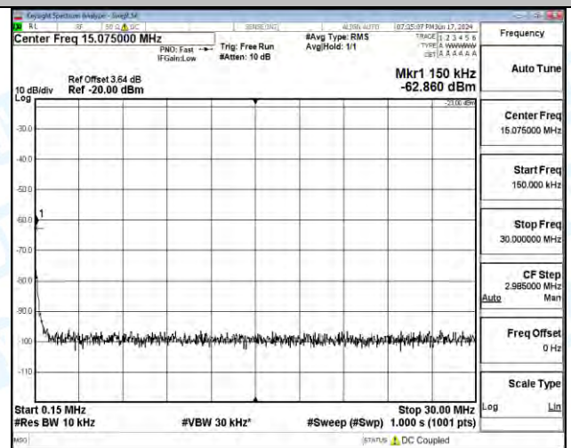
Band12_5MHz_QPSK_23155_25RB#0_1000~3000_1000~3000
