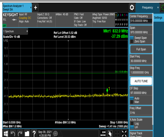
Band25-5MHz-QPSK-26665-1RB#0-Range3:30~1000MHz
