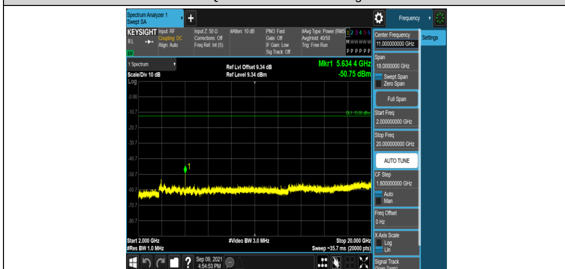
Band25-10MHz-16QAM-26365-1RB#0-Range5:2000~20000MHz
