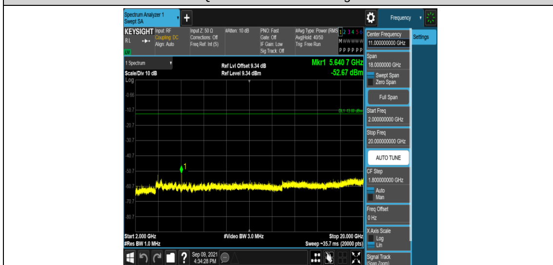
Band25-5MHz-16QAM-26365-1RB#0-Range5:2000~20000MHz
