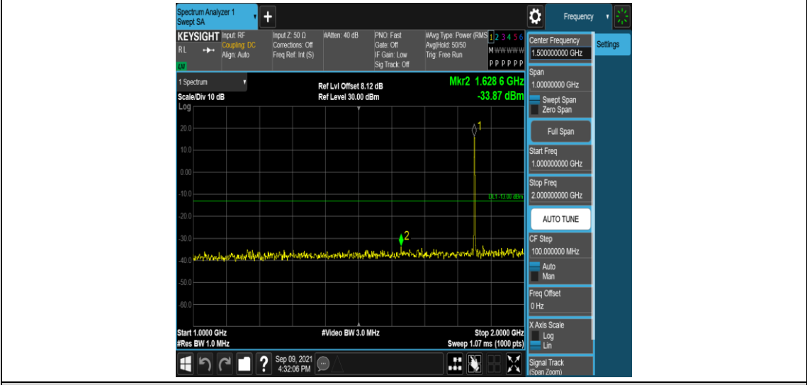
Band25-5MHz-16QAM-26065-1RB#0-Range4:1000~2000MHz
