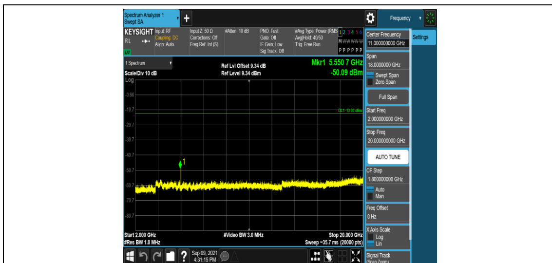
Band25-5MHz-QPSK-26065-1RB#0-Range5:2000~20000MHz
