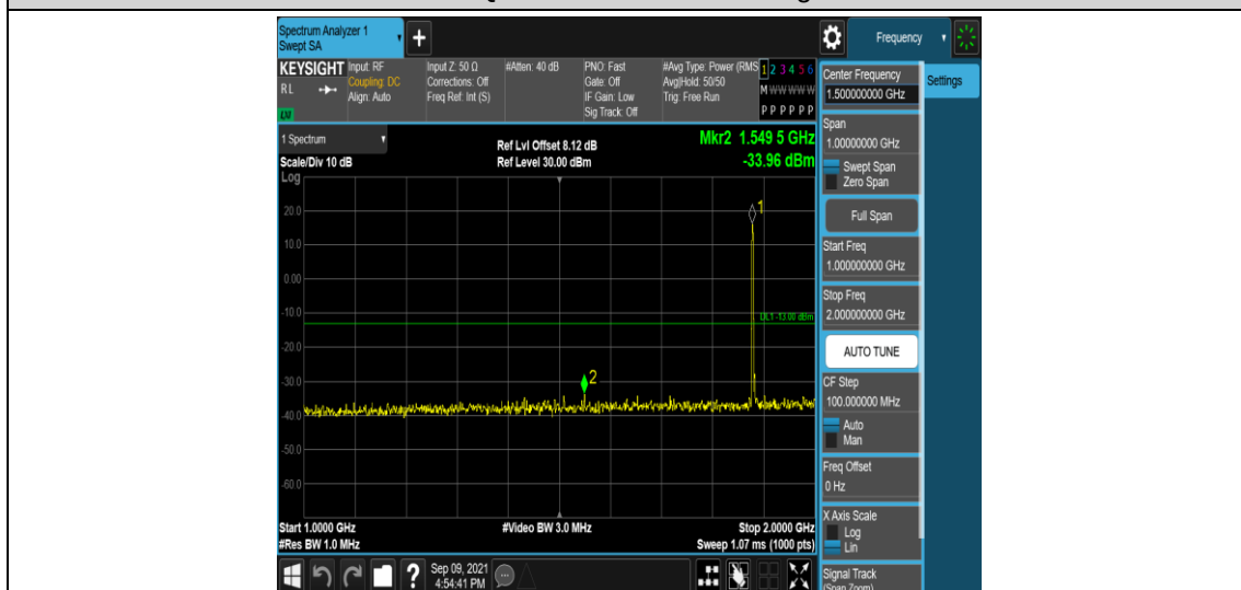
Band25-10MHz-16QAM-26365-1RB#0-Range4:1000~2000MHz
