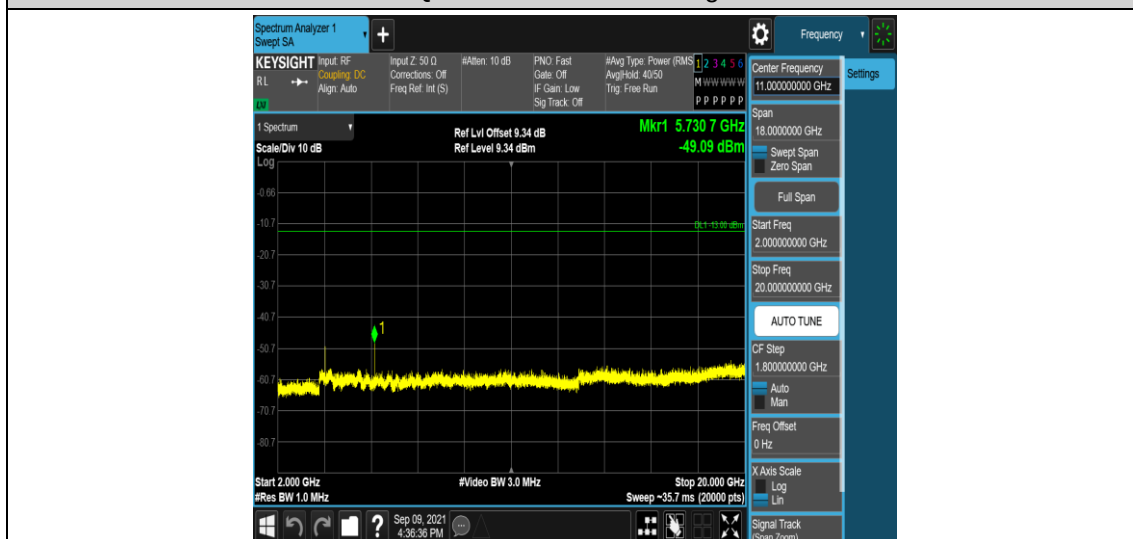
Band25-5MHz-16QAM-26665-1RB#0-Range5:2000~20000MHz
