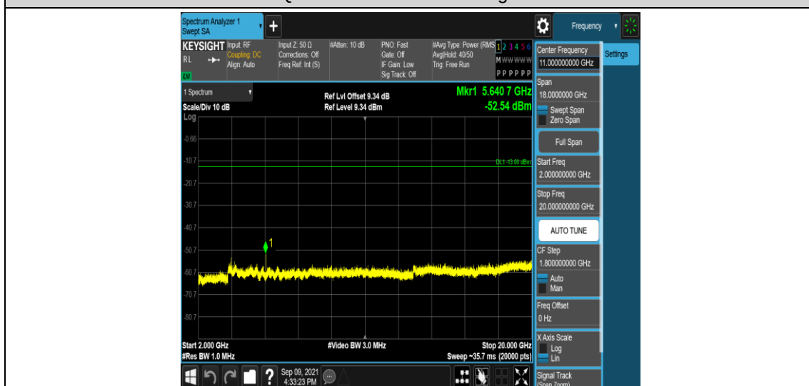
Band25-5MHz-QPSK-26365-1RB#0-Range5:2000~20000MHz
