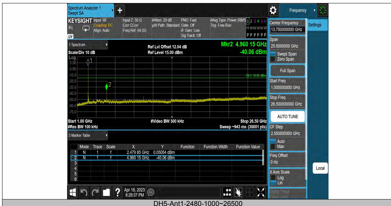
DH5-Ant1-2480-1000~26500
