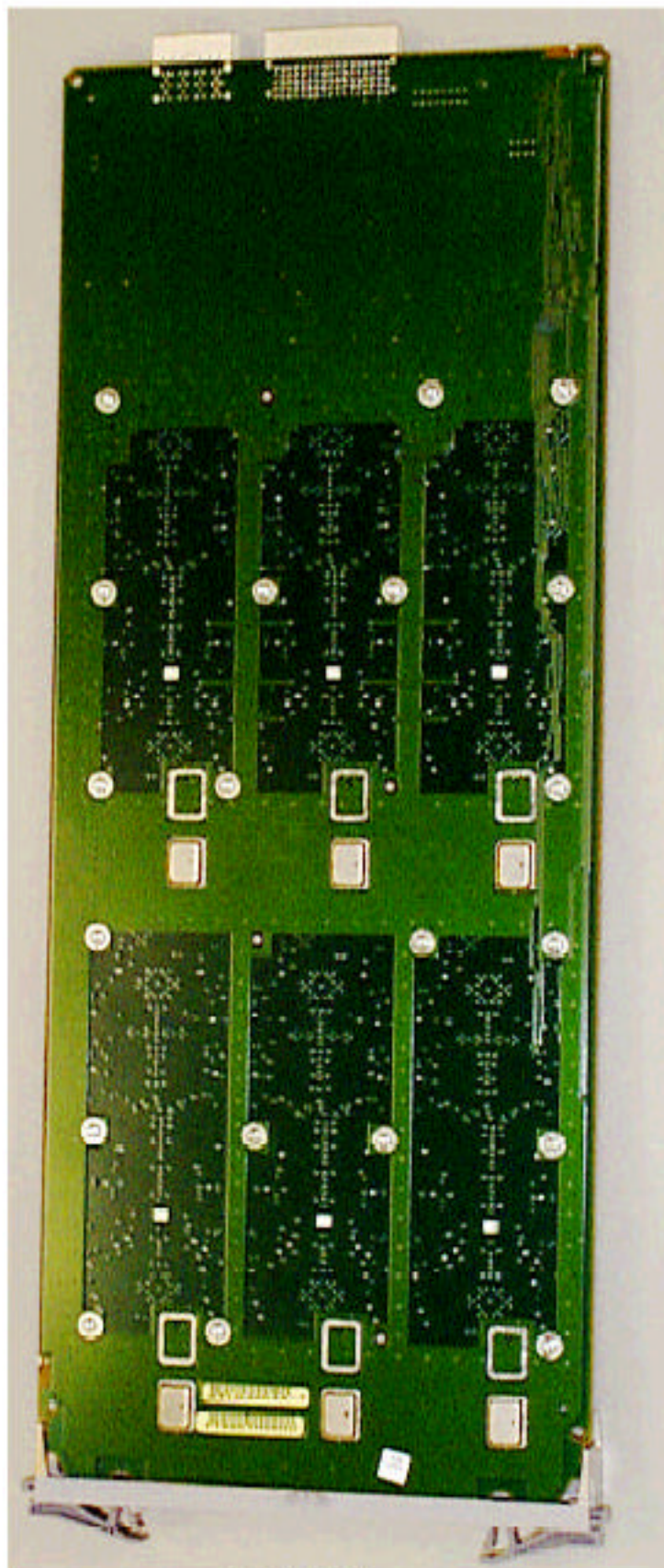
IHET5ZR1 SC4812ET 800 MHz MPC Back
