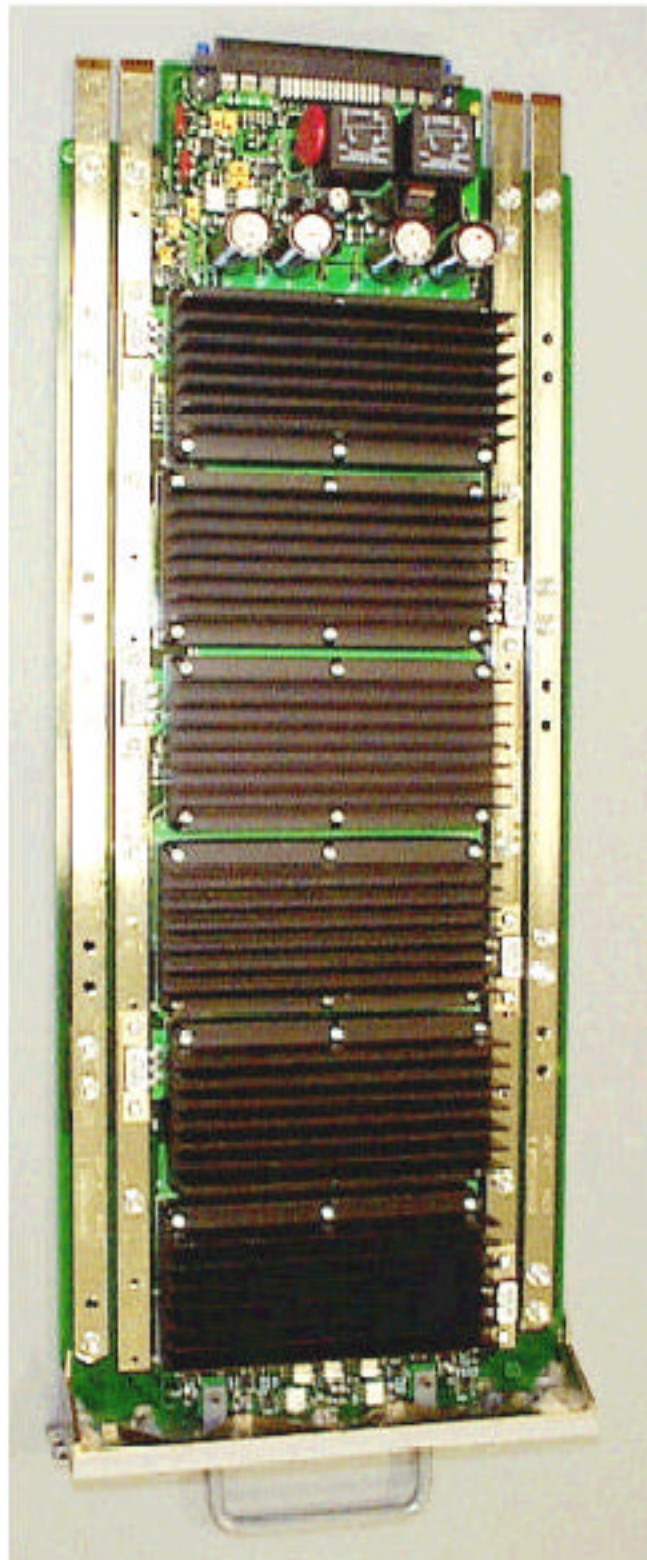
IHET5ZR1 SC4812ET 800 MHz Power Supply Front
