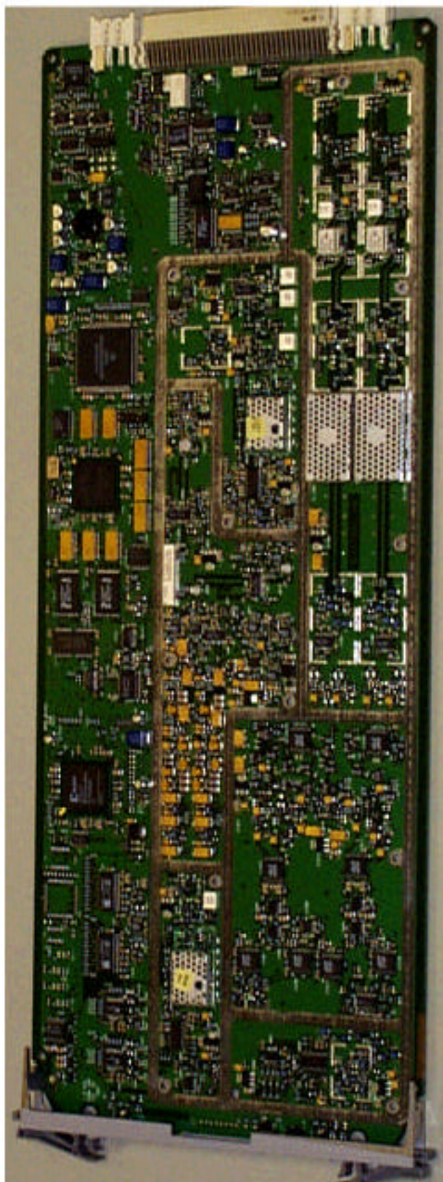
IHET5ZR1 SC4812ET 800 MHz BBX2 without Cover
