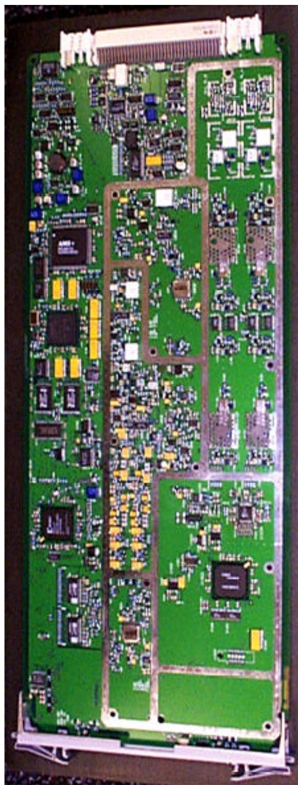
IHET5ZR1 SC4812ET 800 MHz DBPBBX Front without Cover
