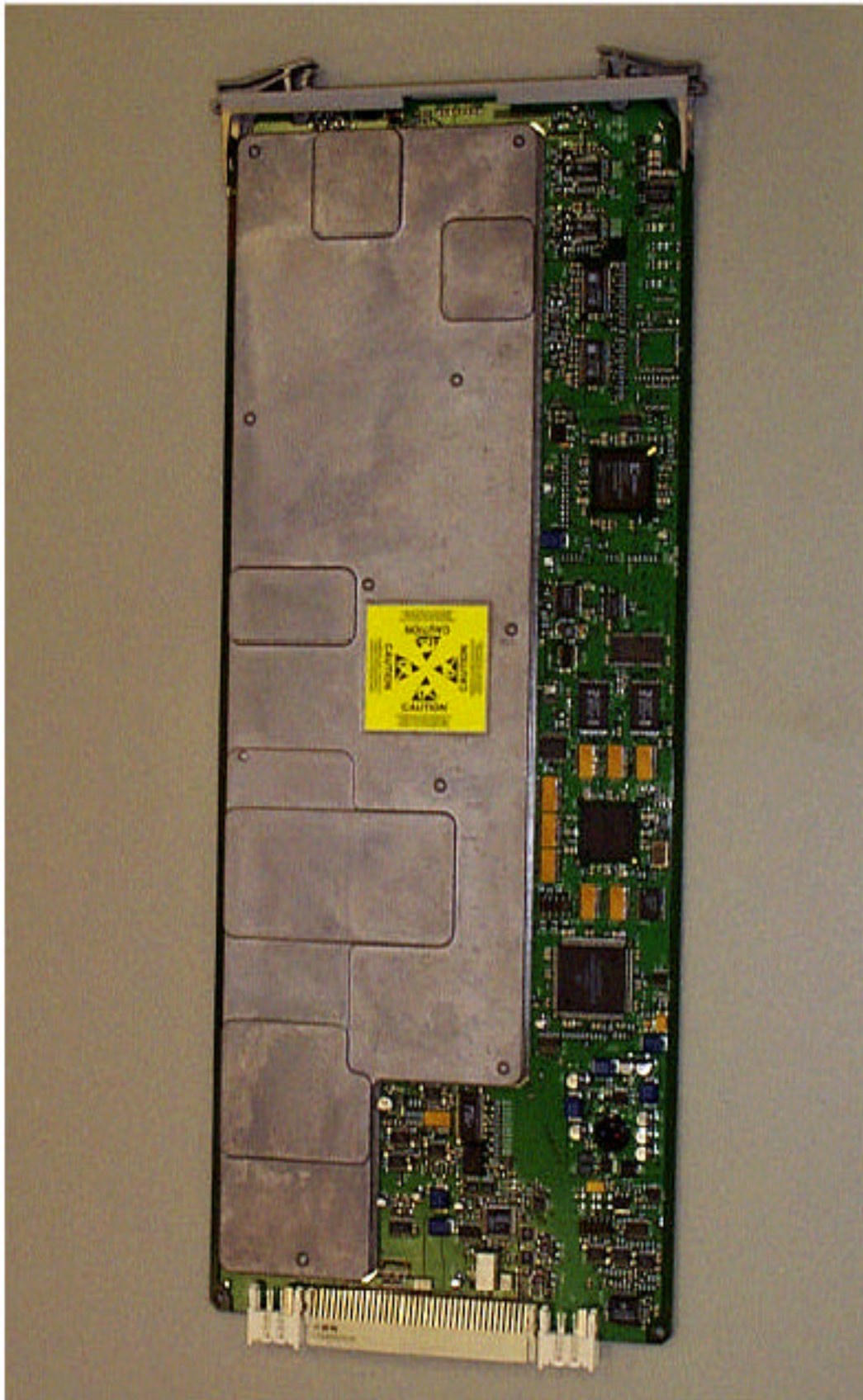
IHET5ZR1 SC4812ET 800 MHz BBX2 with Cover
