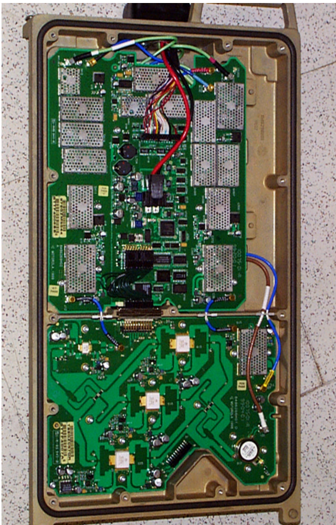
IHET5ZR1 SC4812ET 800 MHz LPA without Cover
