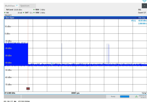
11AX160SISO-Ant1-6985-High-7058.7397-Minimal
