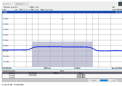
11AX160SISO-Ant1-6505-High-6578.5024-Minimal
