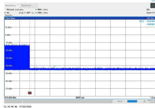
11AX160SISO-Ant1-6825-High-6898.7547-OFF-PASS
