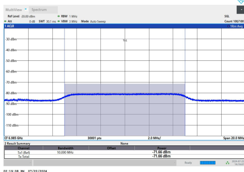
11AX160SISO-Ant1-6985-High-7058.7397-Minimal
