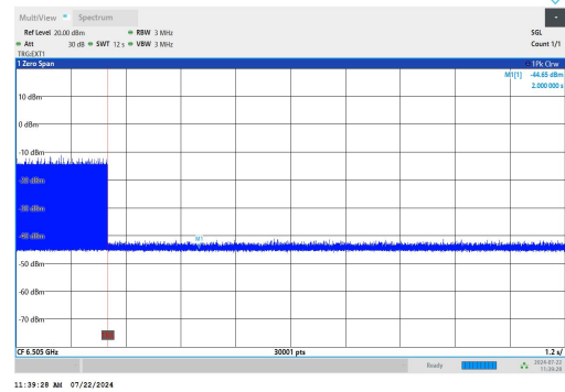
11AX160SISO-Ant1-6505-High-6578.5024-OFF-PASS
