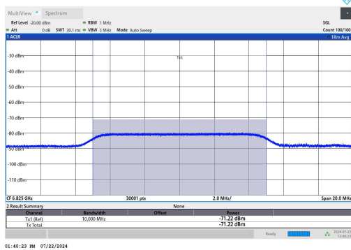
11AX160SISO-Ant1-6825-High-6898.7547-Minimal
