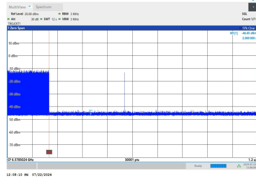
11AX160SISO-Ant1-6825-Low-6751.8896-OFF-PASS
