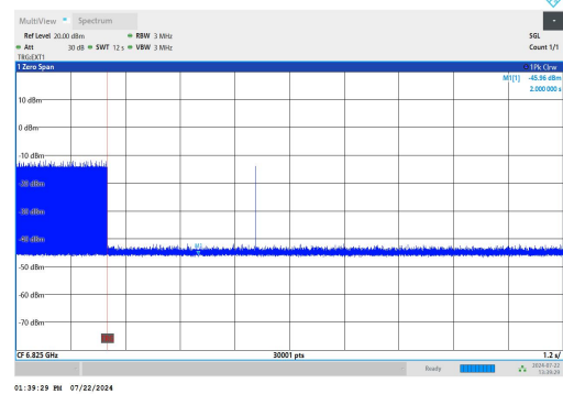
11AX160SISO-Ant1-6825-High-6898.7547-Minimal
