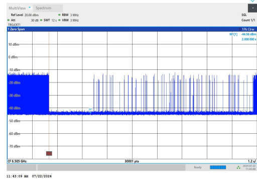
11AX160SISO-Ant1-6505-High-6578.5024-Minimal
