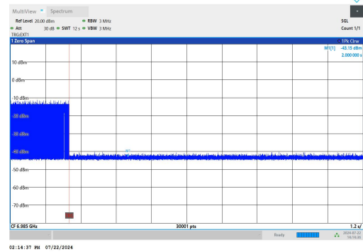
11AX160SISO-Ant1-6985-High-7058.7397-OFF-PASS
