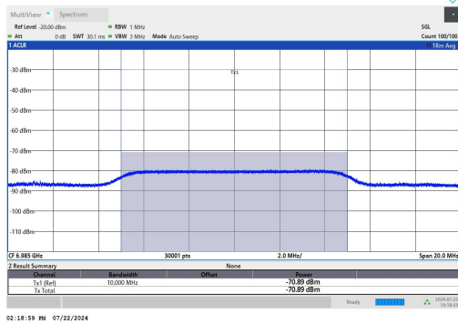
11AX160SISO-Ant1-6985-High-7058.7397-OFF-PASS
