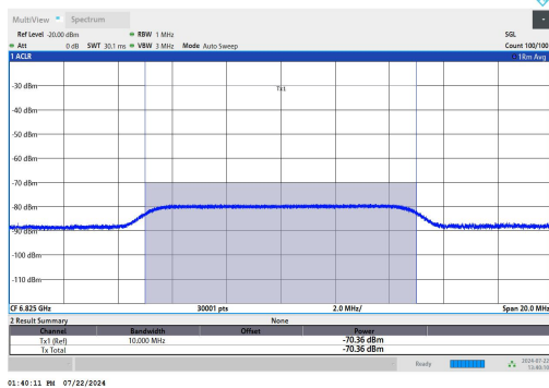
11AX160SISO-Ant1-6825-High-6898.7547-OFF-PASS
