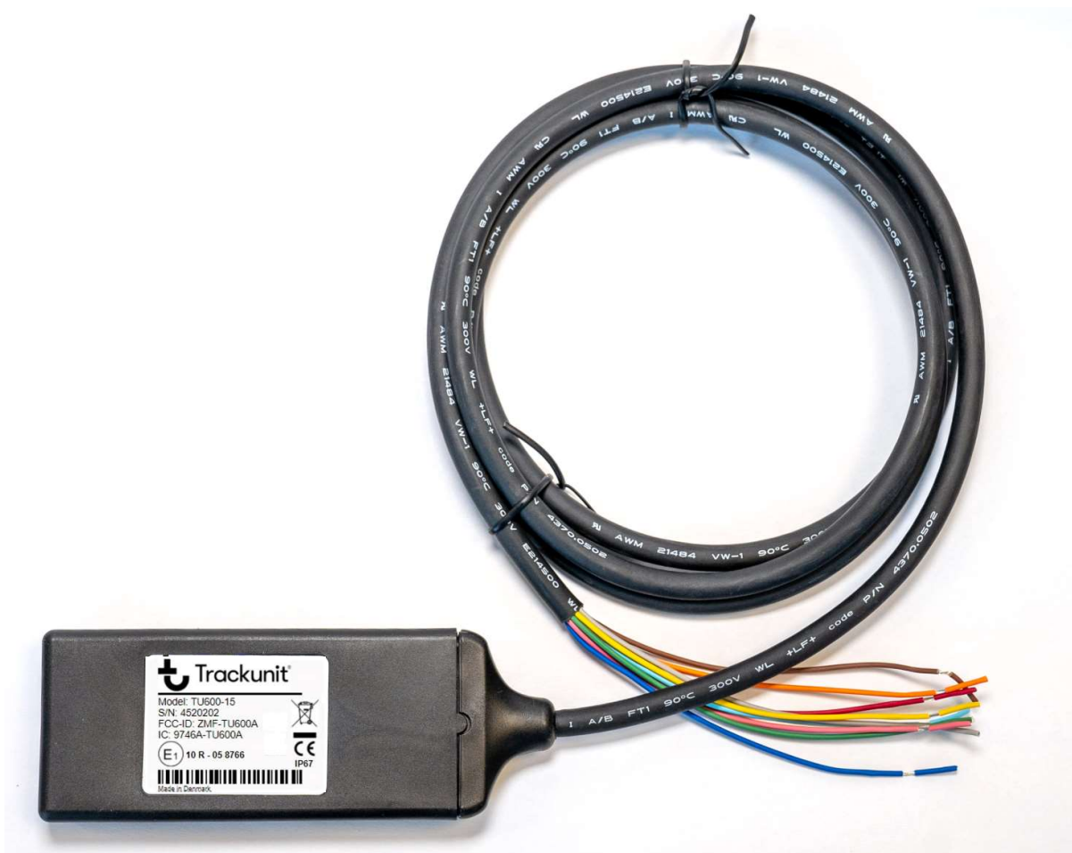
TU600-15 seen from the back with its power/automotive interface cable.
