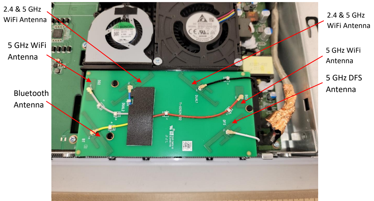
Photograph 3: Antenna Board
