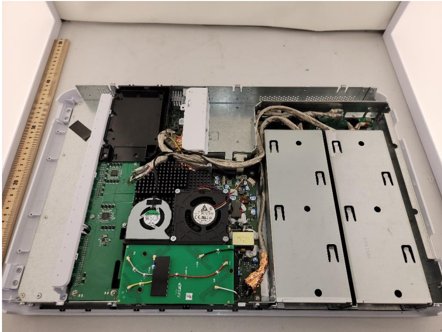
Photograph 2: Side View of the DUT
