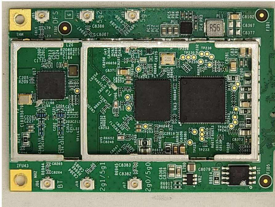
Photograph 4: Front Wireless Printed Circuit Board
