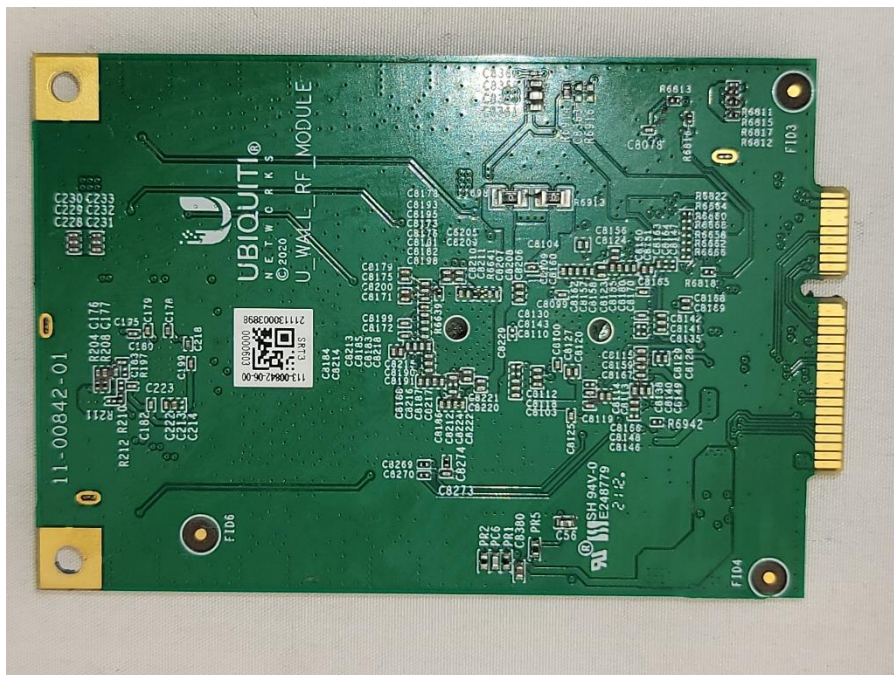
Photograph 5: Back Wireless Printed Circuit Board
