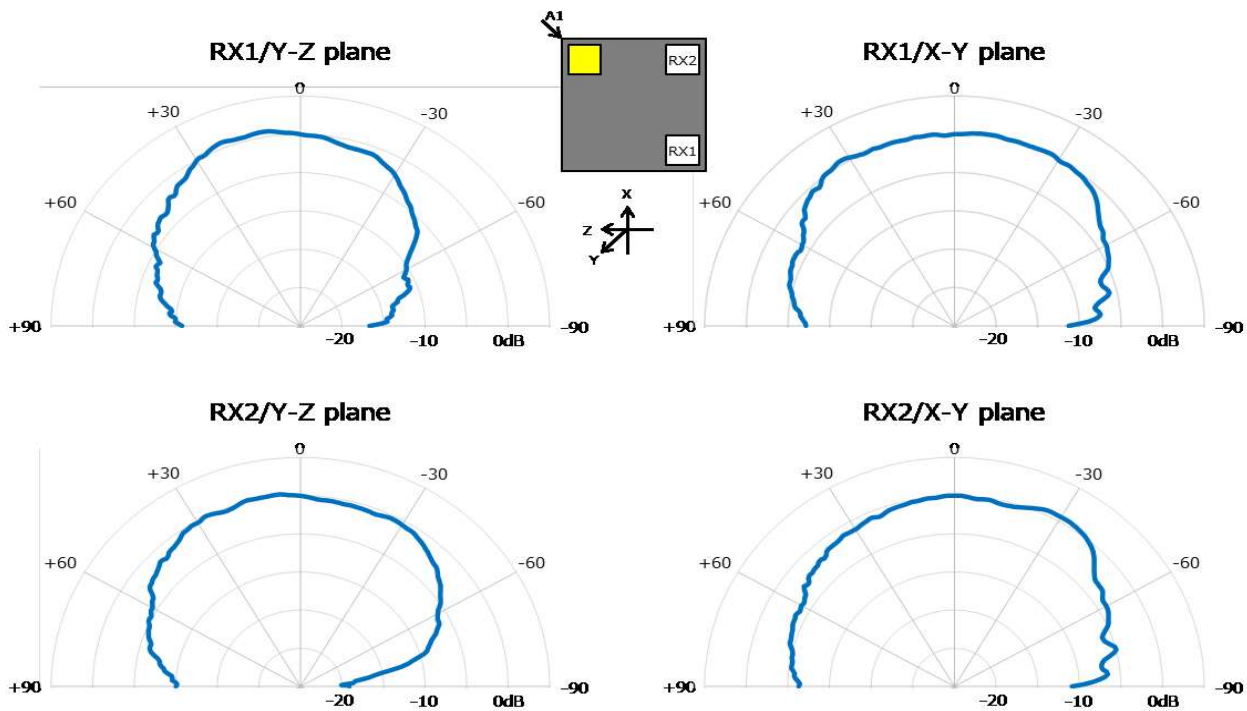
Figure A-2 Measured RX antenna pattern at 24.15GHz
