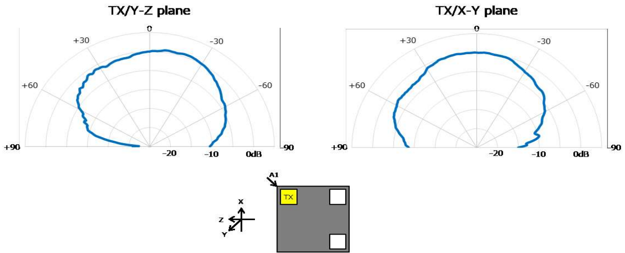
Figure A-1 Measured TX antenna pattern at 24.15GHz
