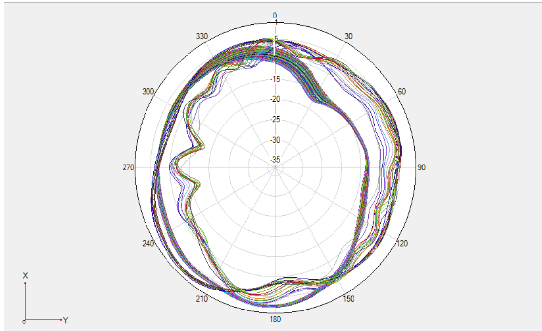
Theta 90 2D
