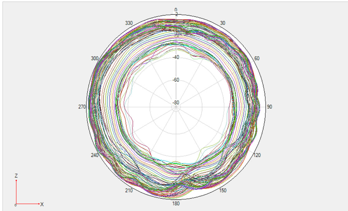
Phi 0 2D
