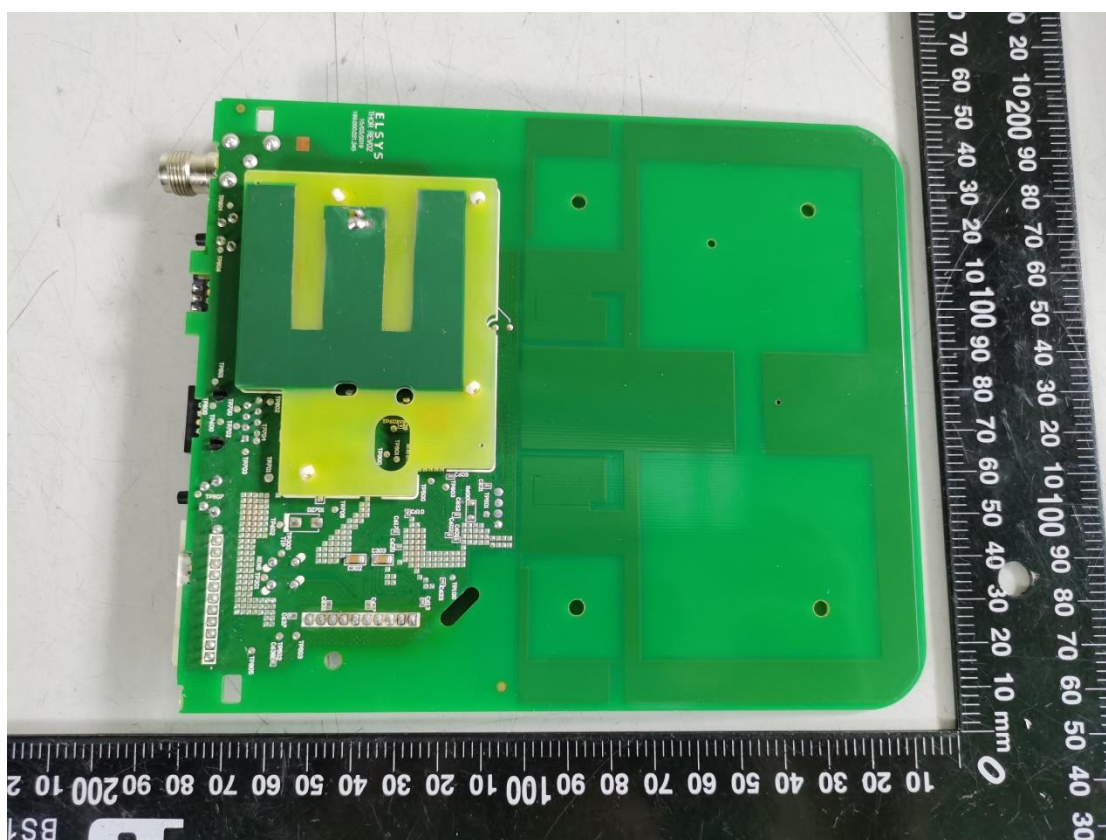
Photo 6 Inside of EUT
