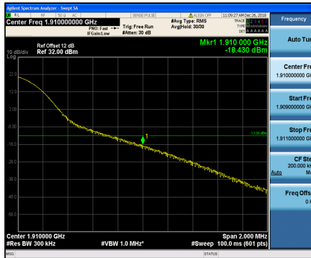
Band2_20MHz_QPSK_19100_1RB#99
