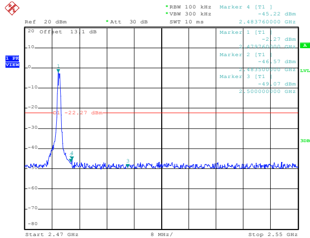
BLE_BT4.0_Ant1_High_2480
