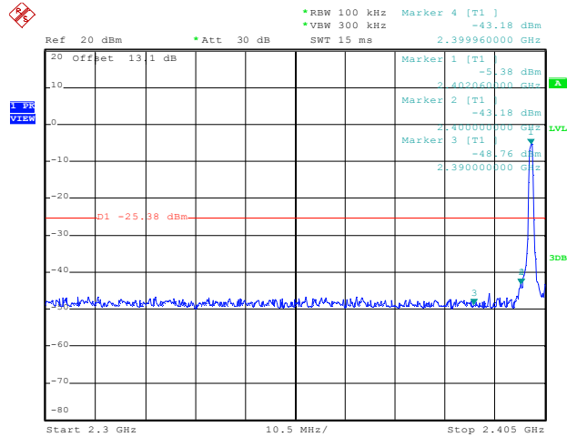
BLE_BT4.0_Ant1_Low_2402
