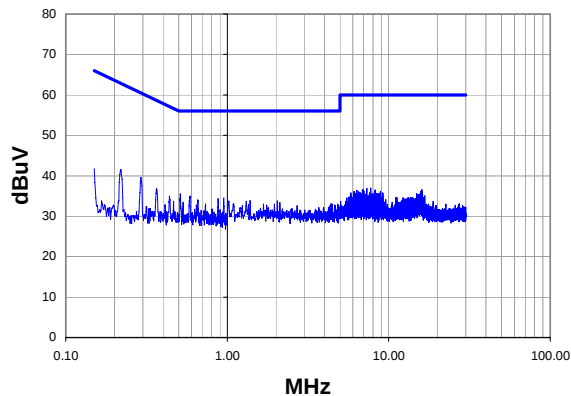
Quasi-Peak
