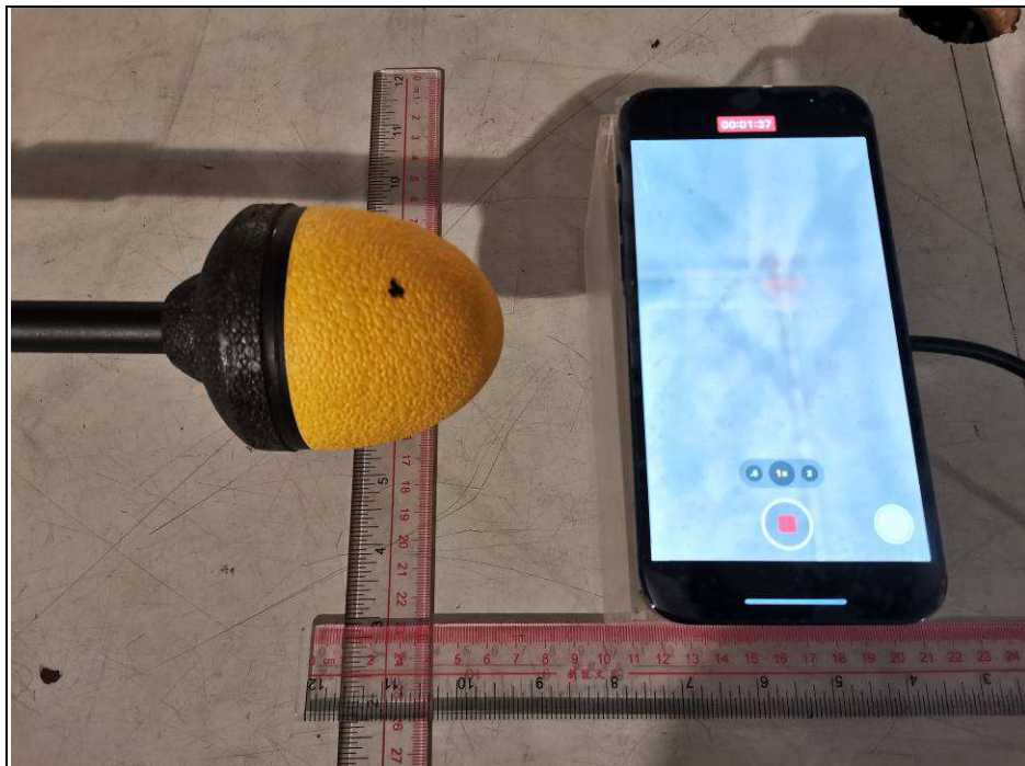
Distance 6 cm
