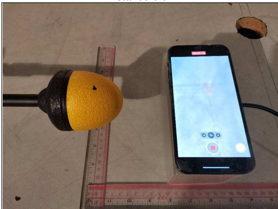
Distance 8 cm
