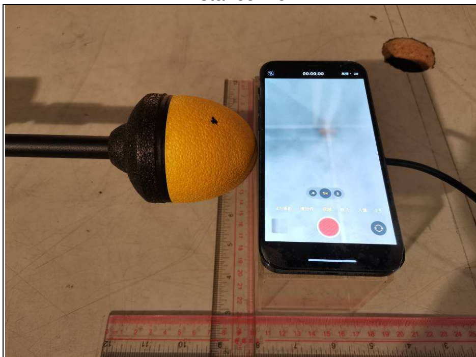
Distance 2 cm
