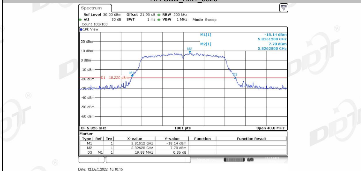
11A-CDD Ant2 5825
