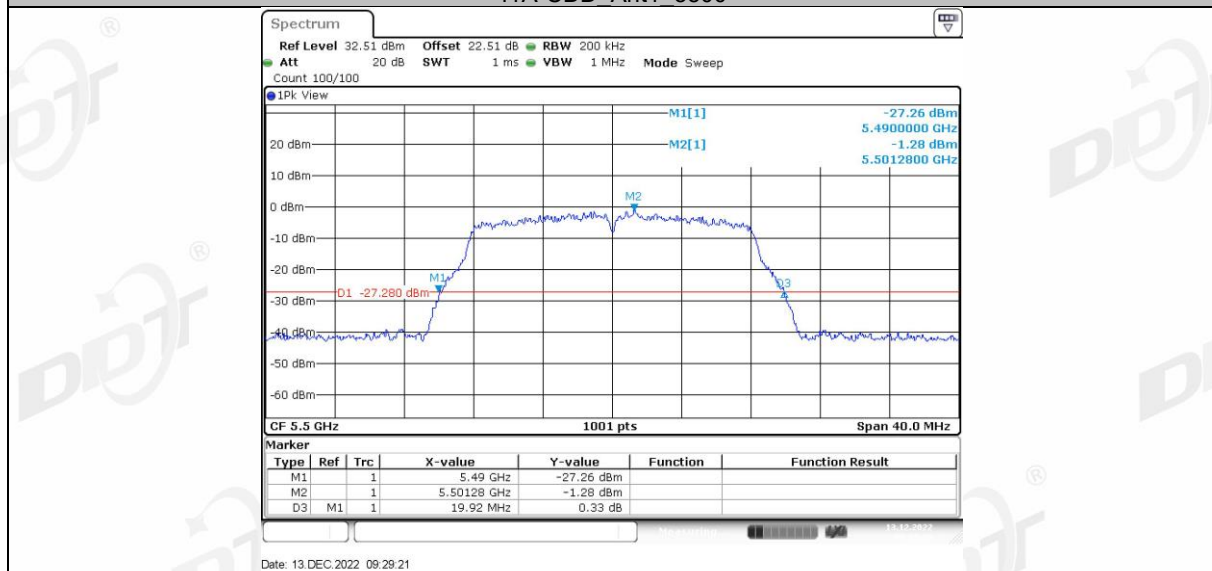
11A-CDD Ant2 5500
