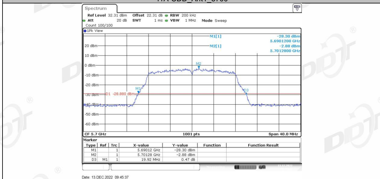
11A-CDD Ant2 5700
