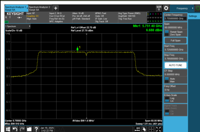
Channel 151 (5755MHz)
