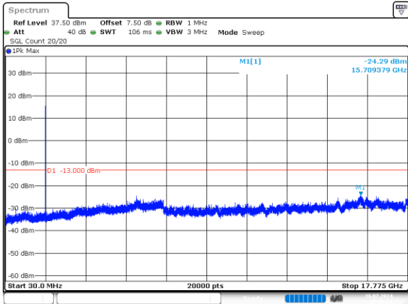
5MHz_High_QPSK_25@0 -24.29dBm
