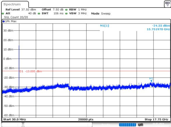
10MHz_High_QPSK_50@0 -24.55dBm
