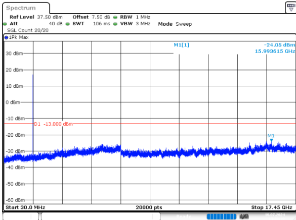
3MHz_Middle_QPSK_15@0 -24.05dBm
