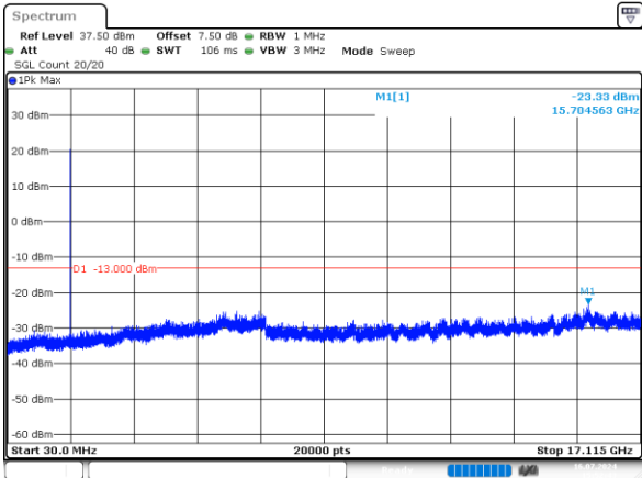
3MHz_Low_QPSK_1@0 -23.33dBm
