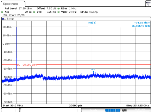
2_15MHz_Low_QPSK_1@0 -34.55dBm
