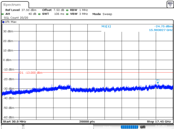
10MHz_Middle_QPSK_1@0 -24.75dBm
