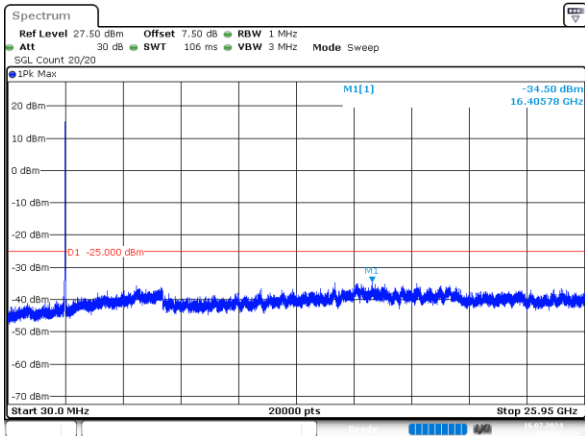
2_20MHz_Middle_QPSK_100@0 -34.50dBm
