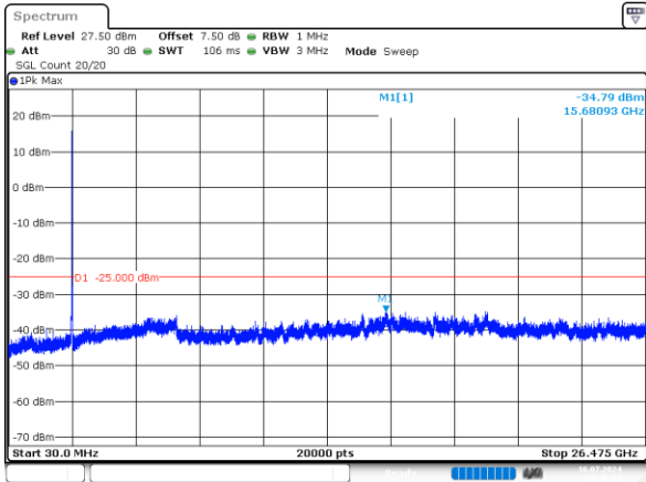
2_15MHz_High_QPSK_75@0 -34.79dBm
