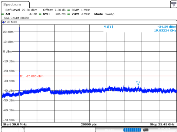
2_20MHz_Low_QPSK_1@0 -34.59dBm
