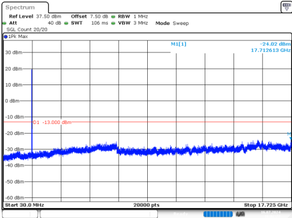
15MHz_High_QPSK_1@0 -24.02dBm
