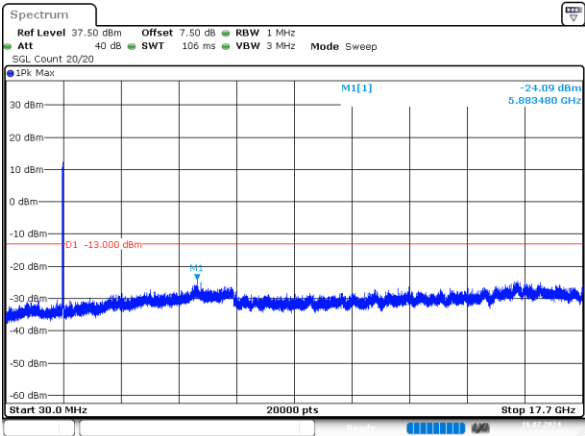
20MHz_High_QPSK_100@0 -24.09dBm
