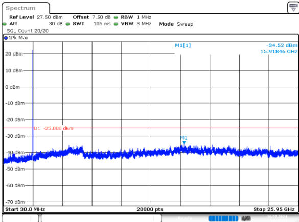
2_15MHz_Middle_QPSK_1@0 -34.52dBm
