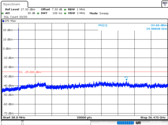
2_15MHz_High_QPSK_1@0 -34.66dBm
