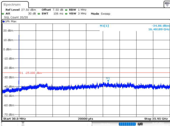
2_15MHz_Middle_QPSK_75@0 -34.86dBm
