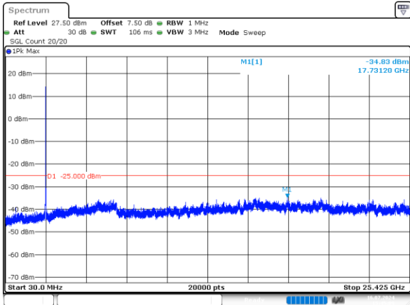
2_15MHz_Low_QPSK_75@0 -34.83dBm
