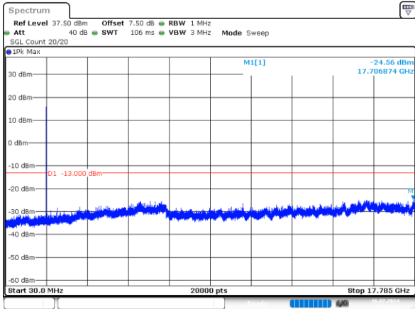
3MHz_High_QPSK_15@0 -24.56dBm
