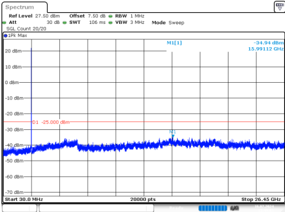
2_20MHz_High_QPSK_1@0 -34.94dBm
