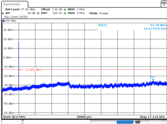
3MHz_Low_QPSK_15@0 -24.70dBm
