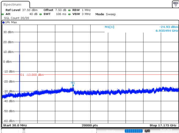
15MHz_Low_QPSK_1@0 -24.93dBm
