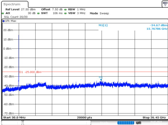
2_20MHz_High_QPSK_100@0 -34.67dBm
