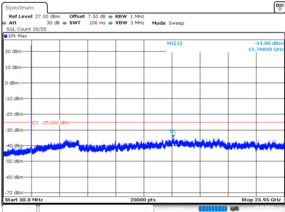
2_20MHz_Middle_QPSK_1@0 -34.80dBm
