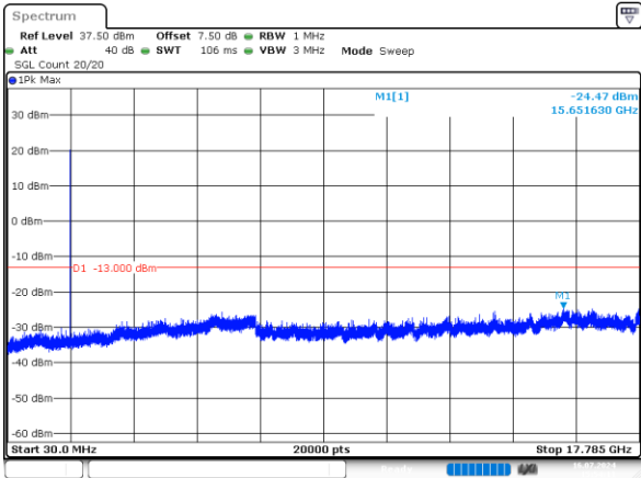
3MHz_High_QPSK_1@0 -24.47dBm
