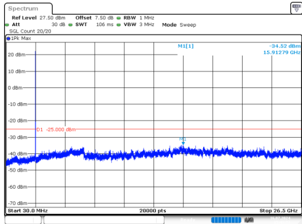
2_10MHz_High_QPSK_1@0 -34.52dBm
