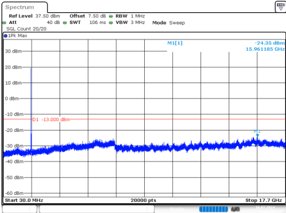
20MHz_High_QPSK_1@0 -24.35dBm
