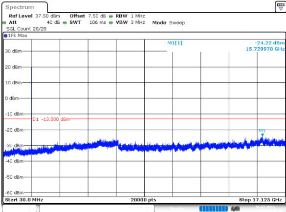
5MHz_Low_QPSK_1@0 -24.22dBm
