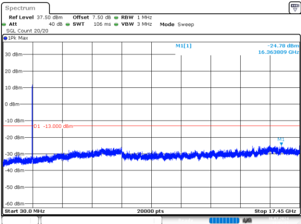
20MHz_Middle_QPSK_100@0 -24.78dBm
