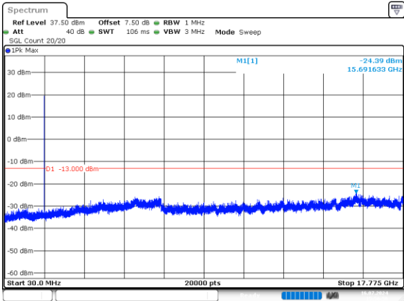
5MHz_High_QPSK_1@0 -24.39dBm
