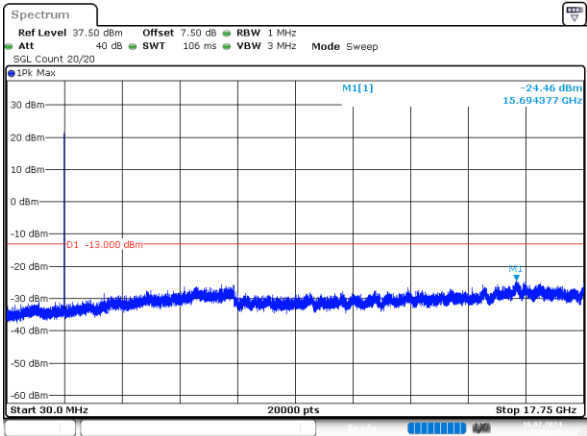
10MHz_High_QPSK_1@0 -24.46dBm
