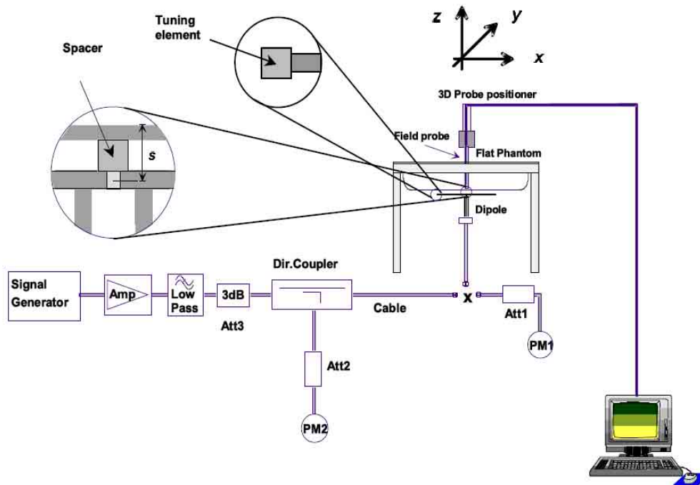
System Check Set-up
