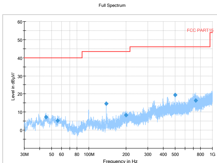
Pic3. Radiated emission (30MHz – 1GHz)
