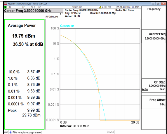
5A_n77(3450-3550MHz) 80M CP-OFDM 256QAM Outer_Full Mid
