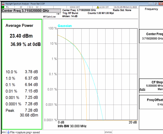
5A_n77(3700-3980MHz) 30M CP-OFDM QPSK Outer_Full Low
