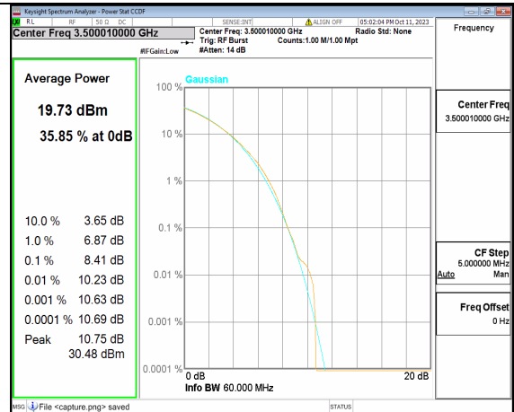
5A_n77(3450-3550MHz) 60M CP-OFDM 256QAM Outer_Full Mid
