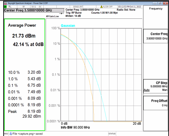
5A_n77(3450-3550MHz) 90M DFT-s-OFDM 256QAM Outer_Full Mid
