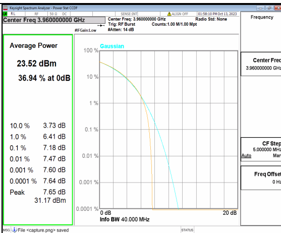
5A_n77(3700-3980MHz) 40M CP-OFDM QPSK Outer_Full High
