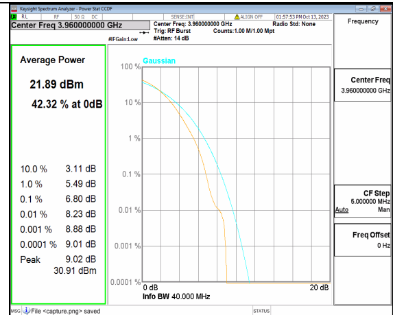
5A_n77(3700-3980MHz) 40M DFT-s-OFDM 256QAM Outer_Full High
