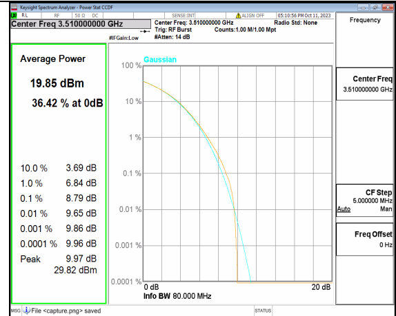
5A_n77(3450-3550MHz) 80M CP-OFDM 256QAM Outer_Full High
