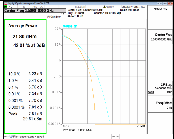
5A_n77(3450-3550MHz) 60M DFT-s-OFDM 256QAM Outer_Full Mid
