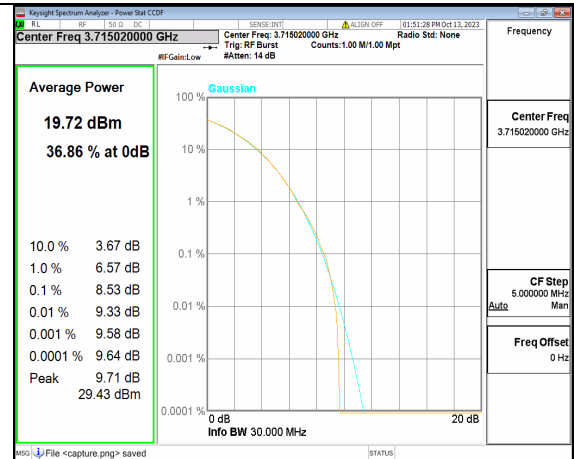
5A_n77(3700-3980MHz) 30M CP-OFDM 256QAM Outer_Full Low
