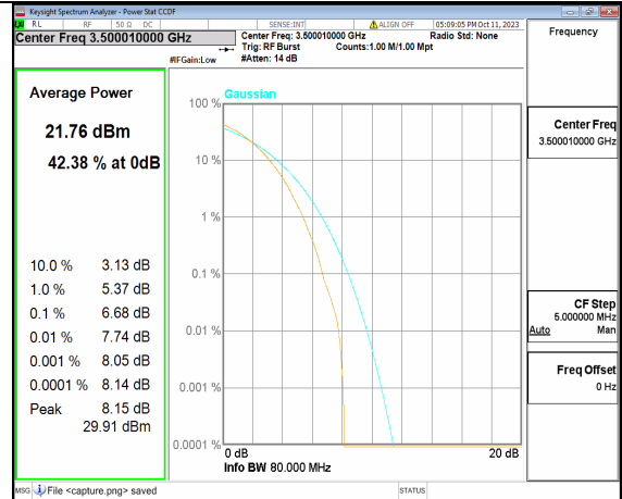
5A_n77(3450-3550MHz) 80M DFT-s-OFDM 256QAM Outer_Full Mid
