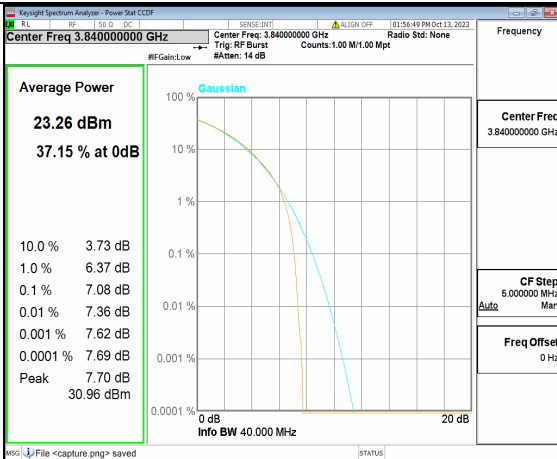
5A_n77(3700-3980MHz) 40M CP-OFDM QPSK Outer_Full Mid
