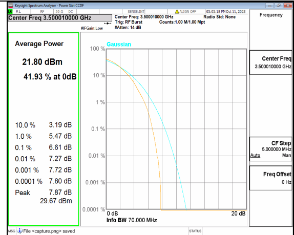
5A_n77(3450-3550MHz) 70M DFT-s-OFDM 256QAM Outer_Full Mid
