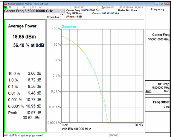
5A_n77(3450-3550MHz) 90M CP-OFDM 256QAM Outer_Full Mid
