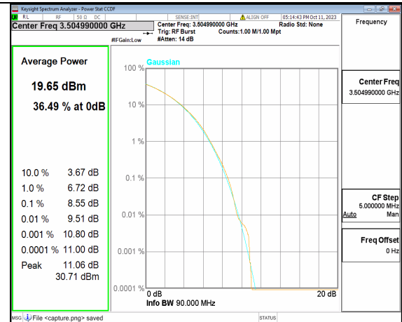
5A_n77(3450-3550MHz) 90M CP-OFDM 256QAM Outer_Full High
