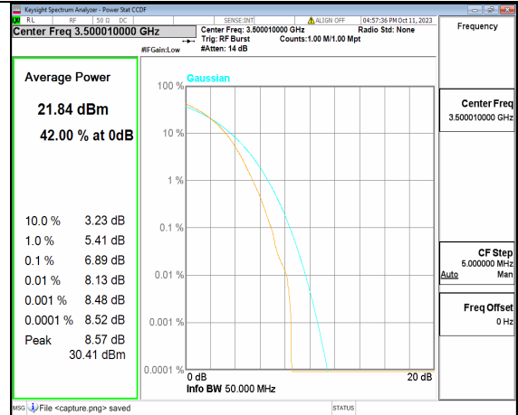
5A_n77(3450-3550MHz) 50M DFT-s-OFDM 256QAM Outer_Full Mid
