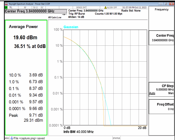
5A_n77(3700-3980MHz) 40M CP-OFDM 256QAM Outer_Full Mid
