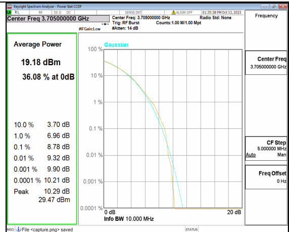
5A_n77(3700-3980MHz) 10M CP-OFDM 256QAM Outer_Full Low
