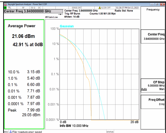
5A_n77(3700-3980MHz) 10M DFT-s-OFDM 256QAM Outer_Full Mid
