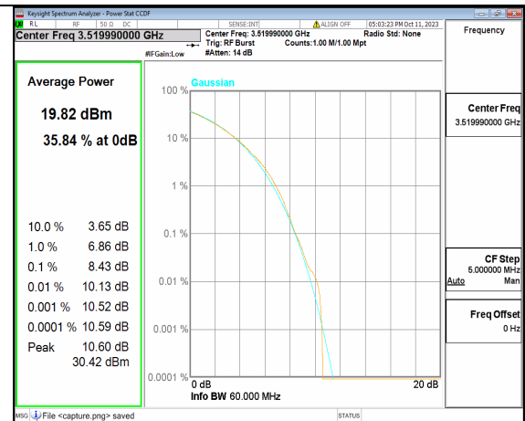
5A_n77(3450-3550MHz) 60M CP-OFDM 256QAM Outer_Full High
