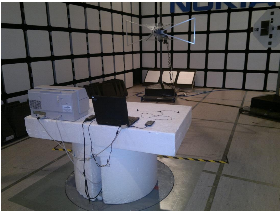
Picture 2. FCC Part 15B Radiated emissions
