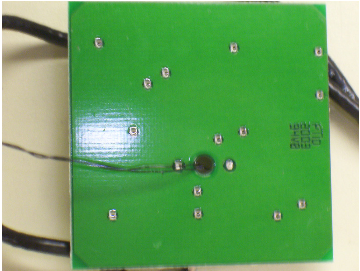
Source Tagging Tester (STT) – Antenna PCB – (solder side)
