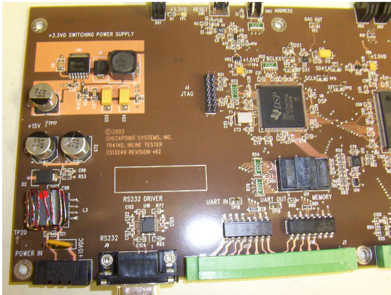
Source Tagging Tester (STT) – TR4140 PCB – (component side, left half)
