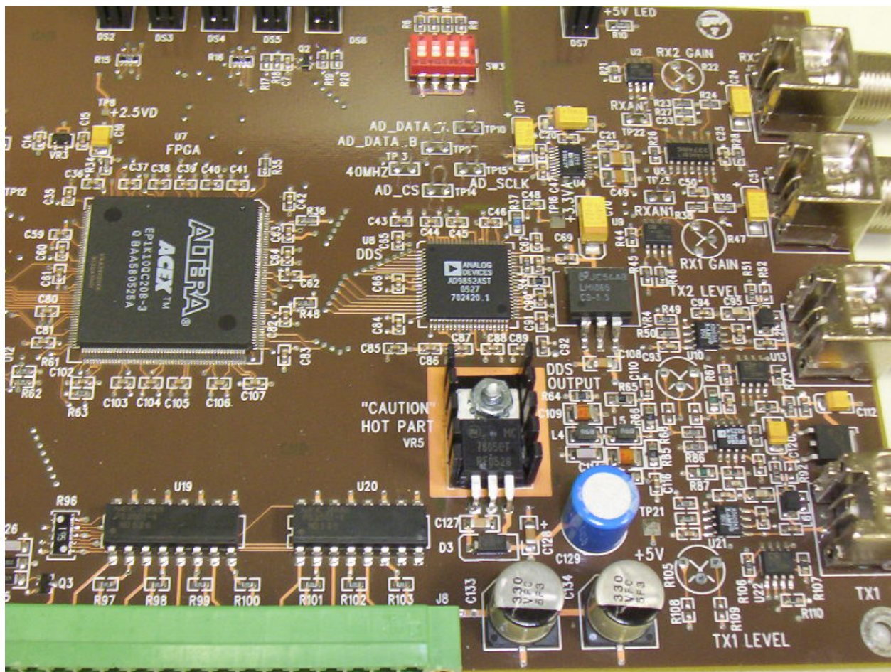
Source Tagging Tester (STT) – TR4140 PCB – (component side, right half)
