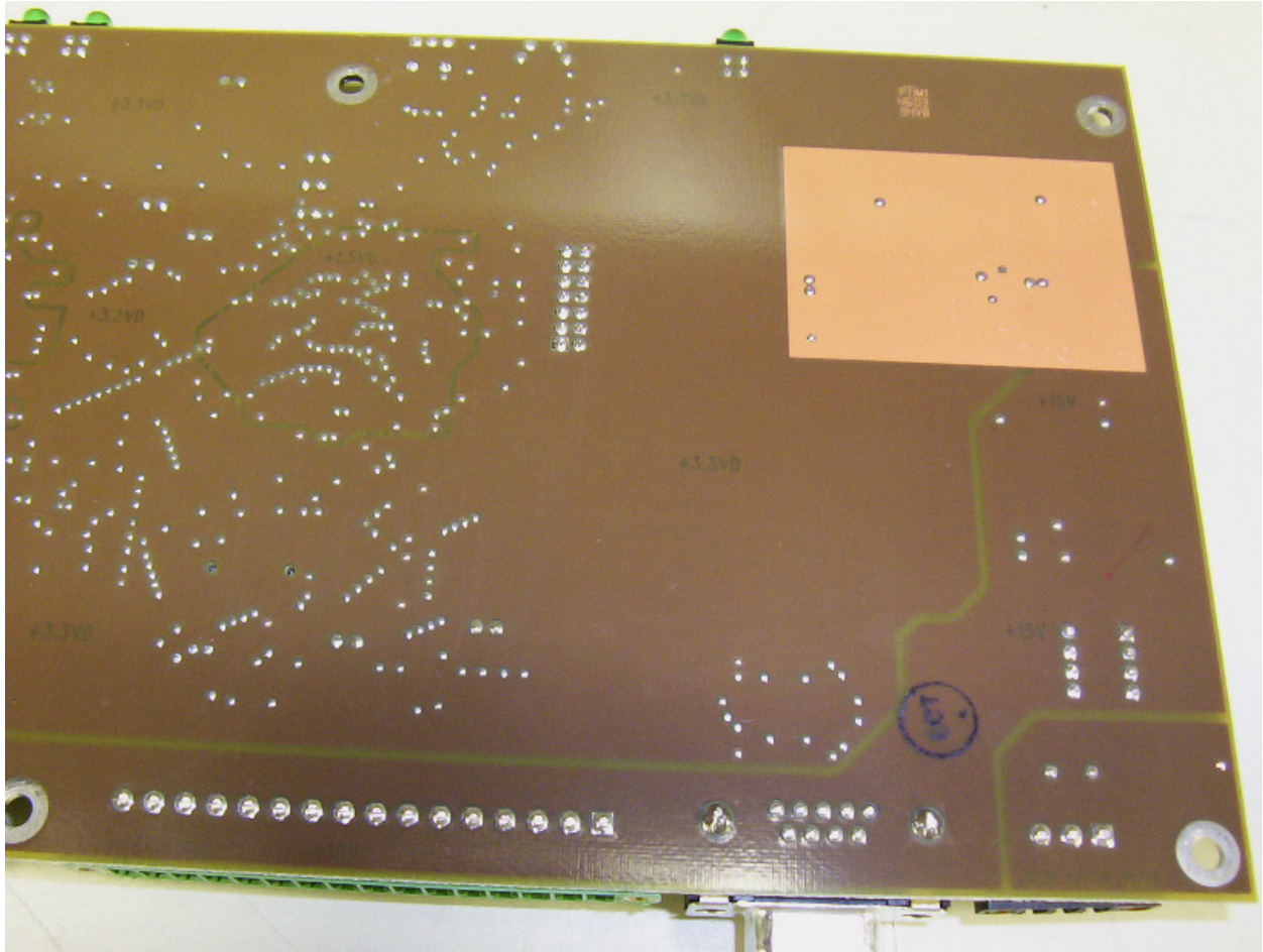
Source Tagging Tester (STT) – TR4140 PCB – (solder side, left half)
