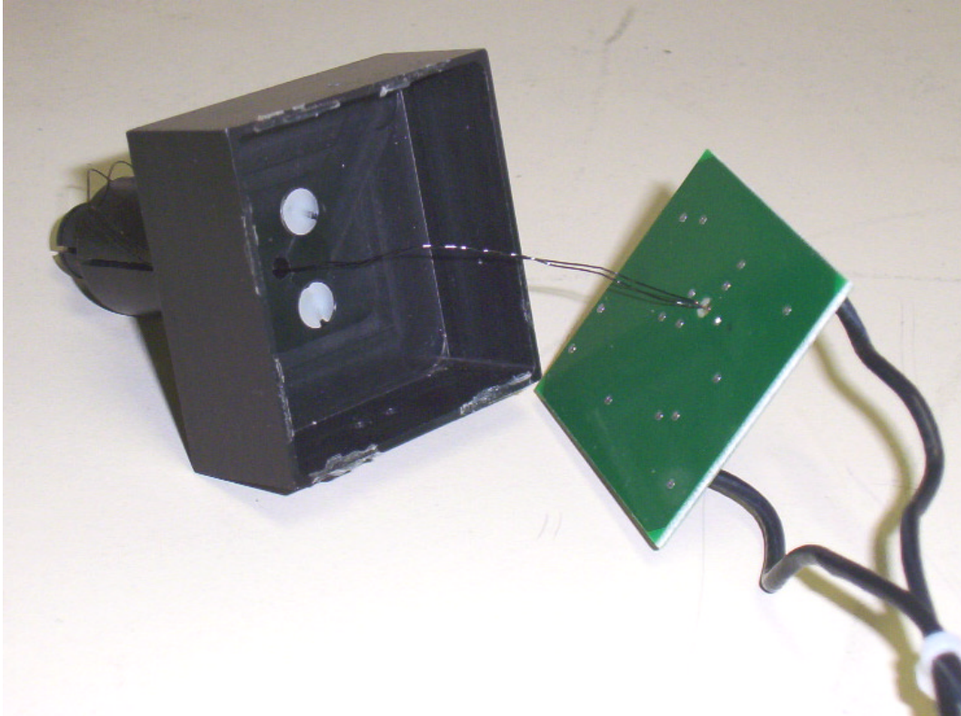
Source Tagging Tester (STT) – Antenna – (bottom cover removed)
