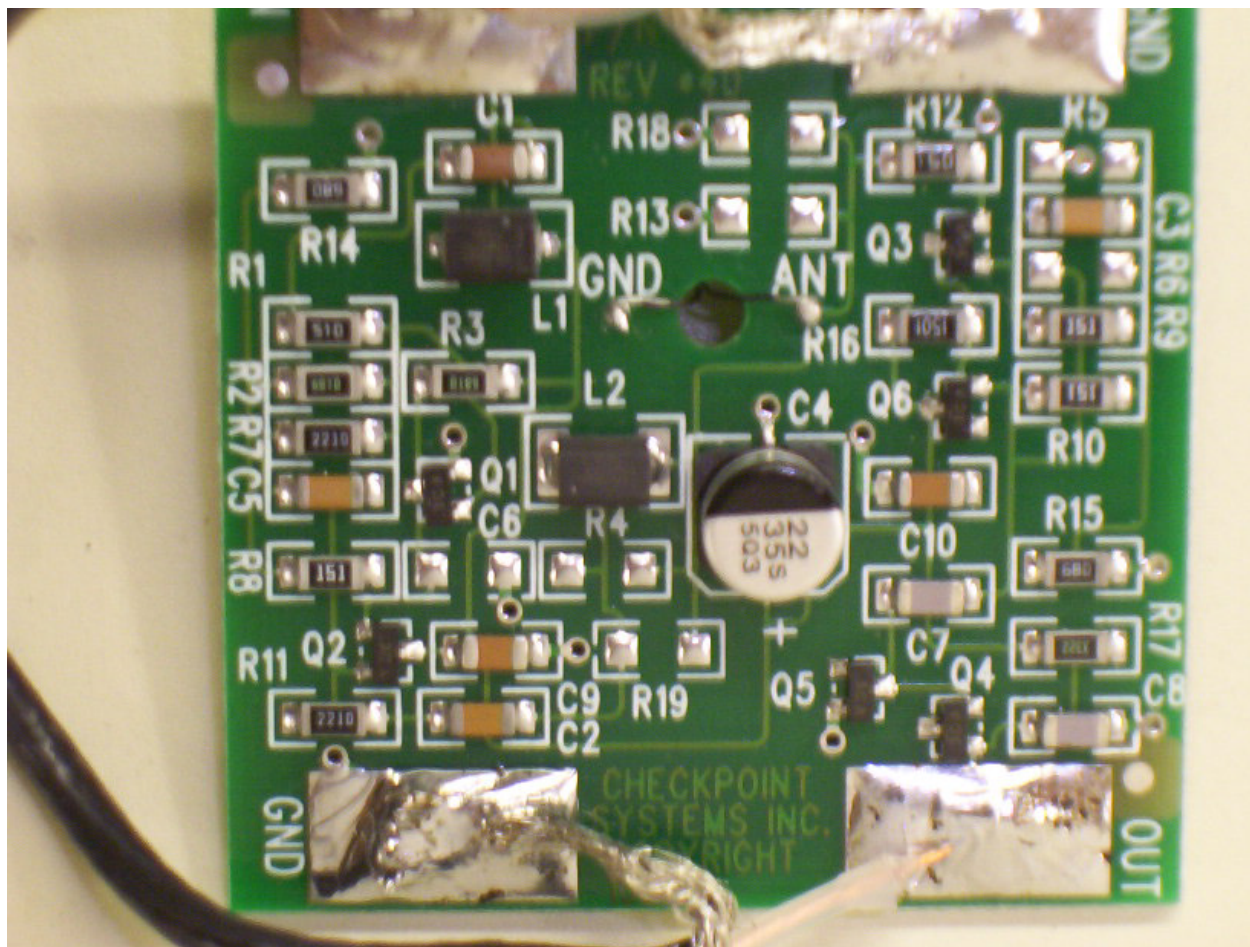
Source Tagging Tester (STT) – Antenna PCB – (component side)
