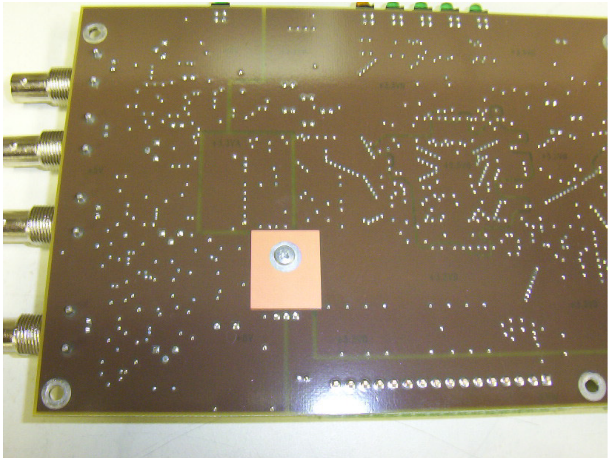
Source Tagging Tester (STT) – TR4140 PCB – (solder side, right half)
