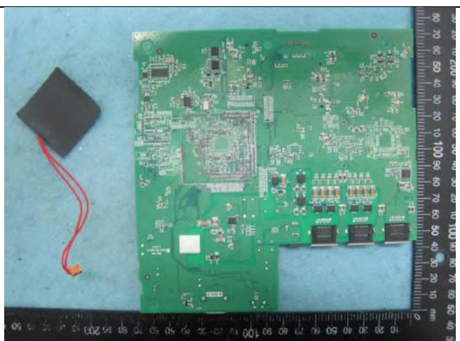
PCB 1 – Cover off view
