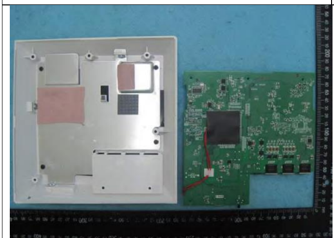
PCB 1 – Top view
