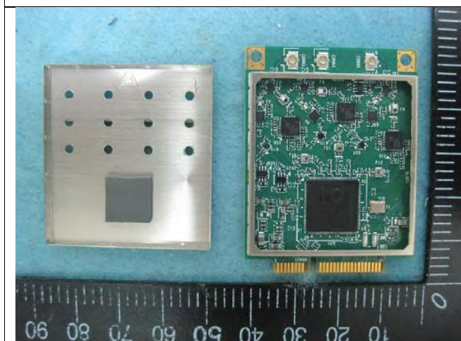
PCB 4 – Top view
