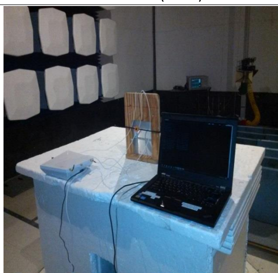
Radiated Emissions (>1GHz) – Rear View
